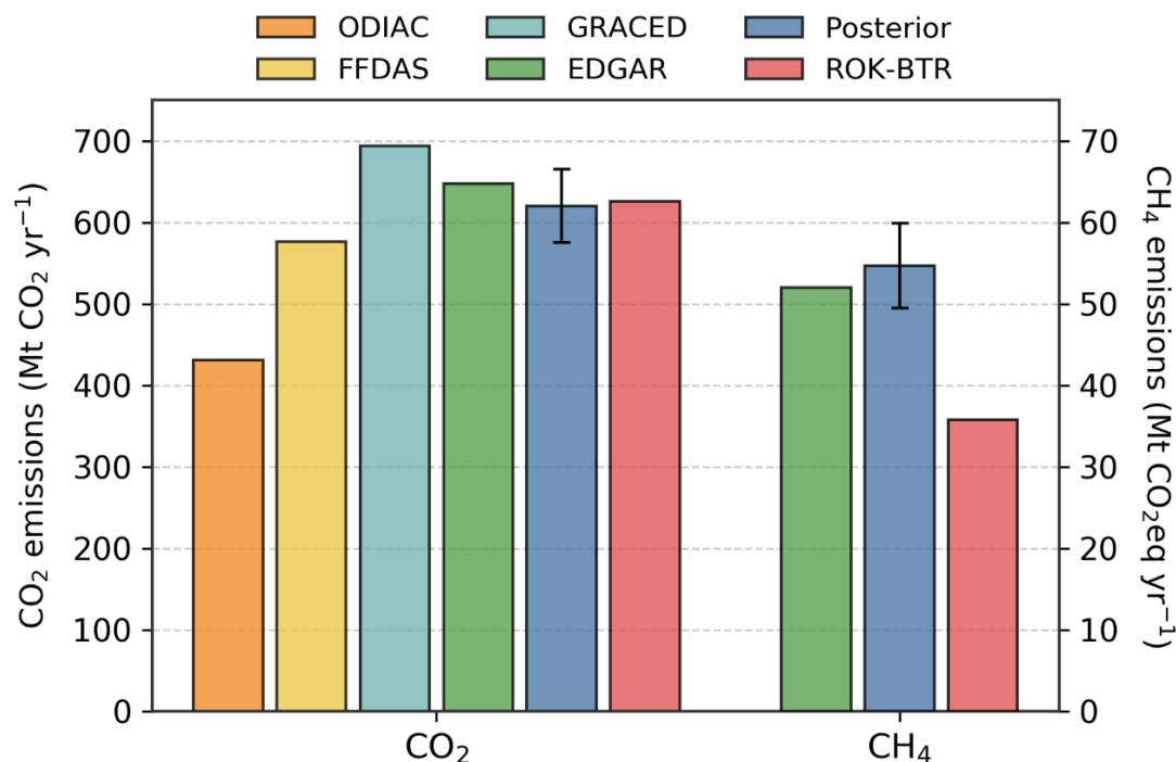
615 Figure 10. Annual total anthropogenic CO 2 and CH 4 emissions over South Korea in 2020 from multiple datasets. CO 2 comparisons include ODIAC, FFDAS, GRACED, EDGAR, ROK-BTR, and the posterior (six sources). CH 4 comparisons include EDGAR, ROK-BTR, and the posterior. Error bars denote posterior uncertainty. (FFDAS was scaled using the 2015–2020 gross emission growth rate from ROK-BTR because FFDAS is available only through 2015)
