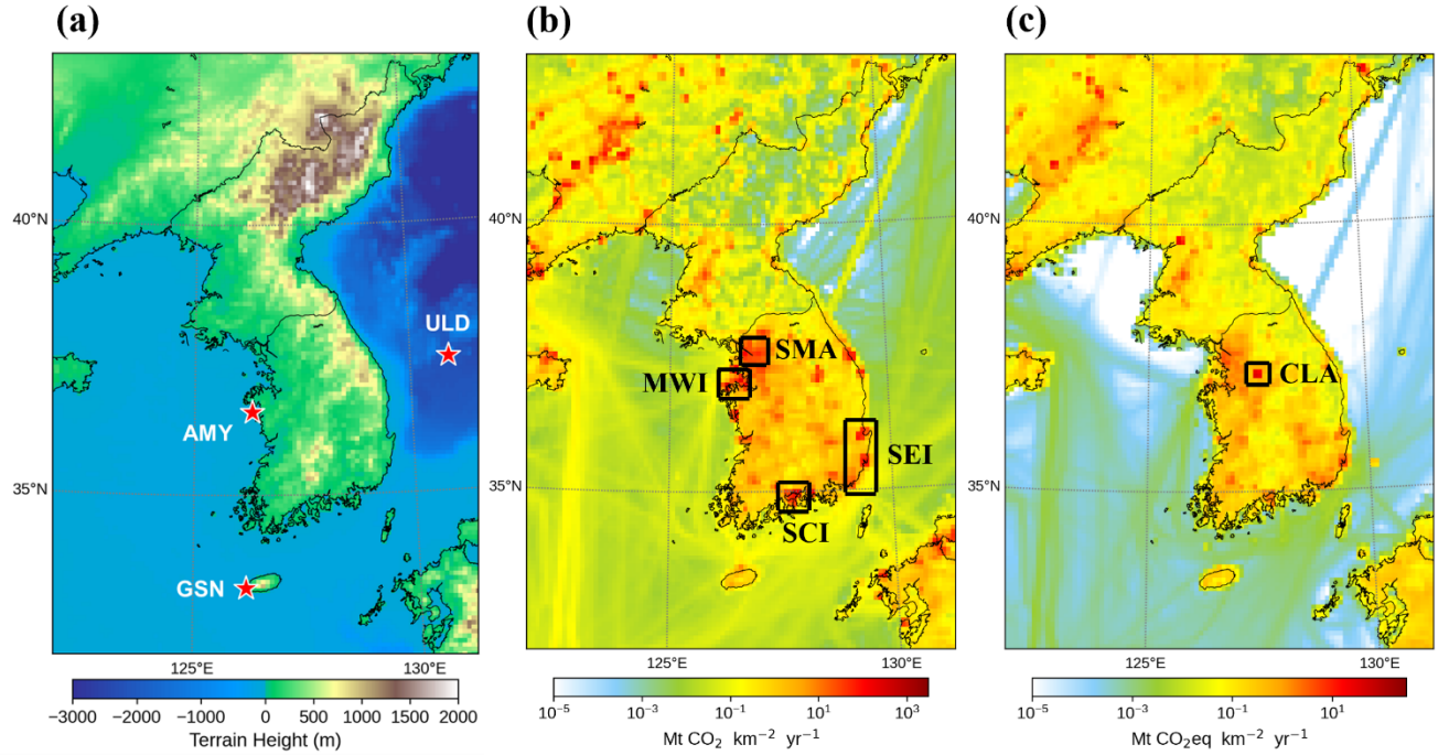
Figure 2. Locations of GHG monitoring stations (AMY, GSN, ULD) over terrain height (a) and annual anthropogenic emissions of CO 2 (b) and CH 4 (c) in the model domain in 2020 from the Emissions Database for Global Atmospheric Research (EDGAR v8.0). Main emission source regions in the model domain are boxed: SMA (Seoul Metropolitan Area), MWI (Mid-Western Industrial Area), SEI (Southeastern Industrial Area), SCI (South Coast Industrial Area), and CLA (Central Livestock Area).
