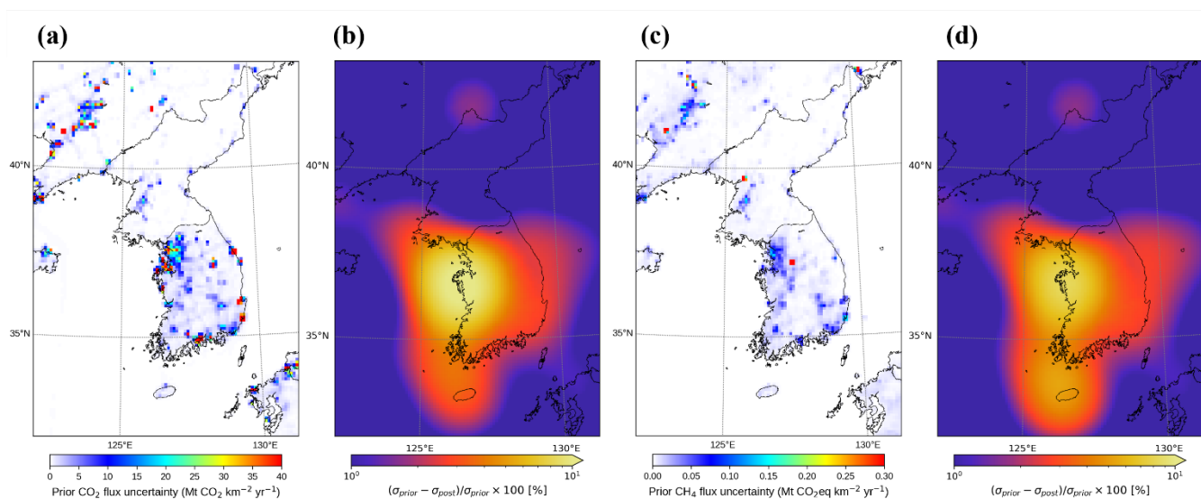
Figure 7. Annual prior flux uncertainty (a and c) and flux-uncertainty reduction (b and d) for CO 2 (a and b) and CH 4 (c and d) in 2020. Note that ocean-grid uncertainties are non-zero but appear small on the plotted scale because the prior spread is prescribed as a fractional perturbation and absolute oceanic flux magnitudes are much smaller than terrestrial sources.
