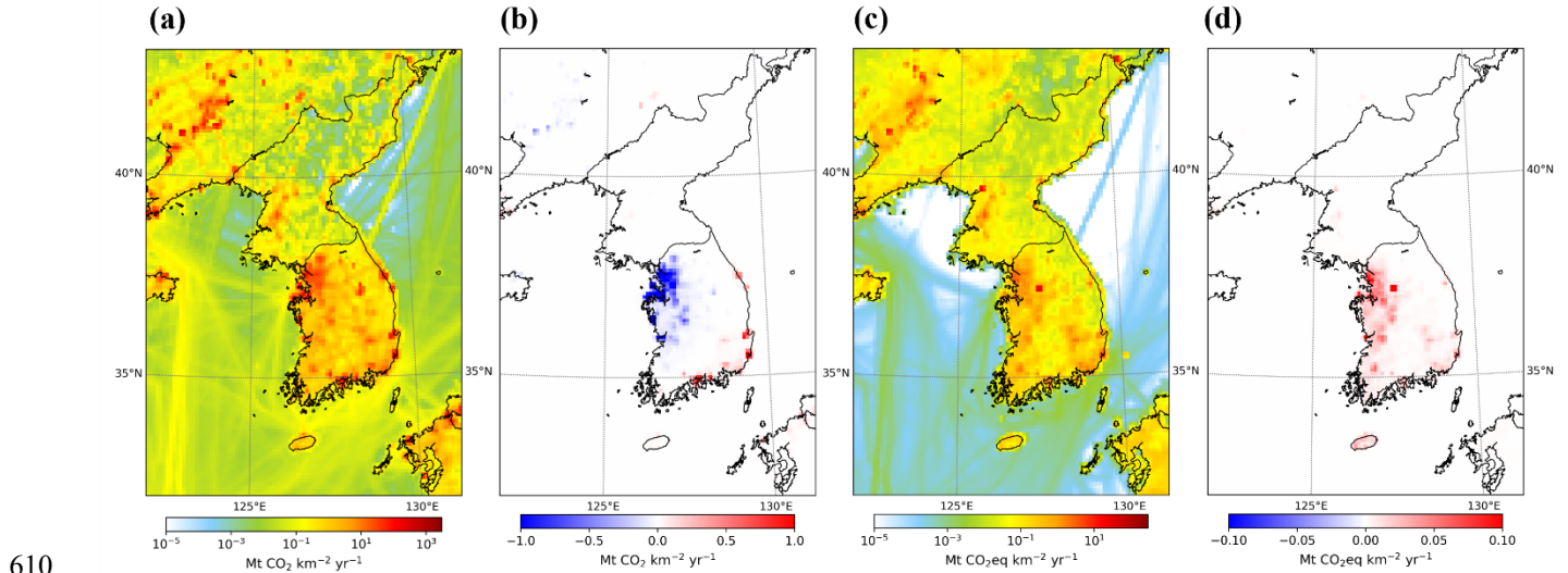
Figure 9. Annual-mean posterior surface fluxes (a and c) and assimilation increments (posterior minus prior) (b and d) for CO 2 (a and b) and CH 4 (c and d) from the WRF-Chem/DART system. Red (blue) shading indicates an increase (decrease) in the posterior relative to the prior.
