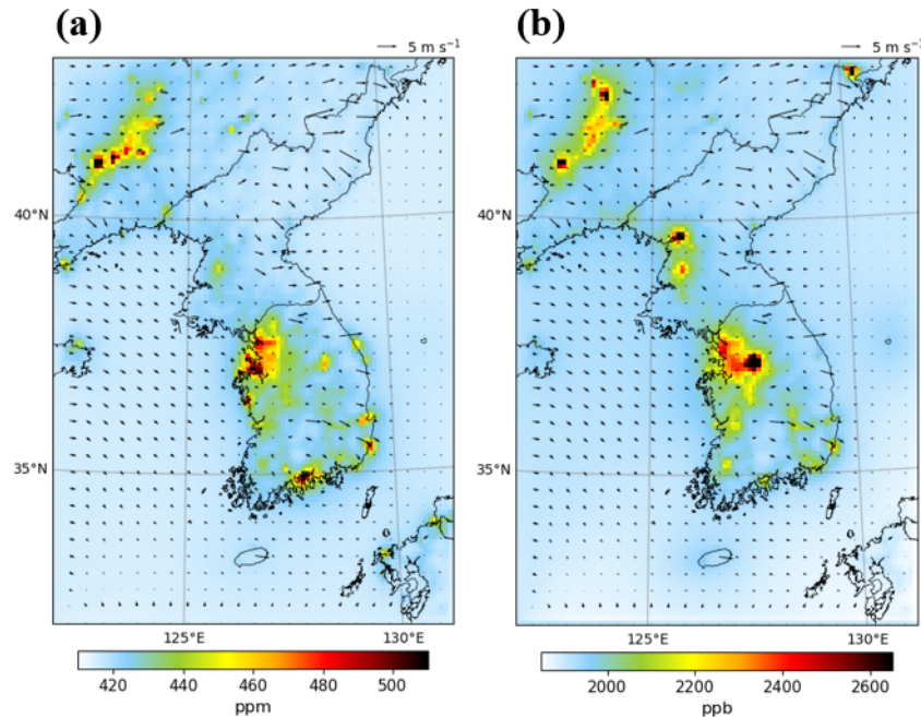
Figure 8. Annual mean surface posterior concentrations of CO 2 (a) and CH 4 (b) over the Korean Peninsula in 2020 from the WRF-Chem/DART inversion system. Wind vectors at 10 m illustrate prevailing flow conditions that shape annual concentration gradients.
