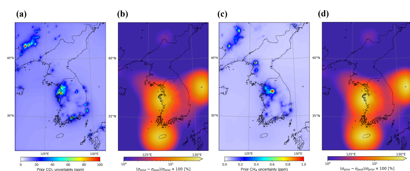
Figure 6. Annual prior concentration uncertainty (ensemble spread) (a,c) and its reduction after assimilation (b,d) for CO 2 (a,b) and CH 4 (c,d) in 2020.
