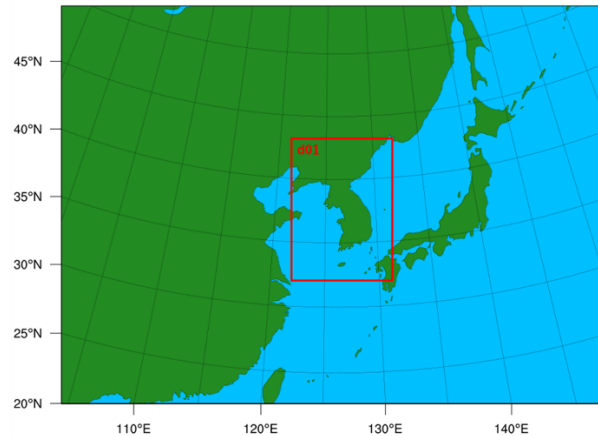
Figure 1. The WRF-Chem model domain used in this study. The red rectangle, marked d01, is the single computational domain of the WRF-Chem simulation (9 km horizontal spacing, 97 \times 136 grid points), covering the Korean Peninsula and its surrounding seas. The remainder 150 of the map shows the wider East Asian region for geographic context and is not part of the simulated area.
