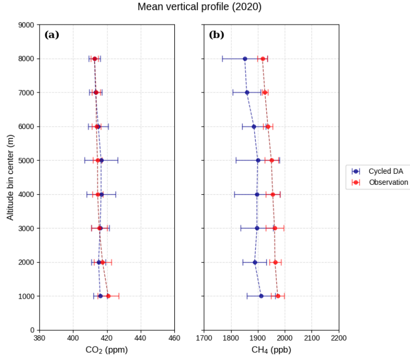
475 Figure 5. Mean vertical profiles of CO 2 and CH 4 from 10 CM-01 flights over South Korea in 2020. Profiles are aggregated into 1 km altitude bins ( \pm 500 m). Symbols and error bars show mean concentrations and associated uncertainties per bin: observations (red) and cycled DA (blue). Observation uncertainties combine measurement precision and sampling variability.
