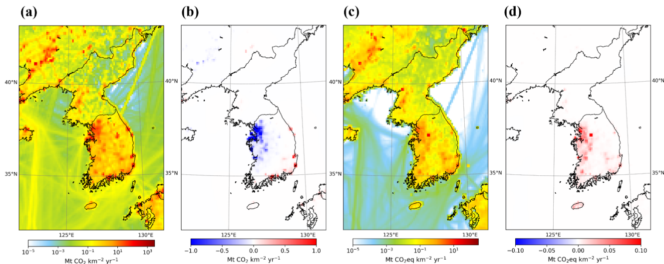
Figure 9. Annual-mean posterior surface fluxes (a and c) and assimilation increments (posterior minus prior) (b and d) for CO 2 (a and b) and CH 4 (c and d) from the WRF-Chem/DART system. Red (blue) shading indicates an increase (decrease) in the posterior relative to the prior.
