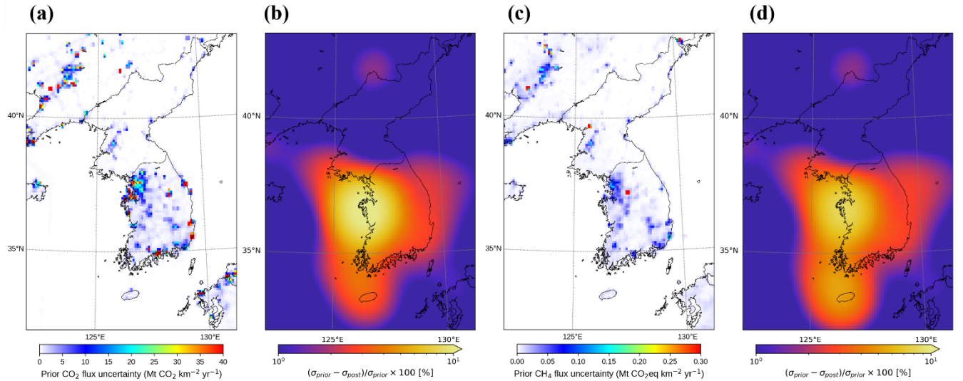
Figure 7. Annual prior flux uncertainty (a and c) and flux-uncertainty reduction (b and d) for CO 2 (a and b) and CH 4 (c and d) in 2020. Note that ocean-grid uncertainties are non-zero but appear small on the plotted scale because the prior spread is prescribed as a fractional perturbation and absolute oceanic flux magnitudes are much smaller than terrestrial sources.
