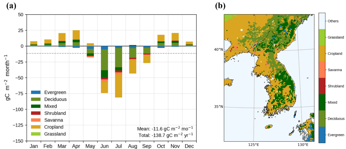
405 Figure 3. (a) Monthly net ecosystem exchange (NEE) contributions by vegetation class over the model domain in 2020. Bars show class totals ( \text{gC m}^{-2} \text{ month}^{-1} ), computed as spatial averages over grid cells of the corresponding vegetation type; negative values indicate net carbon uptake. (b) Spatial distribution of dominant vegetation classes used in WRF-Chem/VPRM; each grid cell is assigned the class with the largest vegetation fraction. Colors are consistent across panels.
