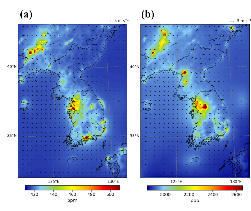
Figure 9. Annual mean surface posterior concentrations of CO 2 (a) and CH 4 (b) over the Korean Peninsula in 2020 from the WRF-Chem/DART inversion system. Wind vectors at 10m illustrate prevailing flow conditions that shape annual concentration gradients.
