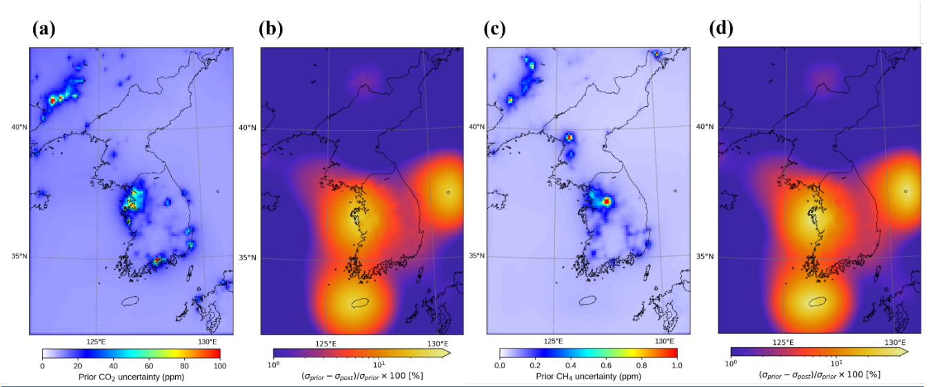
Figure 7. Annual prior concentration uncertainty (ensemble spread) (a,c) and its reduction after assimilation (b,d) for CO 2 (a,b) and CH 4 (c,d) in 2020.
