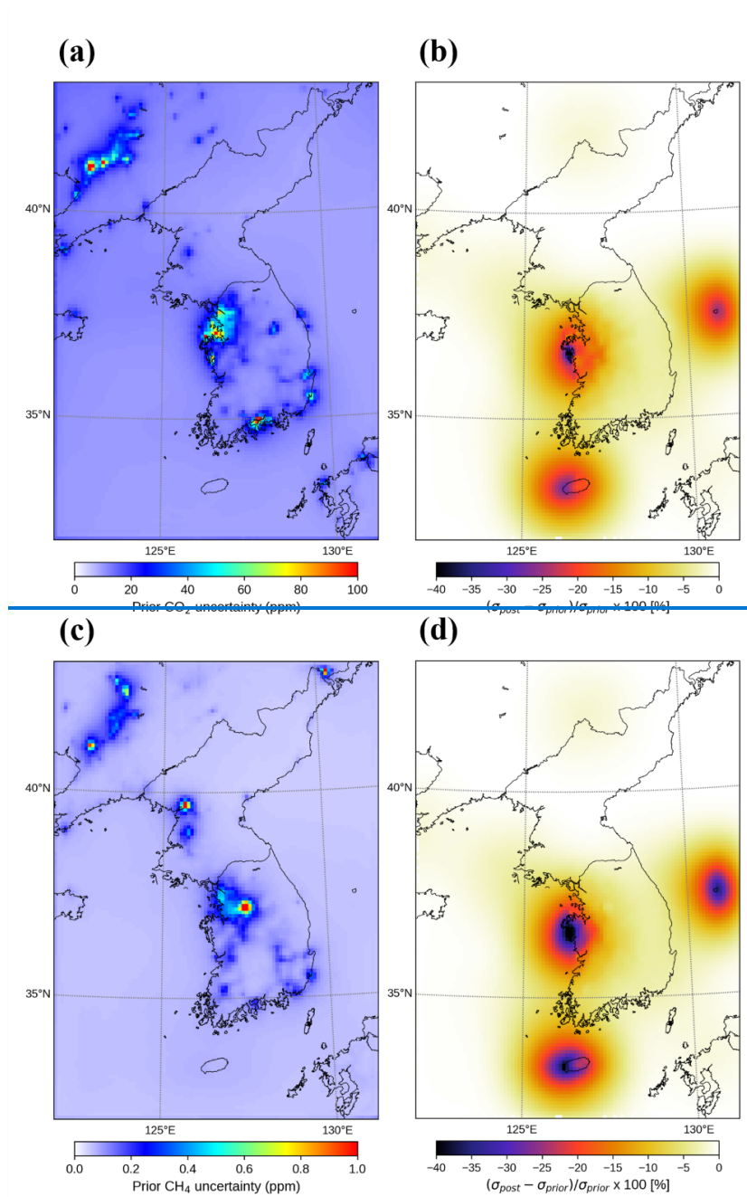
Figure 6. Annual prior concentration uncertainty (ensemble spread) (a,c) and its reduction after assimilation (b,d) for CO 2 (a,b) and CH 4 (c,d) in 2020.
