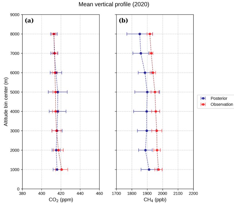
Figure 56. Mean vertical profiles of CO 2 and CH 4 from 10 CM-01 flights over South Korea in 2020. Profiles are aggregated into 1 km altitude bins ( \pm 500 m). Symbols and error bars show mean concentrations and associated uncertainties per bin: observations (red) and posterior (blue). Observation uncertainties combine measurement precision and sampling variability.
