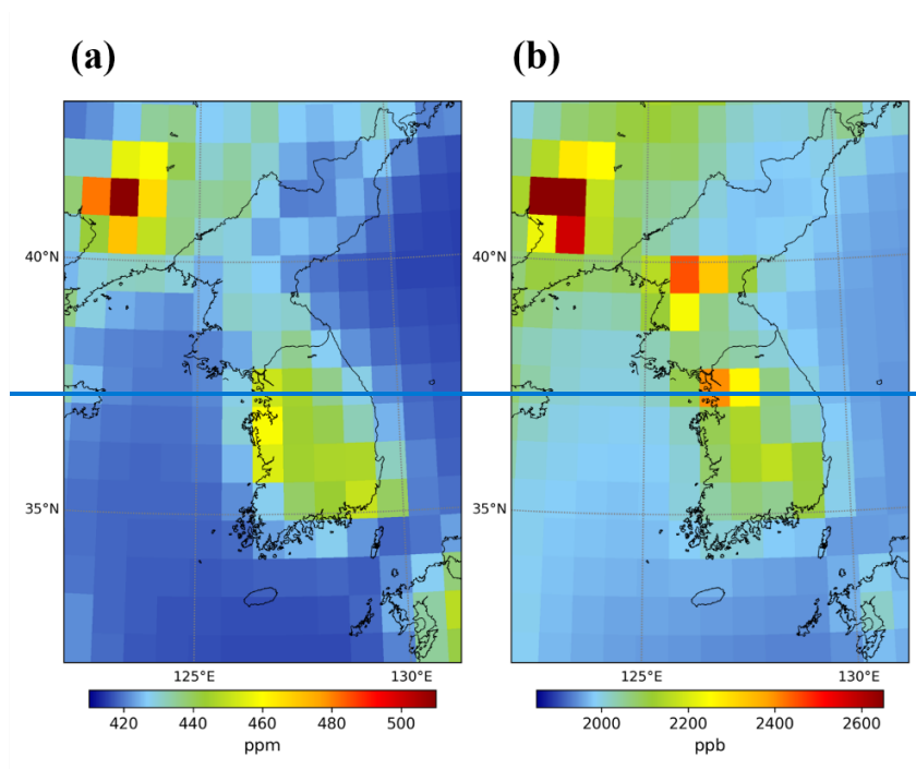
Figure 8. Annual mean surface concentrations of \text{CO}_2 (a) and \text{CH}_4 (b) over the Korean Peninsula in 2020 from the EGG4.
