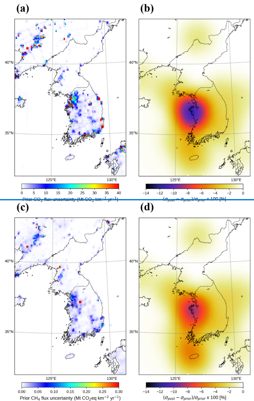
755 Figure 7. Annual prior flux uncertainty (a and c) and flux uncertainty reduction (b and d) for CO 2 (a and b) and CH 4 (c and d) in 2020.
