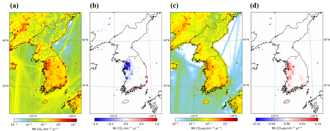
Figure 10. Annual-mean posterior surface fluxes (a and c) and assimilation increments (posterior minus prior) (b and d) for CO 2 (a and b) and CH 4 (c and d) from the WRF-Chem/DART system. Red (blue) shading indicates an increase (decrease) in the posterior relative to the prior.
