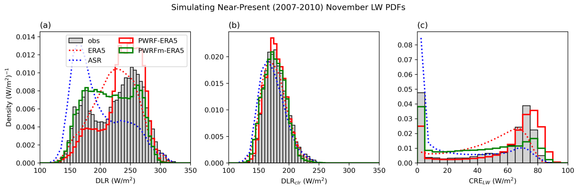
Figure 6. 2007-2010 PDFs of DLR, DLR_{clr} and CRE_{LW} for d02 of the model study. PDFs are generated using CloudSat and CALIPSO 2B-FLXHR-LIDAR (gray bar), ERA5 hourly data (red dotted), ASR 3-hourly data (blue dotted), PWRF-ERA5 hourly data using the P3 scheme (red solid), and PWRF-ERA5 hourly data using the Morrison 2-moment scheme (green solid).
