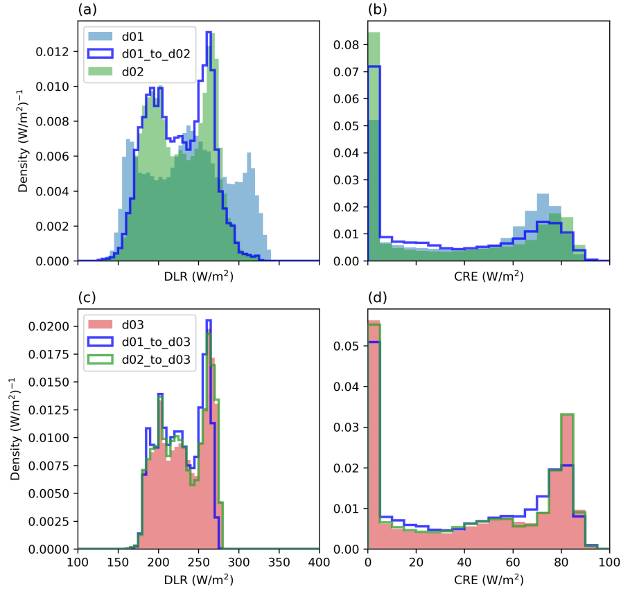
Figure 7. Comparisons between DLR and CRE_{LW} PDFs from PWRP-ERA5 using different horizontal grid resolutions for November 26 - December 1, 2007. (a) DLR PDFs for d01 (blue solid), d02 (green solid), and d01 data interpolated to the d02 grid boxes (blue line). (b) as (a) but for CRE_{LW} . (c) DLR PDFs for d03 (red solid), d01 data interpolated to the d03 grid boxes (blue line), and d02 data interpolated to the d03 grid boxes (green line). (d) as (b) but for CRE_{LW} .
