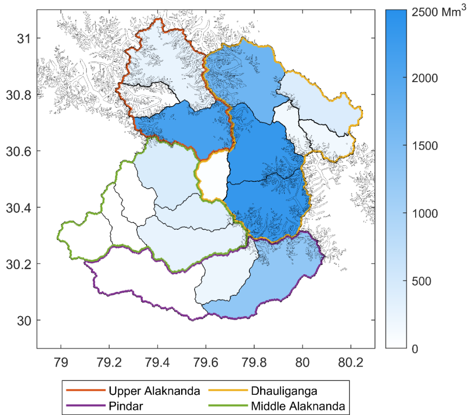
555 Figure 7: Simulated glacier melting in the water years 2001-2020 at sub-basin scale, attributed to the glacier areas represented therein, for Scenario 1.
