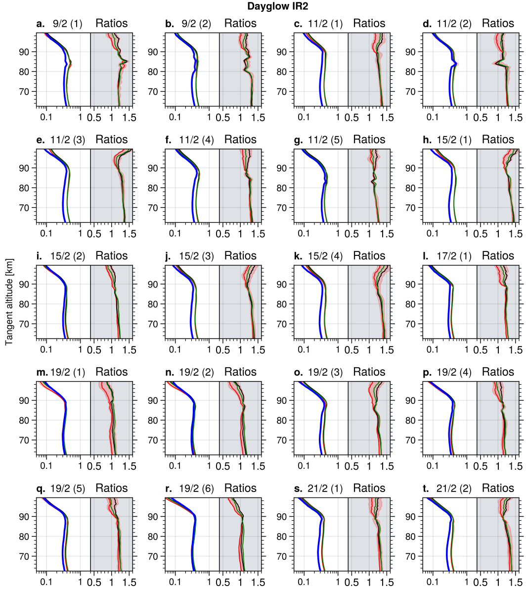
Figure A2. IR2 comparisons when SZA < 90°. The limb radiance is given in 10^{15} \text{ m}^{-2} \text{ s}^{-1} \text{ str}^{-1} \text{ nm}^{-1} .
