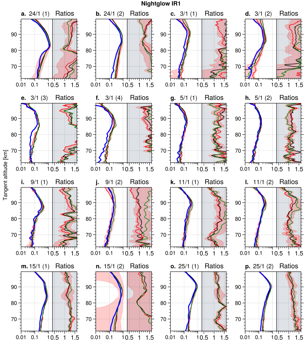
Figure A3. IR1 comparisons when SZA > 100^\circ . Limb radiance is given in units of 10^{14} \text{ m}^{-2} \text{ s}^{-1} \text{ str}^{-1} \text{ nm}^{-1} .
