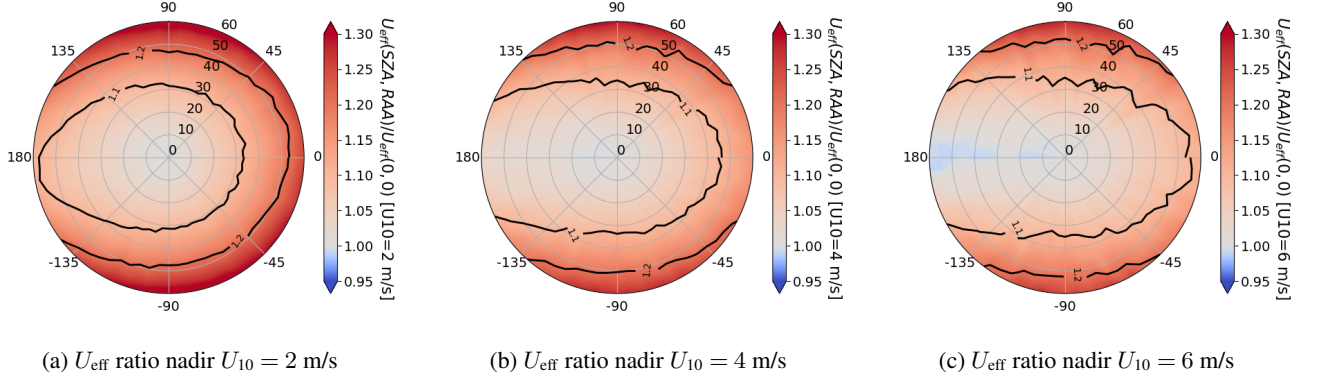
Figure 7. U_{\text{eff}} error ratio against nadir considering Q=3 t/h and noise of 50 ppm. Polar plot represents values of sun angles for a viewing nadir. The angular axis represents the RAA angles and radial axis refers to the SZA angles.
