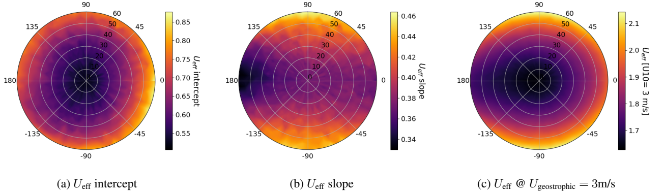
Figure 6. (6a) U_{\text{eff}} intercept, (6b) slope and (6c) reference value at a U_{10} of 3 m/s considering Q=3 t/h and noise of 50 ppm. Polar plot represents values of sun angles for a viewing nadir. The angular axis represents the RAA angles and radial axis refers to the SZA angles.
