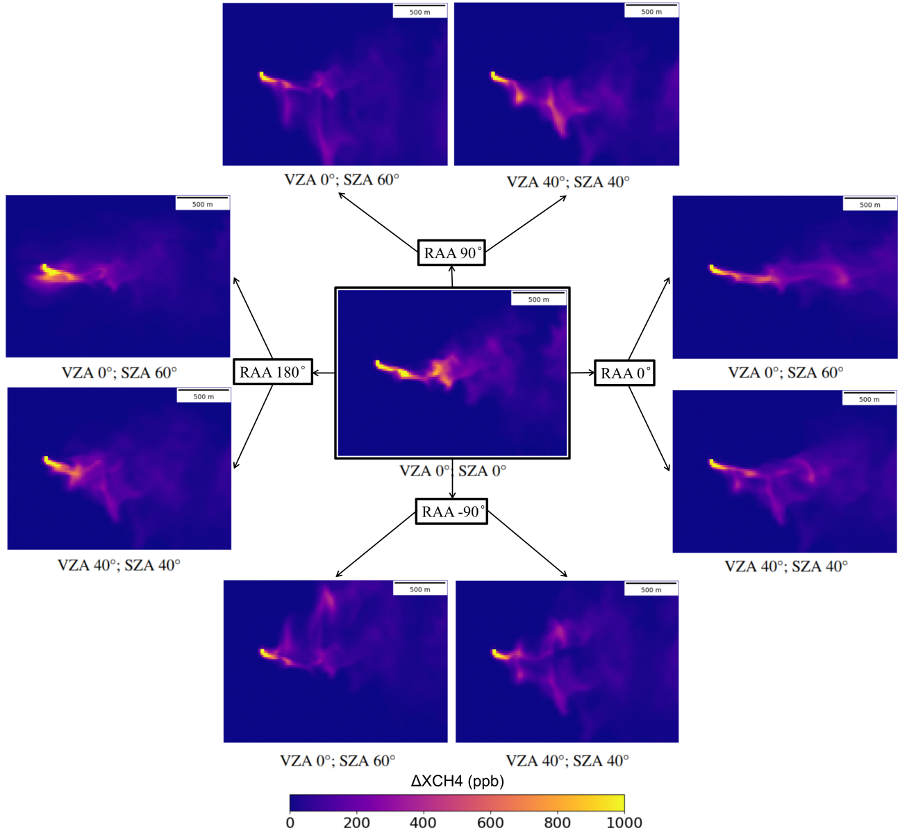
Figure 4. \Delta X_{\text{CH}_4} map at different RAA values for a mid-latitude winter case (SZA 60°, VZA 0°) and a standard angular configuration of a pointing system (SZA 40°, VZA 40°). For all cases the geostrophic wind direction is eastwards RAA = 0°.
