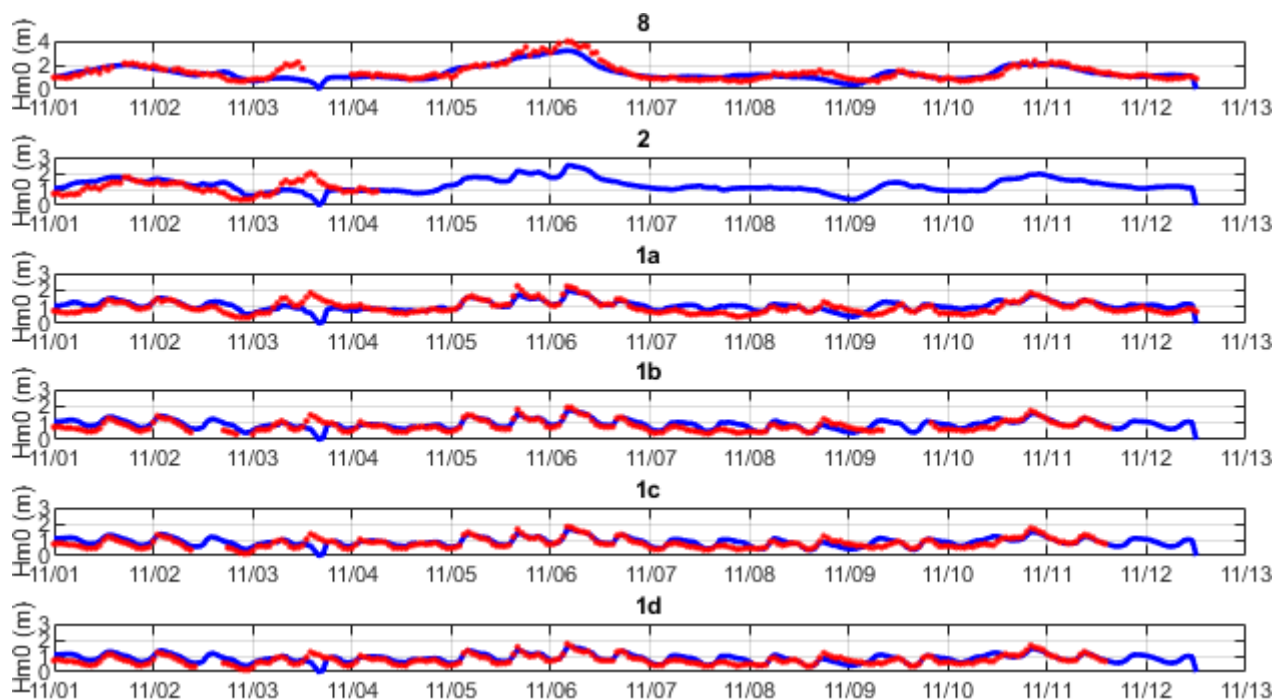
340 Figure 12 Time series of Hm0 wave height at 30 min intervals, measured (red dots) vs computed (drawn blue line). Large-scale model driven by ERA5 boundary conditions, \gamma=0.7 .
