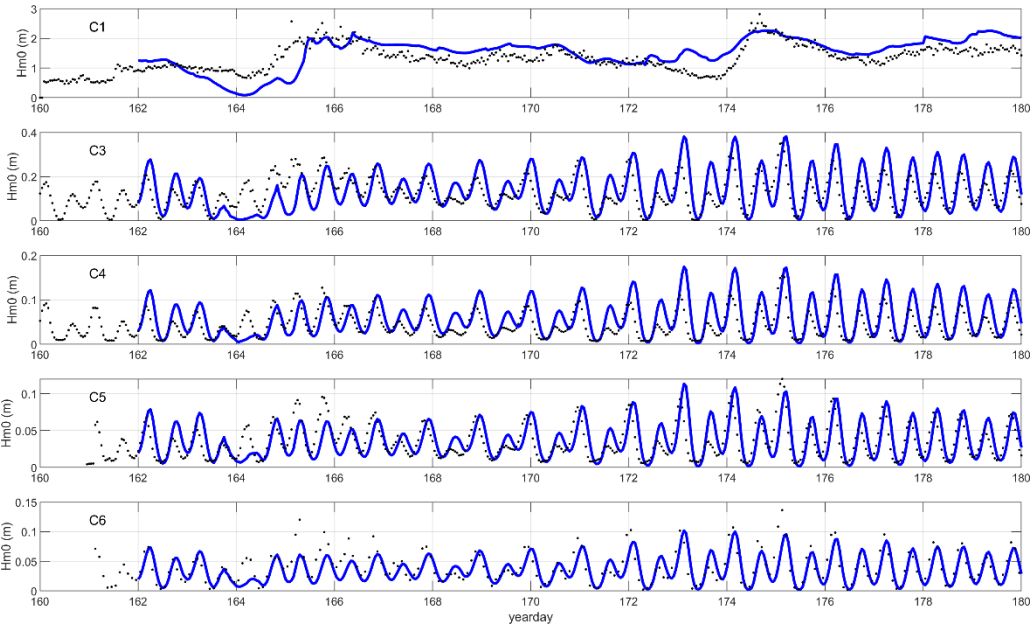
505 Figure 26 Time series of Hm0 wave height across the reef at Ningaloo; observations (black dots) against model simulation (blue drawn lines). Large-scale model.
