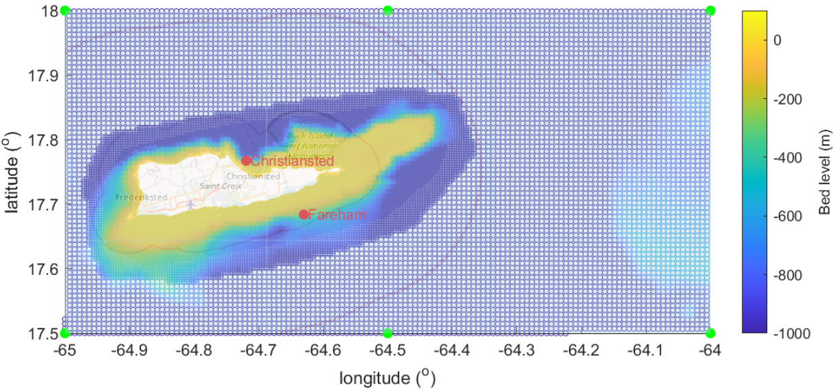
420 Figure 19 Grid layout and bathymetry, St Croix case. Green dots indicate ERA5 boundary locations; red dots indicate the observation points at the site of the CDIP buoys.
