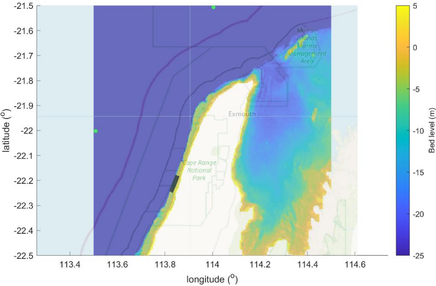
460 Figure 22 Overview of large-scale Ningaloo reef model with bathymetry, boundary points (in green dots) and the location of the local model.
