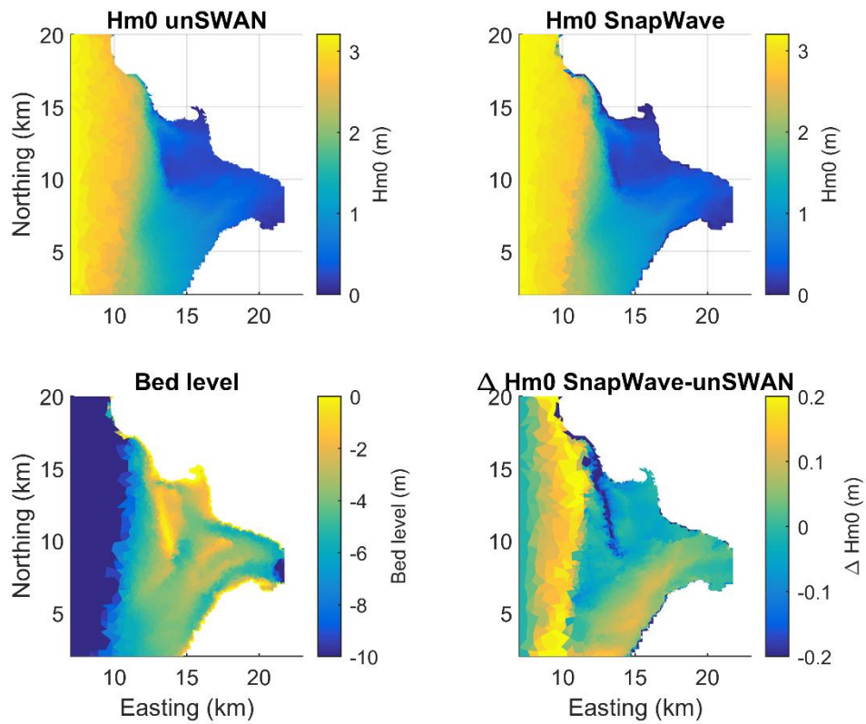
Figure 32 Comparison of unSWAN and SnapWave for the Haringvliet case. Top left and top right panels: Hm0 computed by unSWAN resp. SnapWave; lower left panel: bed level; lower right panel: difference between the models.
