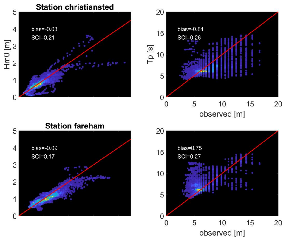
435 Figure 21 Scatter plots (heat maps) of computed vs. observed H_{m0} wave heights (left panels) and T_p wave period (right panels), for stations Christiansted and Fareham, St Croix. For color legend refer to Figure 11.
