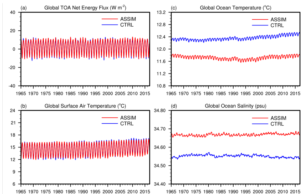
891 892 Figure A1. Time series of (a) global mean top-of-atmosphere (TOA) net energy flux ( \text{W m}^{-2} ), 893 (b) global mean surface air temperature ( ^{\circ}\text{C} ), (c) global mean ocean temperature averaged over 894 the upper 1000 m ( ^{\circ}\text{C} ), and (d) global mean ocean salinity averaged over the upper 1000 m 895 (psu). The blue and red lines denote CTRL and ASSIM, respectively.
