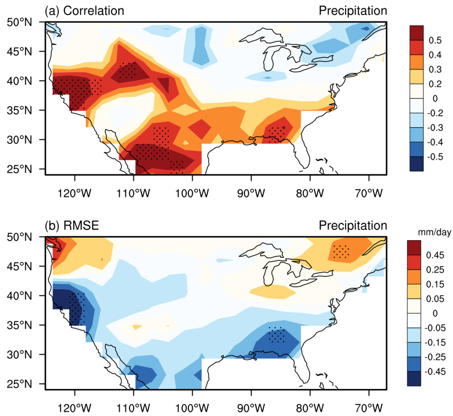
880 Figure 13. Similar to Fig. 12 but for detrended winter precipitation. Dotted areas denote 881 regions where the differences are statistically significant at the 95% confidence level.
