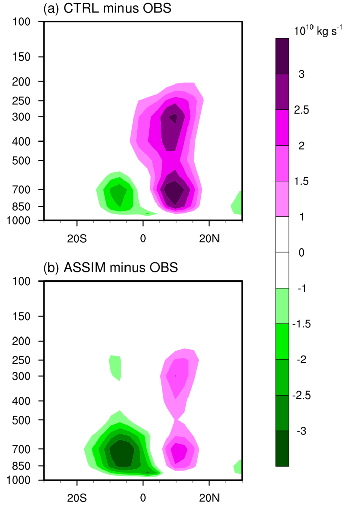
897 Figure A2. Zonal-mean meridional streamfunction differences (units: 10^{10} \text{ kg s}^{-1} ) between 898 model simulations and observations averaged over the period 1980–2016. Panel (a) shows the 899 difference between CTRL and observations, and panel (b) shows the difference between 900 ASSIM and observations. The vertical axis represents pressure levels (hPa), and the horizontal 901 axis denotes latitude.
