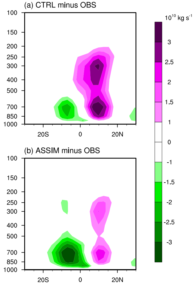
895 Figure A2. Zonal-mean meridional streamfunction differences (units: 10^{10} \text{ kg s}^{-1} ) between 896 model simulations and observations averaged over the period 1980–2016. Panel (a) shows the 897 difference between CTRL and observations, and panel (b) shows the difference between 898 ASSIM and observations. The vertical axis represents pressure levels (hPa), and the horizontal 899 axis denotes latitude.
