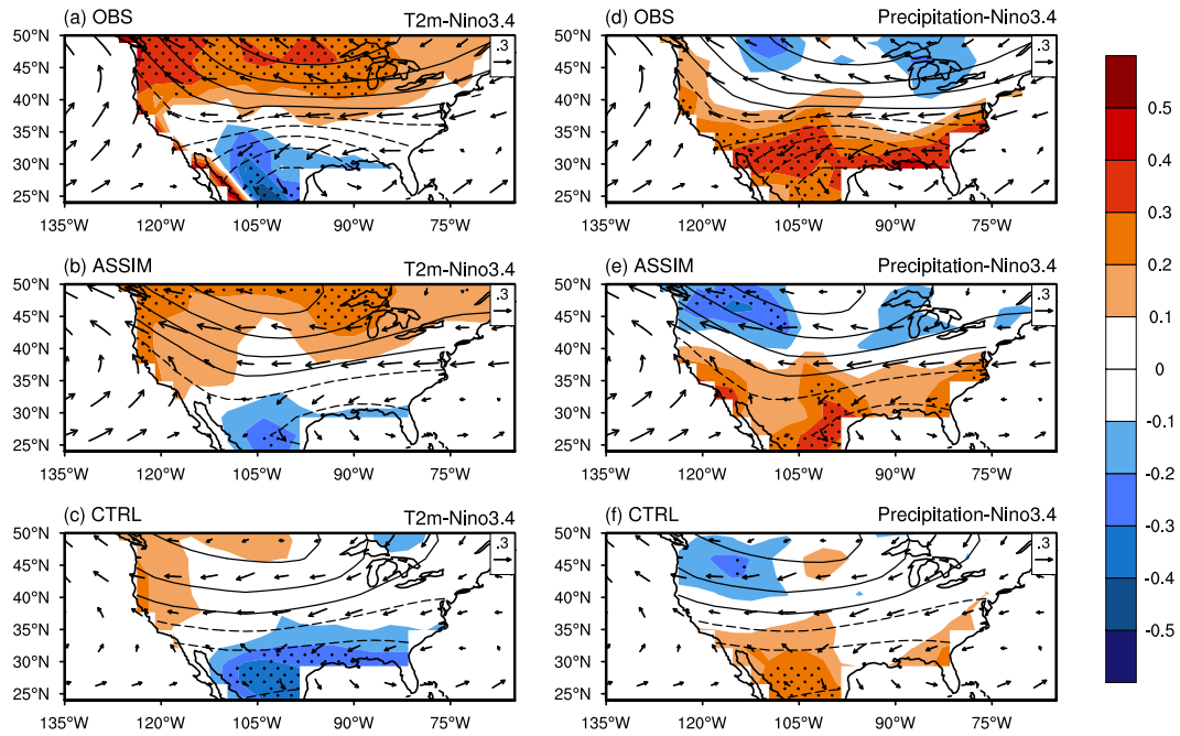
Figure A3. Lagged regression patterns of monthly winter (DJF) surface air temperature (left column; shaded), precipitation (right column; shaded), 500hPa geopotential height (contours), and 850hPa winds (vectors) onto the preceding month's (NDJ) standardized Niño 3.4 index for (a, d) the observation, (b, e) ASSIM, and (c, f) CTRL. Specifically, monthly atmospheric variables from December to February (DJF) are regressed onto the standardized monthly Niño 3.4 index from November to January (NDJ), corresponding to a one-month lead time. The Niño 3.4 index is calculated separately from each corresponding dataset. Dotted areas denote statistical significance at the 95% confidence level.
