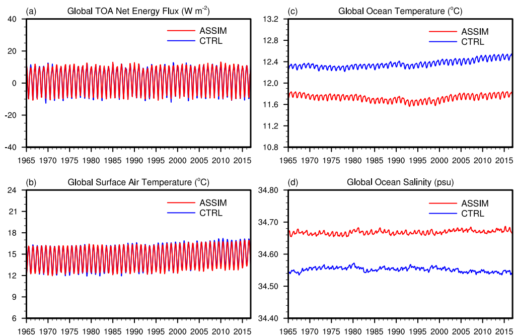
890 Figure A1. Time series of (a) global mean top-of-atmosphere (TOA) net energy flux ( \text{W m}^{-2} ), 891 (b) global mean surface air temperature ( ^{\circ}\text{C} ), (c) global mean ocean temperature averaged over 892 the upper 1000 m ( ^{\circ}\text{C} ), and (d) global mean ocean salinity averaged over the upper 1000 m 893 (psu). The blue and red lines denote the CTRL and ASSIM, respectively.
