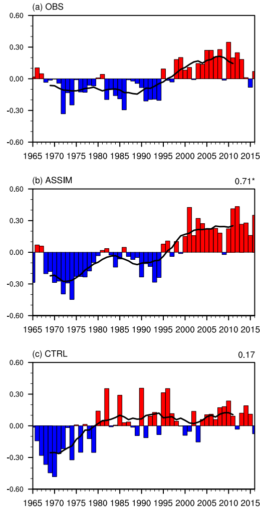
Figure 11. Time series of the Atlantic Multidecadal Oscillation (AMO) index from 1965 to 2016 for (a) the observation, (b) ASSIM, and (c) CTRL. The black line denotes the 10-year running mean. The numbers at the top right of (b) and (c) indicate the temporal correlations of ASSIM and CTRL with observations. The asterisk indicates that the correlation is statistically significant at the 95% confidence level. The AMO index is calculated by subtracting the global mean SST anomalies (60°S–60°N) from the North Atlantic SST anomalies (0–60°N, 0–80°W).
