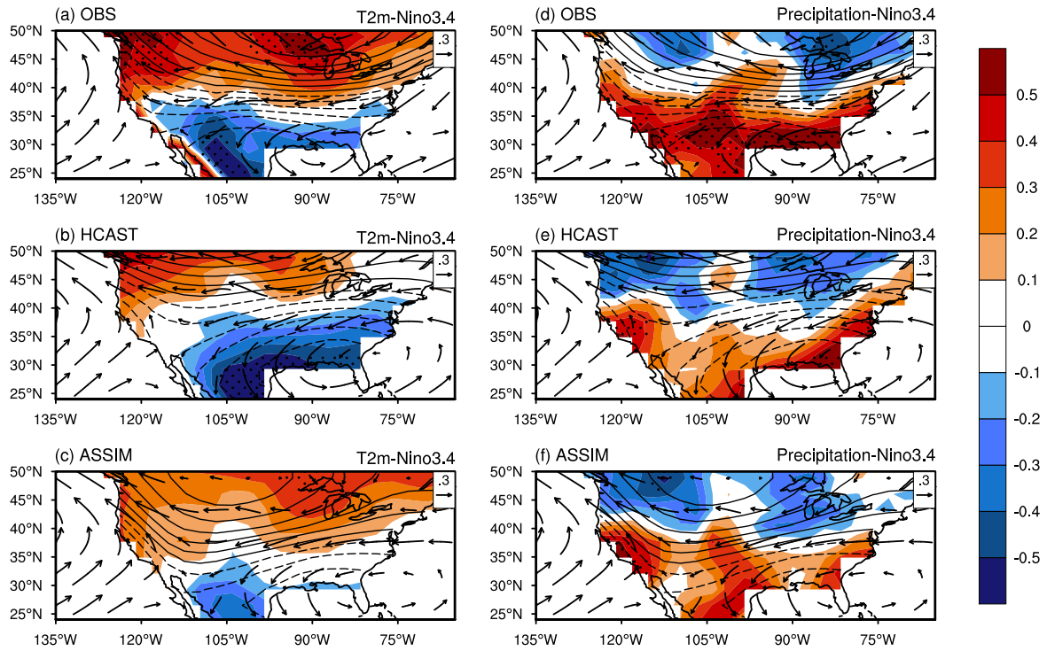
920 Figure A5. Regression patterns of winter surface air temperature (left column; shaded) and 921 precipitation (right column; shaded), 500hPa geopotential height (contours), and 850hPa winds 922 (vectors) on the standardized winter Niño 3.4 index from 1981 to 2010 for (a, d) the observation, 923 (b, e) HCAST, and (c, f) ASSIM. The HCAST results are based on the ensemble mean hindcasts 924 initialized at five-year intervals from 1981 to 2006, as described in Fig. A4. The successive 925 five-year segments are then concatenated to form a continuous time series from 1981 to 2010, 926 without any bias correction applied. Dotted areas indicate regions where the regressions are 927 statistically significant at the 95% confidence level.
