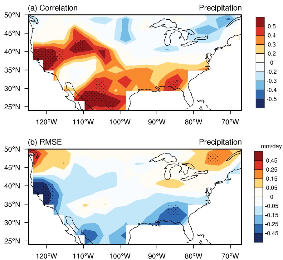
878 Figure 13. Similar to Fig. 12 but for detrended winter precipitation. Dotted areas denote 879 regions where the differences pass the 95% confidence level.
