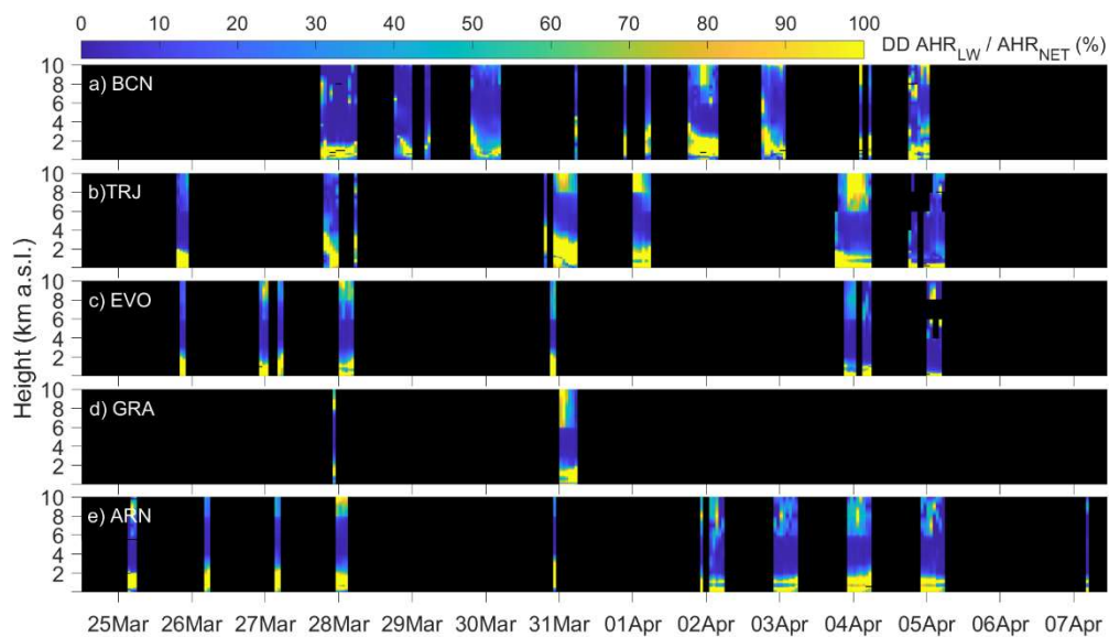
Figure S13. Vertical distribution of the LW-to-net aerosol heating rate ratio ( AHR_{LW}/AHR_{NET} \% ) corresponding to DD particles at the five Iberian lidar stations (from North-East to South-West, by decreasing latitude): a) BCN, b) TRJ, c) EVO, d) GRA and e) ARN.
