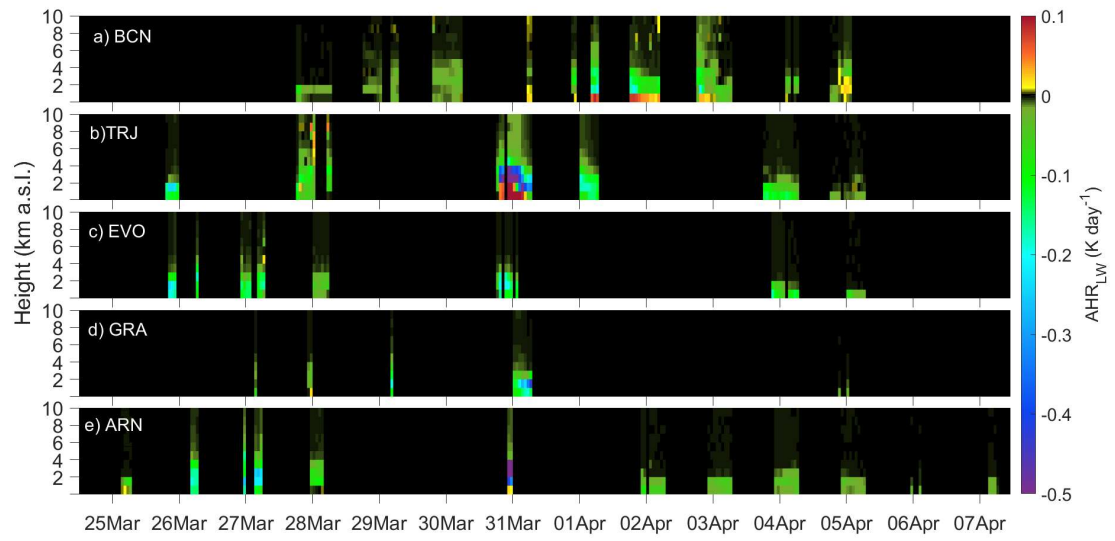
Figure S12. The same as Fig. S11, but in the LW range (AHR LW , K day -1 ).
