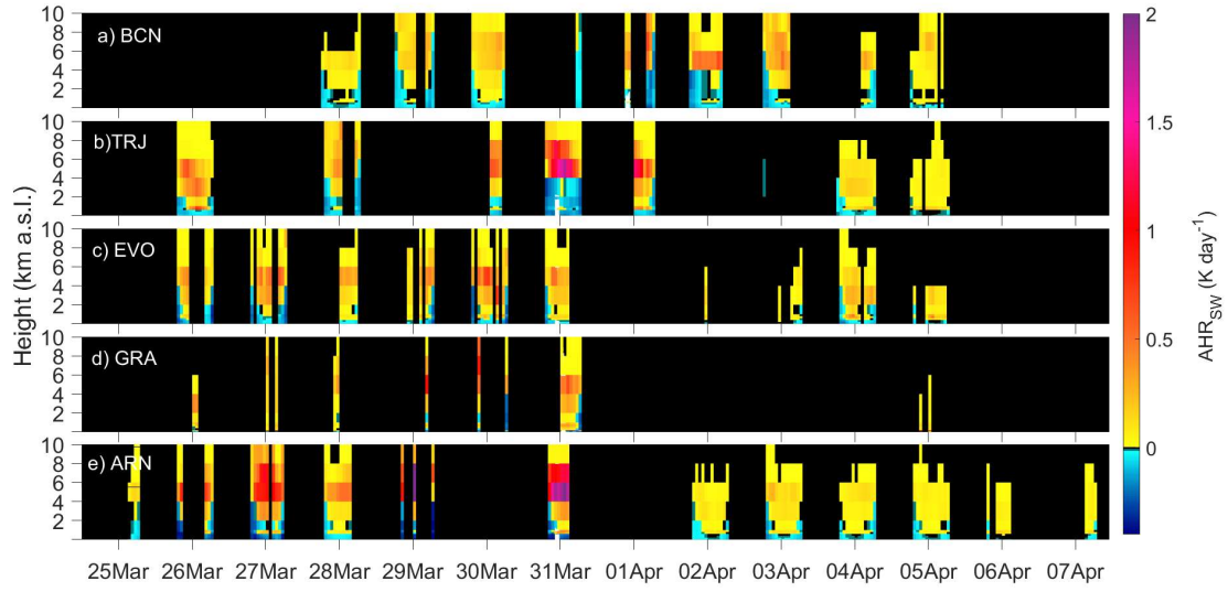
Figure S11. Vertical distribution of the aerosol heating rates in the SW range ( AHR_{sw} , K day^{-1} ) corresponding to DD particles at the five Iberian lidar stations (from North-East to South-West, by decreasing latitude): a) BCN, b) TRJ, c) EVO, d) GRA and e) ARN.
