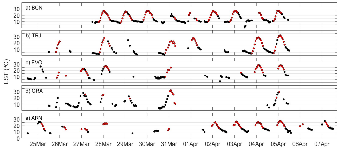
Figure S1. Hourly land surface temperature (LST) at the five Iberian lidar stations (from NE to SW, by decreasing latitude): (a) Barcelona (BCN), (b) Torrejón/Madrid (TRJ), (c) Évora (EVO), (d) Granada (GRA) and (e) El Arenosillo/Huelva (ARN). The associated uncertainty is added as a shaded area, although is so small that it is almost imperceptible. The red dots represent the values coincident with lidar measurements.
