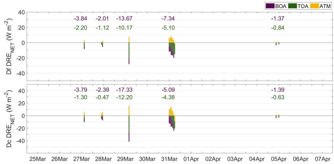
Figure S7. Dust direct radiative effect in the net range (DRE NET , \text{W m}^{-2} ) at BOA (purple), TOA (green) and in the atmosphere (ATM, yellow) at the GRA station, as induced by the (top) fine dust (Df), and (bottom) coarse dust (Dc) particles.
