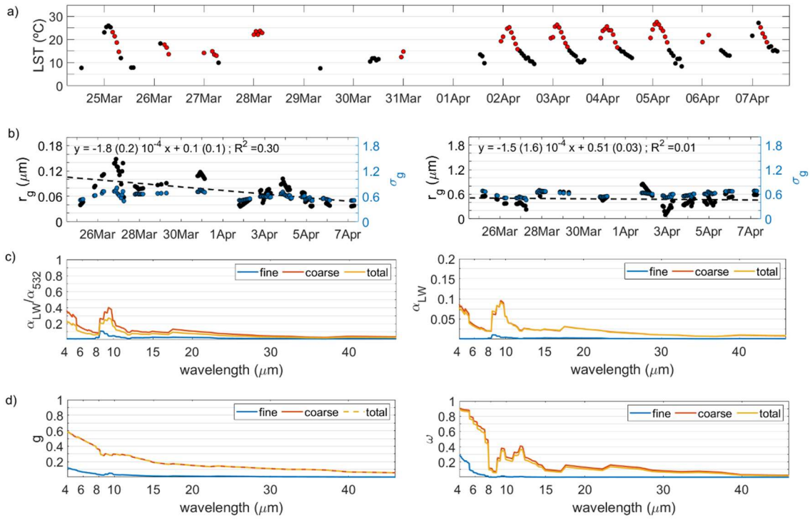
Figure 1. (a) Hourly land surface temperature (LST, in °C), where the red dots represent the cases coincident with lidar measurements; (b) AERONET geometric median radius ( r_g , in \mu\text{m} ) and standard deviation ( \sigma_g ) for the (Left) fine and (Right) coarse modes, where the dashed lines represent the linear fitting of r_g over time; and (c) Episode-averaged values of the (Left) normalized spectral extinction ( \alpha_{LW}/\alpha_{532} ) and (Right) spectral extinction ( \alpha_{LW} , see equation 3) for fine, coarse and total components; (d) (Left) asymmetry factor ( g_{LW} ) and (Right) single scattering albedo ( \omega_{LW} ), for the fine (blue), coarse (red) and total (yellow) modes. All the plots refer to El Arenosillo/Huelva (ARN) station; for the rest of stations, see the Supplementary Material.
