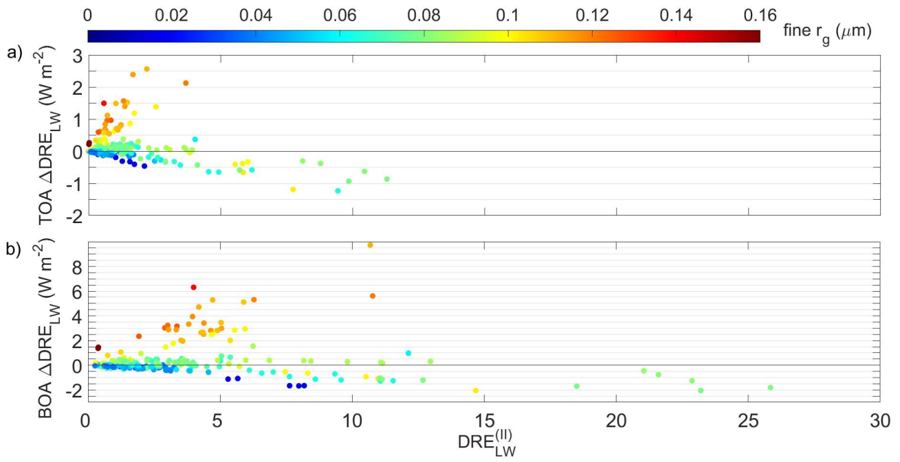
Figure 6. Differences in \text{DRE}_{\text{LW}} as obtained from the two approaches ( \Delta\text{DRE}_{\text{LW}} = \text{DRE}_{\text{LW}}^{(\text{I})} - \text{DRE}_{\text{LW}}^{(\text{II})} , Eq. 3; \text{W m}^{-2} ) as a function of \text{DRE}_{\text{LW}}^{(\text{II})} at: a) TOA, and b) BOA, for all five lidar stations from 25 March to 7 April 2021. The dependence on the fine r_g ( \mu\text{m} ) is shown as a colour-scaled bar at the top.
