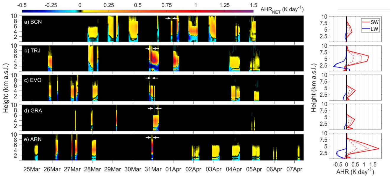
985 Figure 9. Left) Vertical distribution of the net aerosol heating rates ( AHR_{NET} , K day^{-1} ) corresponding to dust (DD) particles at the 986 five Iberian lidar stations (from North-East to South-West, by decreasing latitude): a) BCN, b) TRJ, c) EVO, d) GRA and e) ARN 987 stations. (Right) An example of an hourly-averaged AHR profile for the SW (red) and LW (blue) range at each station. These specific 988 profiles are marked on the left panel between white arrows. Solid, dashed and dotted lines refers to DD, Df and Dc AHR_{NET} , 989 respectively.
