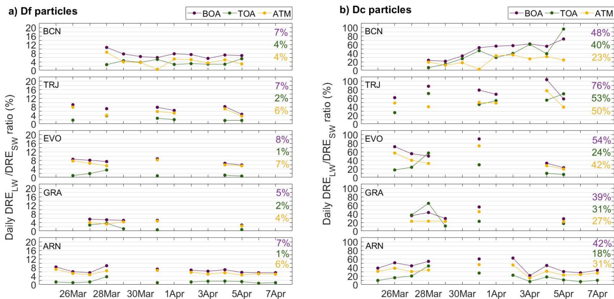
940 Figure 3. Daily DRE_{LW}/DRE_{SW} ratio (%; in absolute units) at the five Iberian lidar stations, at BOA (purple), TOA (green), and in ATM (yellow), corresponding to: a) Df particles, and b) Dc particles. The episode-averaged values are also shown on the right of each panel.
