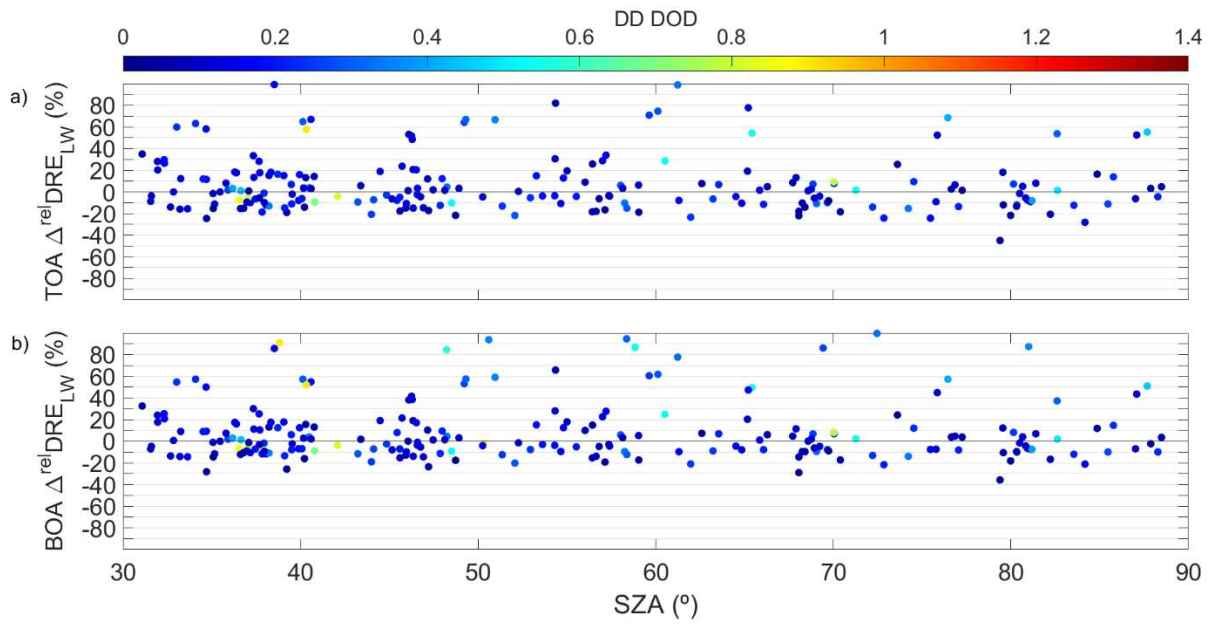
955 Figure 5. Relative differences in DRE LW ( \Delta^{\text{rel}}\text{DRE}_{\text{LW}} , in %) as obtained from the two approaches (Eq. 6) as a function of SZA at: a) TOA, and b) BOA, for all five lidar stations from 25 March to 7 April 2021. The dependence on DD DOD 532 is shown as a colour-scaled bar at the top.
