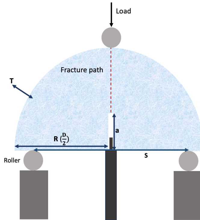
Figure 4. Experiment set up for ice fracture tests with semi-circular bend samples. T refers to sample thickness, R, sample radius, S, the separation between rollers, and a, the notch length. Specimens were loaded via cylindrical rollers, with two lower support rollers and a centrally applied upper loading roller. The support rollers were free to rotate and adjust position slightly during loading, minimising frictional resistance and ensuring appropriate boundary conditions. The loading configuration was symmetric about the notch plane. Dimensions used for the experiments can be found in Table 1.
