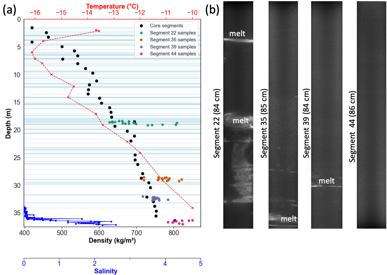
Figure 2. (a) Density measurements for whole segments (black) measured in the field, and smaller samples cut from the same segments used for fracture analysis (green, orange, purple, pink) measured in the lab. The spread in density of the smaller samples is due to some samples containing refrozen melt, which increases those samples' density relative to the average segment density. Refrozen melt layers within the core are shown by the background blue bands. Red dashed line shows temperature data recorded at specific depth intervals using TinyTag loggers. (b) Line-scanned segments for segment 22 (with a top depth of 16.45 m), segment 35 (27.67 m), segment 39 (31.07 m) and segment 44 (35.92 m). Line scan data highlight the melt within the segments.
