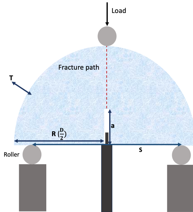
Figure 4. Experiment set up for ice fracture tests with semi-circular bend specimen. T refers to sample thickness, R , sample radius, S , the separation between rollers, and a , the notch length. Specimens were loaded via cylindrical rollers, with two lower support rollers and a centrally applied upper loading roller. The support rollers were free to rotate and adjust position slightly during loading, minimising frictional resistance and ensuring appropriate boundary conditions. The loading configuration was symmetric about the notch plane. Dimensions used for the experiments can be found in Table 1.
