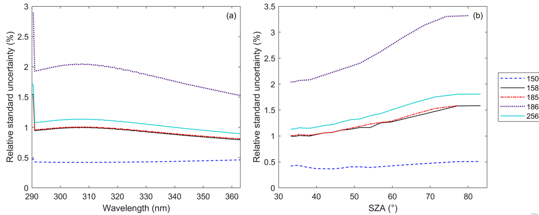
Figure 7. Relative standard uncertainty on 13 September 2023 caused by the cosine correction implemented. (a) Spectral dependency at 12:30 UTC. (b) SZA dependency at 305 nm.
