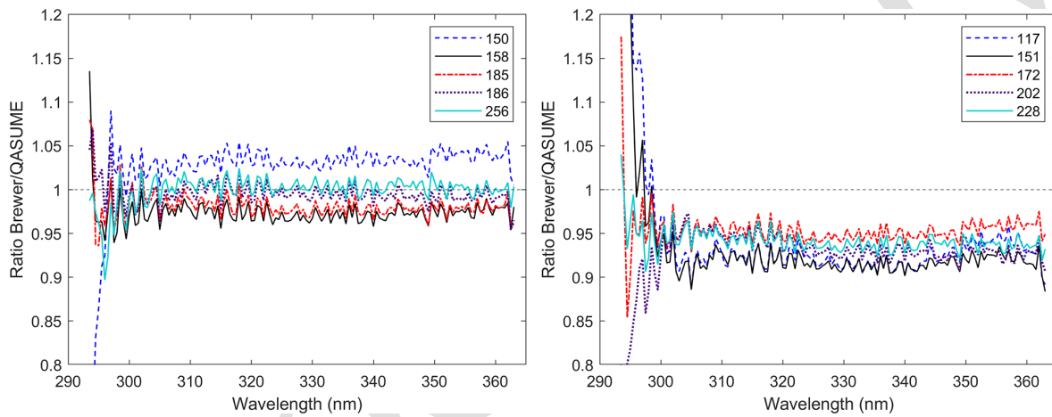
Figure 4. Global irradiance ratio to the QASUME recorded on 13 September at 14:00 UTC. (a) First group (double Brewers with cosine correction). (b) Second group (two single and three double Brewers with no cosine correction implemented).
