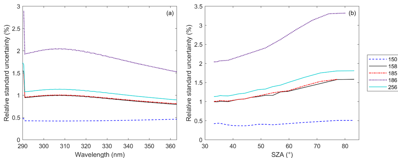
Figure 7. Relative standard relative uncertainty on 13 September 2023 caused by the cosine correction implemented. (a) Spectral dependency at 12:30 UTC. (b) SZA dependency at 305 nm.
