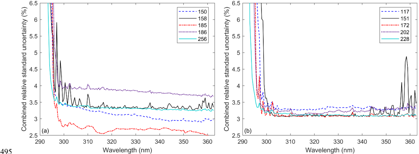
Figure 2. Relative combined standard uncertainties of the UV irradiances shown in Fig. 1. (a) First group (double Brewers with cosine correction). (b) Second group (two single and three double Brewers with no cosine correction implemented).
