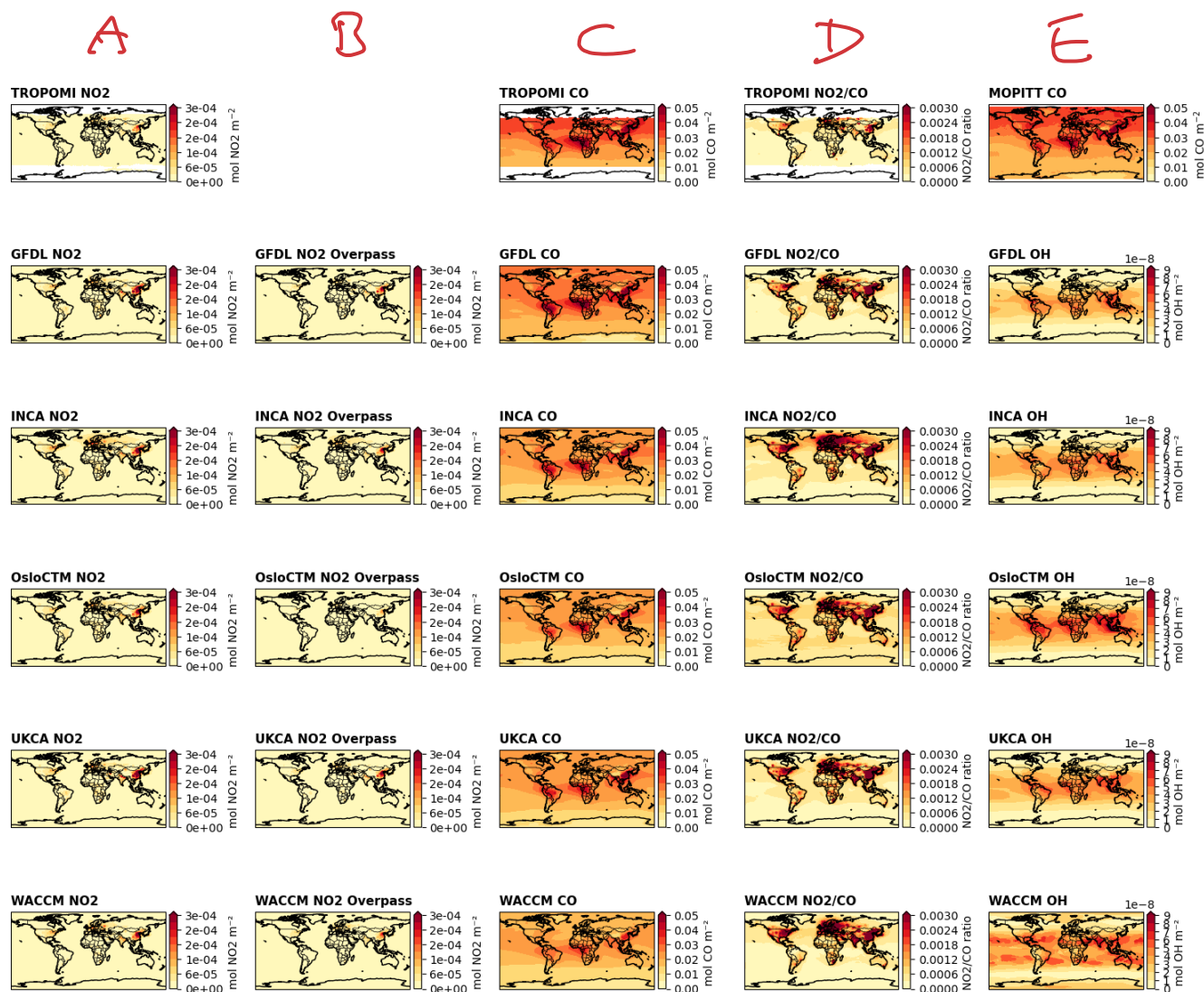
430 Figure A3: Similar to Fig. 3, but including a column estimating model NO 2 during overpass using the ratio of overpass time NO 2 to monthly mean NO 2 from the 3-hourly OsloCTM3 simulations. Global maps of annual mean satellite retrievals for (a) NO 2 for TROPOMI and models; (b) NO 2 for the models with monthly mean values multiplied by the ratio of monthly mean:3-hourly values during overpass for OsloCTM3; (c) CO for MOPITT, TROPOMI and models; (d) NO 2 /CO values in the models, and (e) OH in the models other than UCI.
