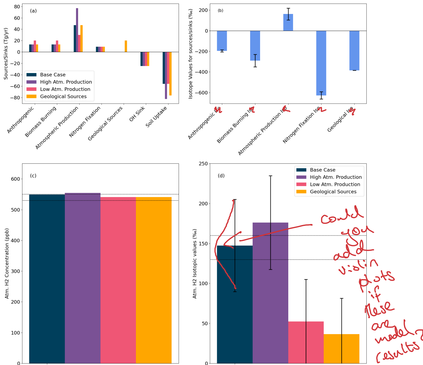
Figure 9: Box model results with isotopic calculations for the Base case (dark blue bars), high atmospheric production (purple), low atmospheric production (pink) and geological sources (yellow) (a) showing the burdens for different sources and sinks used in the box model; (b) isotopic values for the sources used in box model; (c) calculated H 2 concentration; and (d) calculated isotopic values for tropospheric H 2 for the different cases. The dashed black lines show the observed range in (c) H 2 concentration taken here as 530-550 ppb to account for changes in concentrations since Novelli et al. (1999) and (d) H 2 isotopic compositions from Gerst and Quay (2001).
