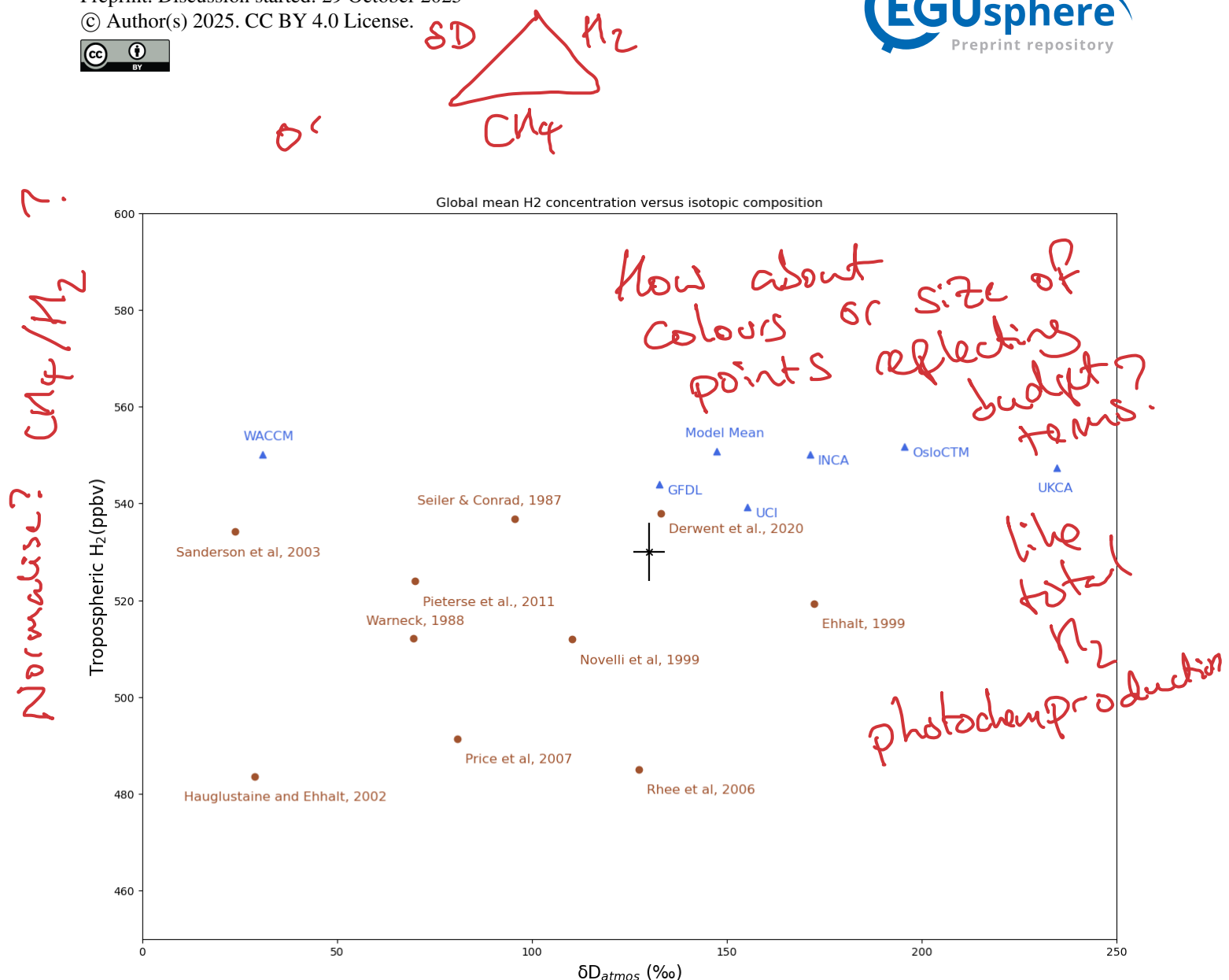
Figure 8: Relationship between atmospheric hydrogen mole fraction and isotopic composition ( \delta D ) from different models (triangles) and published literature (circles). The cross indicates the observed range of lower tropospheric H_2 concentrations between 1991-1996 of 531 \pm 6 ppb (Novelli et al., 1999) and \delta D values (Price et al., 2007; the sensitivity to using values from Pieterse et al., 2011 is shown in Fig. A4). The model concentrations are higher than observed possibly because they are calibrated for more recent observations. (Paulot et al., 2024) suggests an increasing trend of \sim 1.7 ppb/year.
