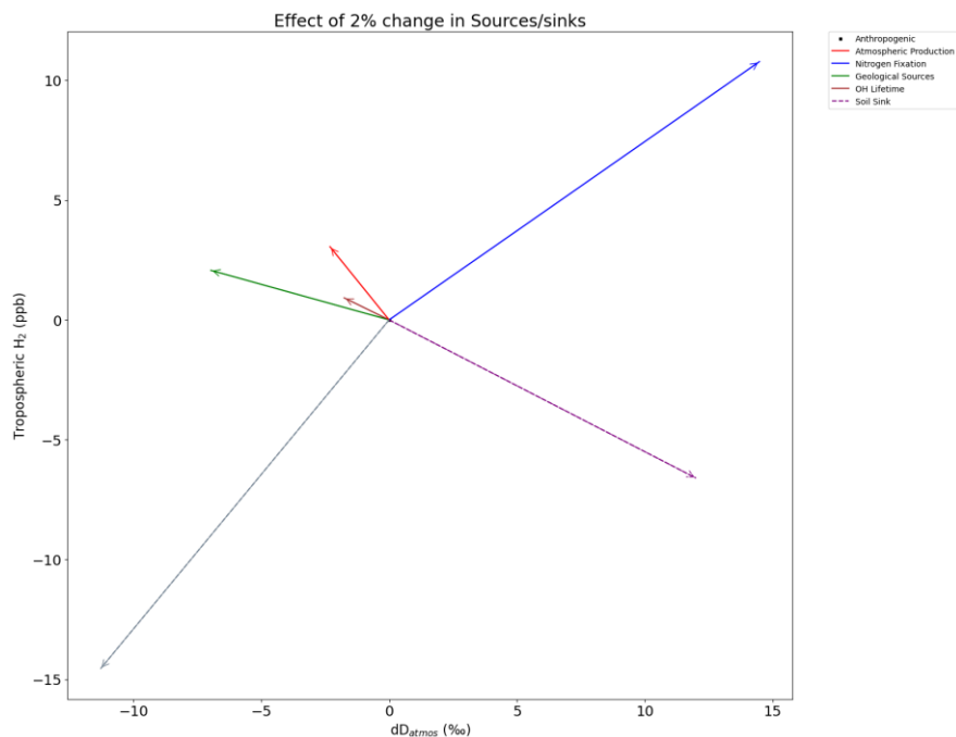
445 Figure 108: Impact of a 2% change in individual sources and sinks on the tropospheric mole fraction and the isotopic composition of H 2 .
