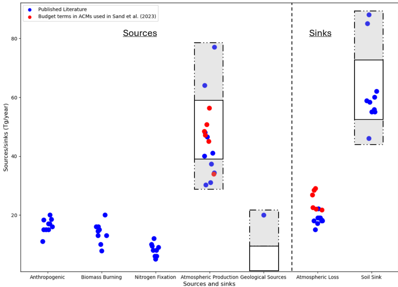
Figure 419: Sources and sinks in the tropospheric hydrogen budget, showing updated ranges for atmospheric production, atmospheric loss based on this study. The grey shaded area with dashed outlines represents previously reported ranges, while the solid white boxes indicate the updated ranges. Model values are shown for the atmospheric production and loss terms that are analyzed in this study.
