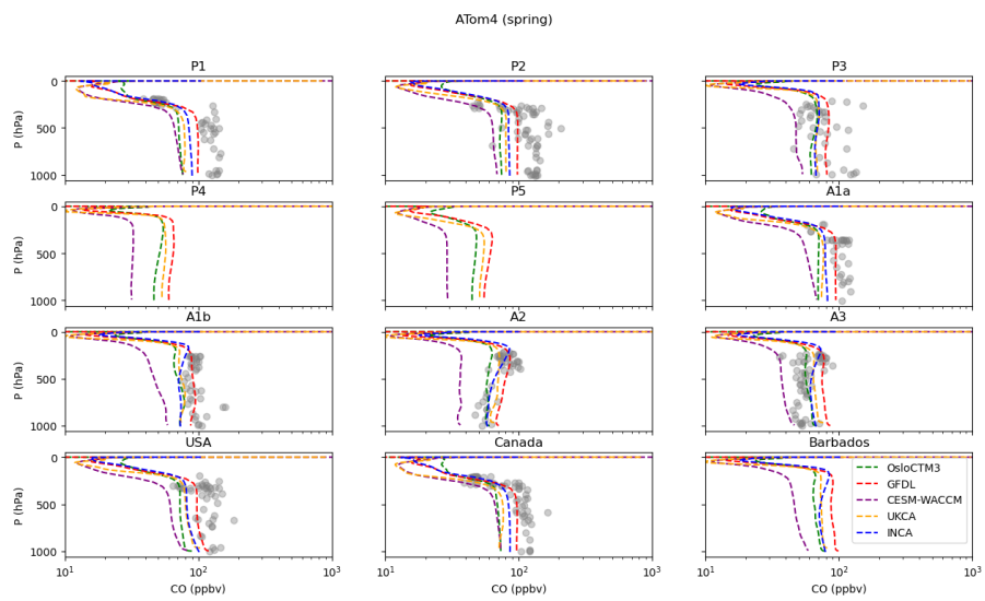
Figure A2A7: Similar to Fig. A1A6 but for vertical profiles of carbon monoxide against observations from the ATom campaigns.
