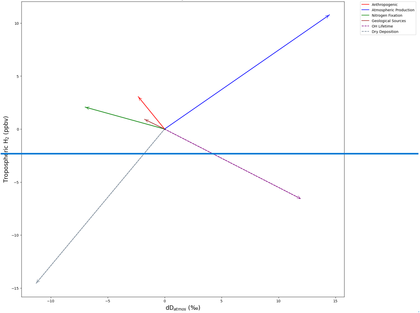
Effect of 2% change in Sources/sinks
