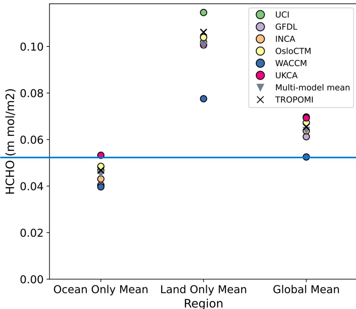
220 Figure 2: Comparison of annual mean formaldehyde over ocean, land, and global from TROPOMI satellite retrievals for 2010 (black crosses), six different ACMs (colored circles) and the multi-model mean (inverted triangle).
