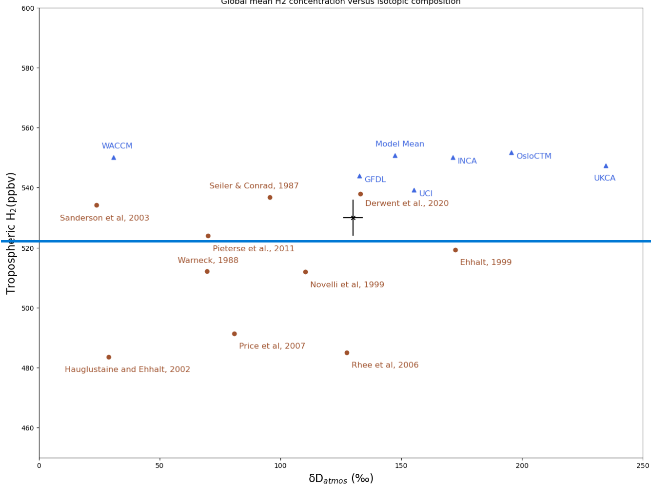
Global mean H 2 concentration versus isotopic composition
