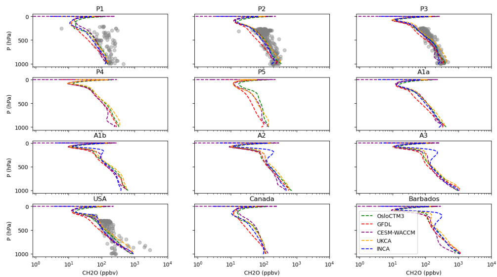
Figure A6: Vertical profiles of formaldehyde (HCHO) compared against observations from four different ATom campaigns. Each panel corresponds to a specific geographical box, defined by latitude and longitude bounds: P1 (180°W to 135°W, 60°N to 90°N): Polar North Pacific; P2 (180°W to 135°W, 30°N to 60°N): Mid-latitude North Pacific; P3 (180°W to 135°W, 0°N to 30°N): Equatorial North Pacific; P4 (160°E to 135°W, 30°S to 0°S): Equatorial South Pacific; P5 (160°E to 135°W, 60°S to 30°S): Mid-latitude South Pacific; A1a (45°W to 10°W, 30°N to 60°N): Mid-latitude North Atlantic; A1b (45°W to 10°W, 0°N to 30°N): Equatorial North Atlantic; A2 (45°W to 10°W, 30°S to 0°S): Equatorial South Atlantic; A3 (65°W to 30°W, 60°S to 30°N): Western Atlantic; USA (135°W to 80°W, 30°N to 60°N); Canada (135°W to 45°W, 60°N to 90°N); Barbados (80°W to 45°W, 0°N to 30°N).
