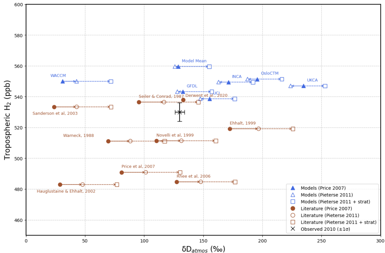
585 Figure A4A9: Similar to Fig. 8, but using isotopic compositions for sources and sinks from (Pieterse et al., 2011) and 29‰ as stratospheric contribution.
