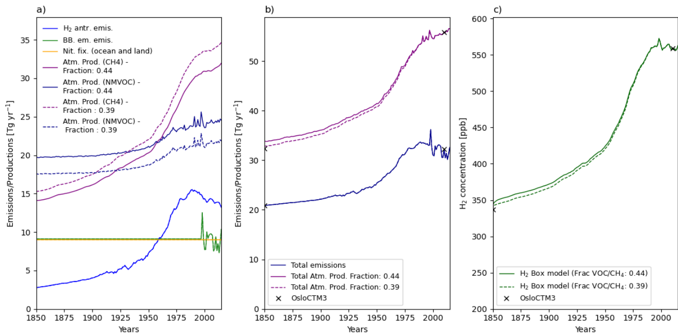
Figure 63: Similar to Fig. 52, but with different relative contributions of atmospheric production via CH 4 and VOCs. Solid lines represent values from a box model simulation with a VOC/CH 4 production ratio of 0.44 from Ehhalt and Rohrer, (2009), while stippled lines indicate results from a box model simulations with the ratio of 0.39 from (Paulot et al., 2024).
