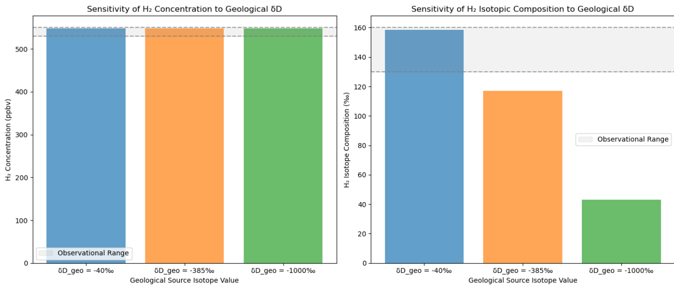
Figure A5A10: Effect of different isotopic compositions for a geological source of 9 Tg/yr.
