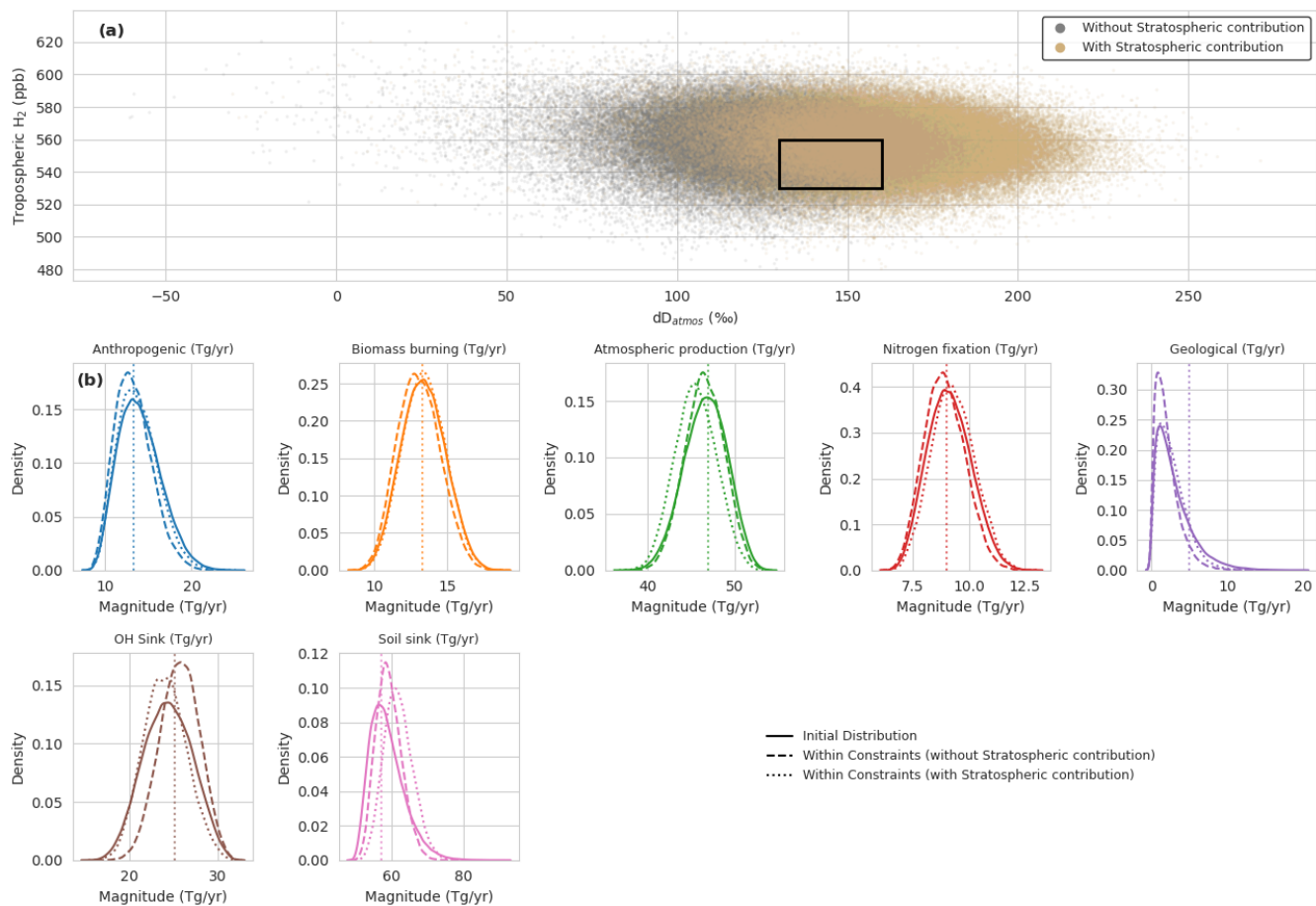
430 Figure 7: Joint analysis of the different sources and sinks and isotopic compositions and the resulting probably density function changes with and without stratospheric contribution. The distributions for the different sources and sinks are all beta- distributions within the ranges found in published literature and models, while for geological sources we used a log-normal distribution for the source term. The isotopic ranges are the minimum and maximum values found in literature. The box model is run 100,000 times with samples being randomly picked from the distributions. For the stratospheric contributions, a value between 29-37‰ is also randomly picked and added to calculate the final isotopic composition of the atmospheric H 2 . 435
