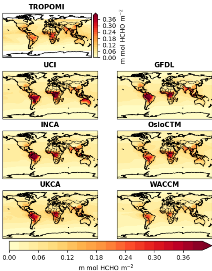
215 Figure 1: Spatial comparison of formaldehyde between TROPOMI satellite retrievals for 2010 July 2018 – June 2019 and the different Atmospheric Chemistry Models listed in Table 1.
