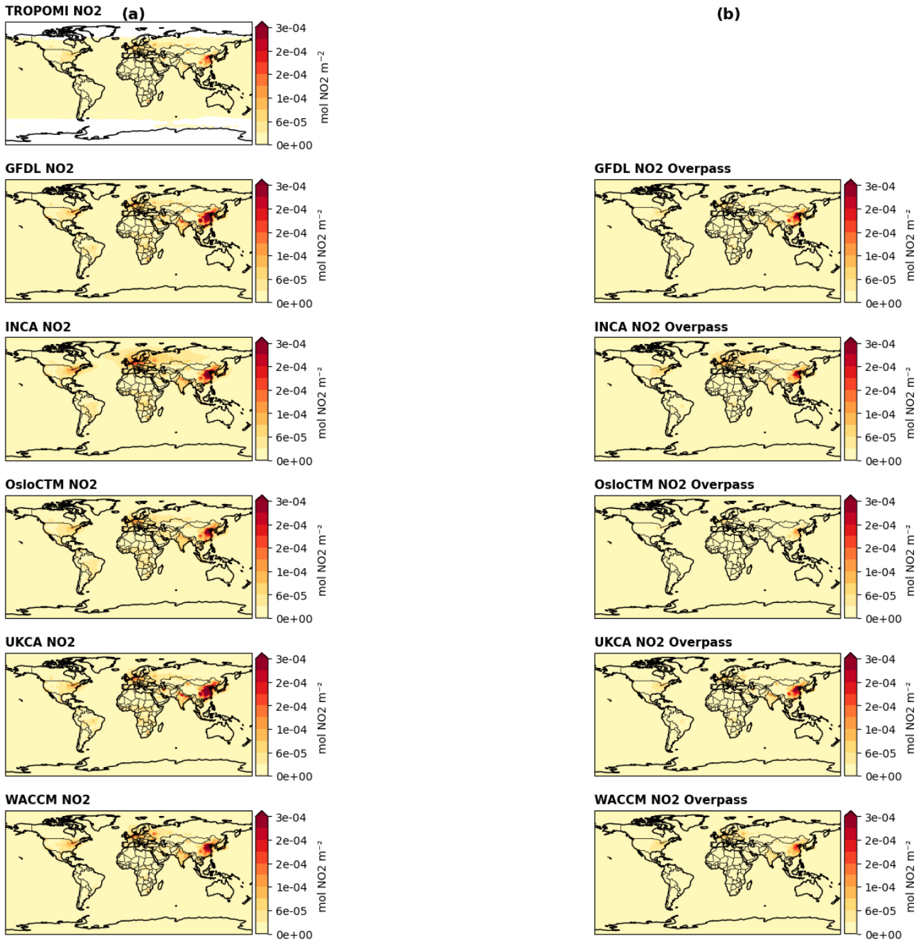
Figure A3: Similar to Fig. 3, but including a column estimating model NO 2 during overpass using the ratio of overpass time NO 2 to monthly mean NO 2 from the 3 hourly OsloCTM3 simulations. A8: Global maps of annual mean satellite retrievals for (a) NO 2 for TROPOMI satellite retrievals for June 2009-June 2010 and models; (b) NO 2 annual mean model NO 2 ; and (b) model NO 2 during overpass for the models with-calculated as the product of monthly mean values multiplied-by-with the ratio of monthly mean:3-
