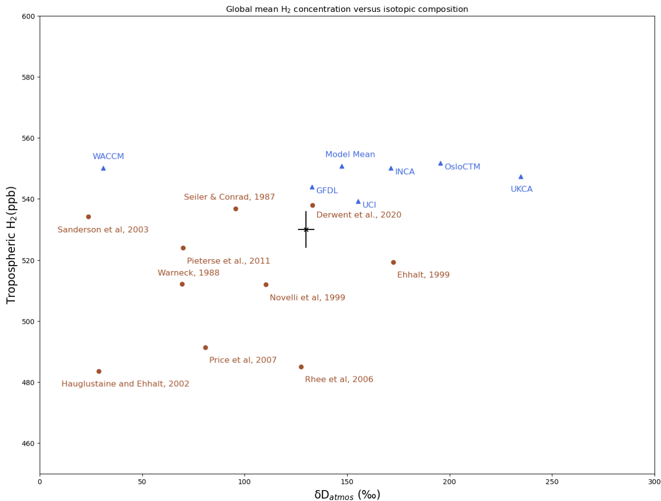
Figure 85: Relationship between atmospheric hydrogen mole fraction and isotopic composition ( \delta D ) from different models (triangles) and published literature (circles). The cross indicates the observed range of lower-tropospheric H 2 concentrations between 1991-1996 of 531±6 ppb (Novelli et al., 1999) and \delta D values (Price et al., 2007; the sensitivity to using values from Pieterse et al., 2011 is shown in Fig. A4A9). The model concentrations are higher than observed possibly because they are calibrated for more recent observations. (Paulot et al., 2024) suggests an increasing trend of -1.7ppb/year. The model concentrations are higher than observed because they are calibrated for more recent observations.
