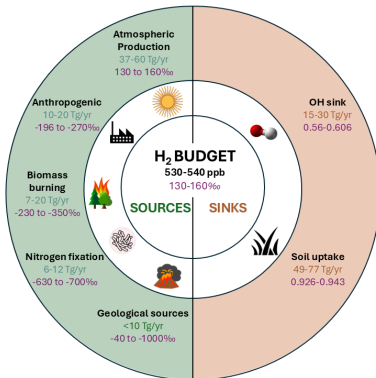
500 Figure 4210: An updated estimate of source and sink ranges based on existing literature and this study. Numbers include the range of sources (green) and sinks (brown) in Tg/yr and isotopic values of sources and fractionation factors for the sinks (in purple).
