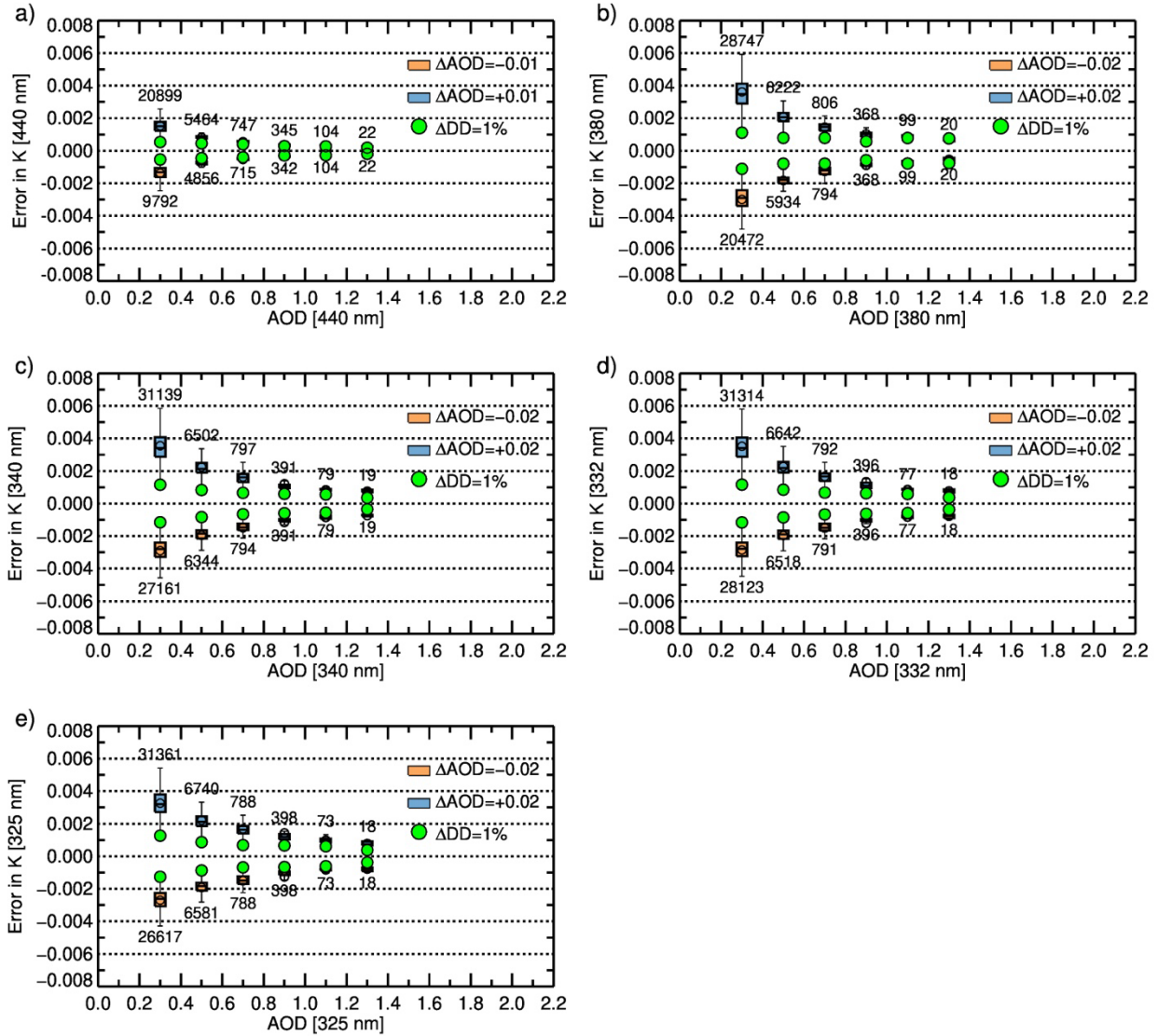
Figure 7. Errors in the MFRSR-retrieved spectral imaginary part of the index (K) resulting from 1) the uncertainties in the AERONET-measured AOD (orange and blue boxes) and 2) 1% change in the MFRSR-measured diffuse-to-direct irradiance ratio (filled green circles). Data represent MFRSR record from 2019-2023. Box-and-whisker elements indicate the interquartile range (25 th -75 th percentiles; boxes) and 1.5 times IQR (whiskers); mean values are shown as open circles and median values as horizontal lines.
