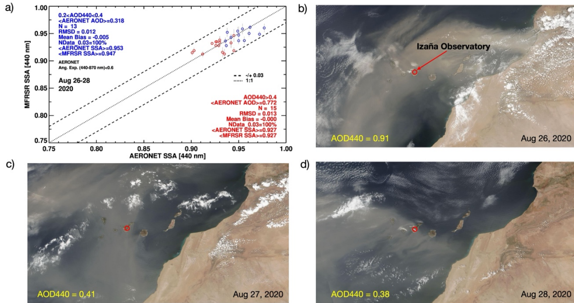
Figure 9. a) Comparison of the MFRSR vs. AERONET retrieved SSA at 440 nm for the data acquired on August 26, 27, and 28 of 2020. Blue and red circles represent temporally matched data with coincident AERONET-measured AOD (440 nm) 0.2-0.4 and >0.4 , respectively. The statistics of the comparison for different AOD conditions are included within the plots. The true-color RGB images acquired from Suomi-NPP/VIIRS sensor for three dates are shown in b), c), and d).
