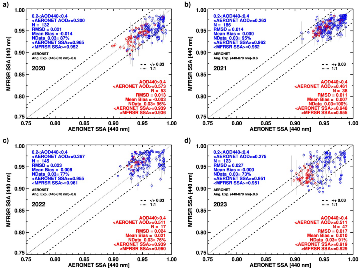
Figure 12. Comparison of MFRSR (y-axis) vs. AERONET (x-axis) SSA at 440 nm for the 2020-2023 (a through d) operation period of MFRSR measurements at Izaña site derived assuming empirically derived aspect ratios. Matchup data points in red (blue) represent AOD 440 > 0.4 (0.2 < AOD 440 < 0.4) conditions. The statistical measures of the comparison are included within individual plot.
