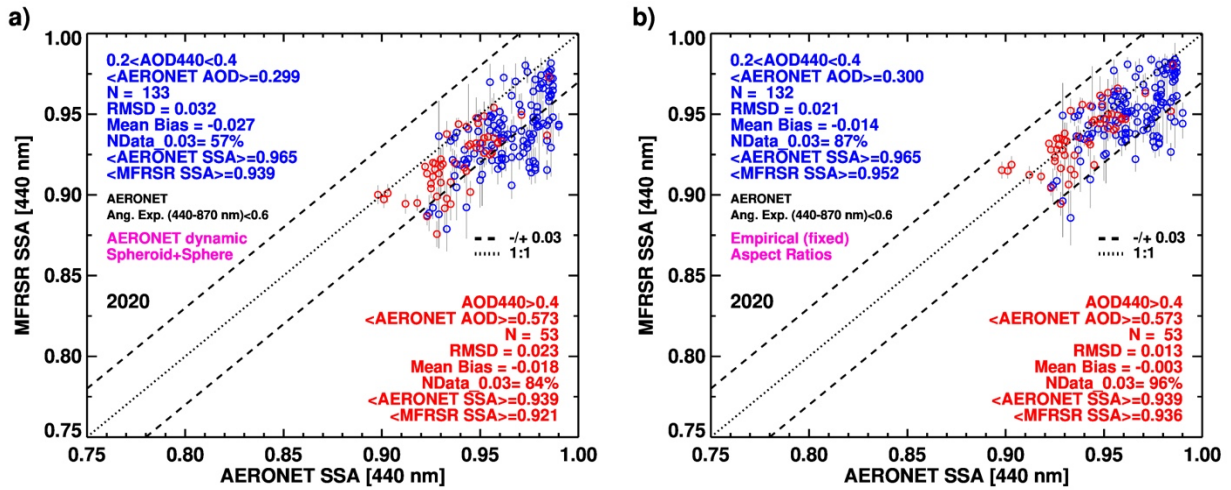
Figure 11. Comparison of MFRSR (y-axis) vs. AERONET (x-axis) SSA at 440 nm for the matchup data collected during 2020 at Izaña site derived assuming a) AERONET-like ‘mixing’ approach combining sphericity-weighted randomly oriented spheroid (Dubovik et al., 2006) and sphere, and b) empirically derived aspect ratios adopted in the over-ocean dust aerosol models used for near-UV aerosol algorithm of OMI, EPIC, and TROPOMI sensors. SSA matchup data points in blue and red represent the coincident AOD 440 conditions of 0.2-0.4 and >0.4, respectively. The statistics of the comparison for different AOD conditions are included within the plots.
