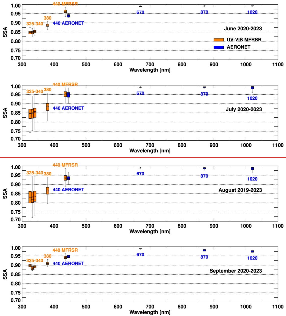
Figure 14. Same as in Figure 12 but for the retrieved spectral SSA.
