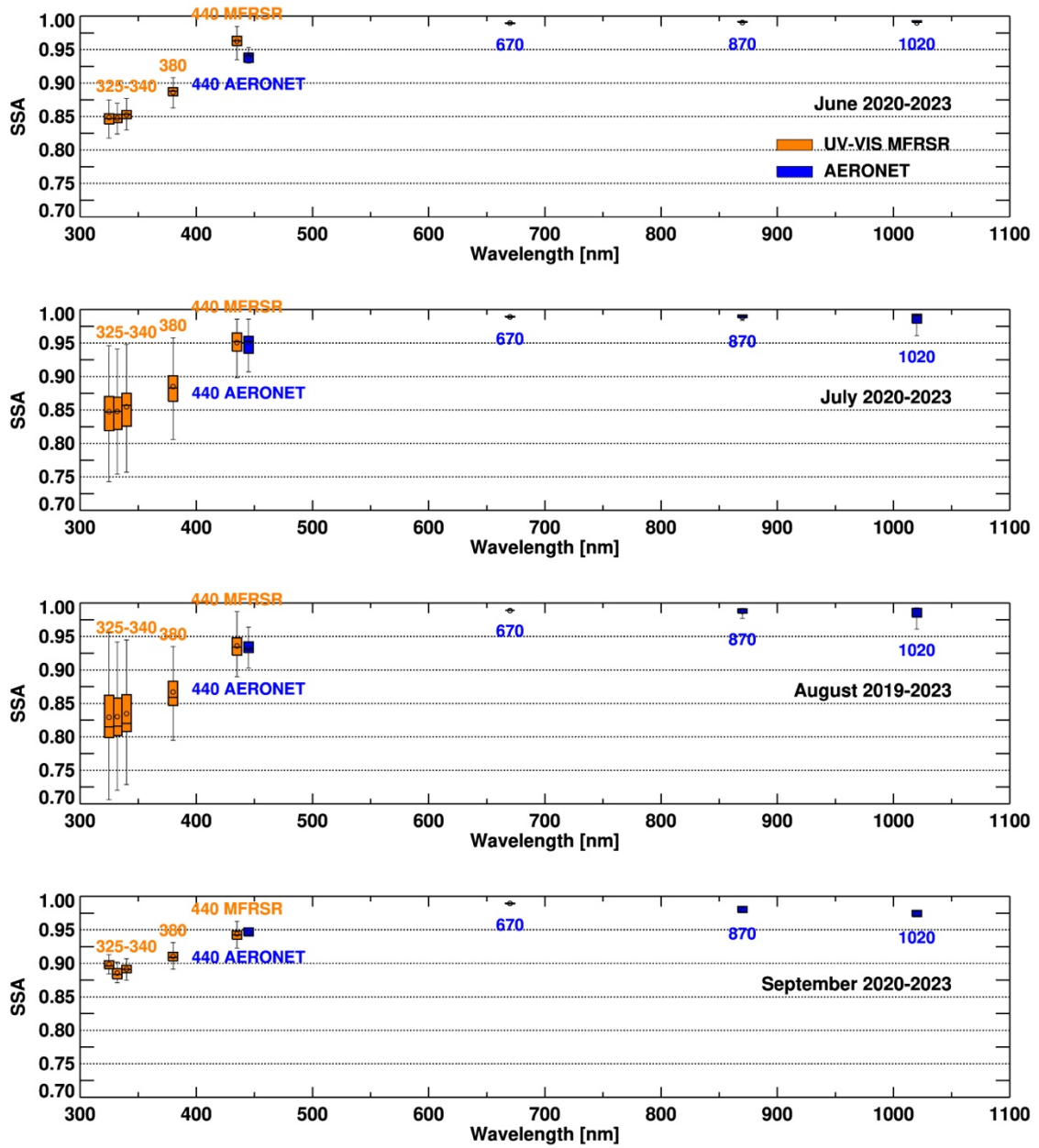
Figure 15. Same as in Figure 14 but for the retrieved spectral SSA.
