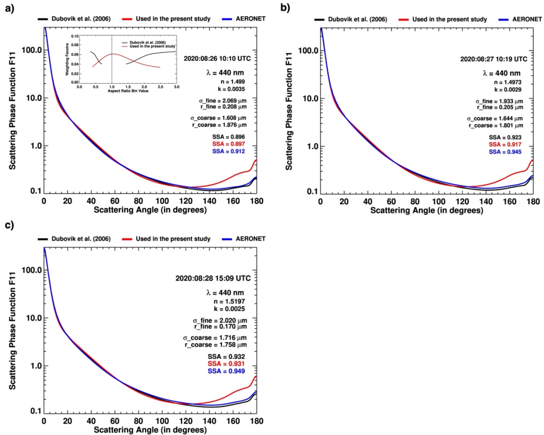
1025 Figure 5. Aspect Ratio distribution distributions and corresponding weighting factors representing randomly oriented 1030 spheroids. The black and red curves represent the aspect ratio distribution data obtained from Dubovik et al. (2006) and the empirically derived distribution used in the present study, as explained in the text. Scattering phase function F11 (440 nm) of mineral dust aerosols retrieved on a) August 26 at 10:10 UTC, b) August 27 at 10:19 UTC, and c) August 28 at 15:09 UTC of 2020 corresponding to randomly oriented spheroids in Dubovik et al. (2006) (black), empirically derived distribution (red) used in the present study, and that from AERONET inversion product (blue). F11 (except for AERONET) was simulated using the SDLS software package for a single MFRSR-AERONET collocated measurement for the respective dates. Aspect ratio distribution proposed by Dubovik et al. (2006) and that used in the presented study are shown as an inset in the top-left plot (a).
