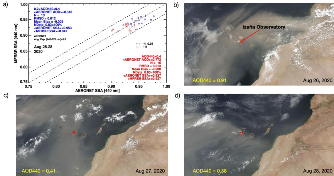
1050 Figure 97. a) Comparison of the MFRSR vs. AERONET retrieved SSA at 440 nm for the data acquired on August 26, 27, and 28 of 2020. Blue and red circles represent temporally matched data with coincident AERONET-measured AOD (440 nm) 0.2-0.4 and >0.4, respectively. The statistics of the comparison for different AOD conditions are included within the plots. The true-color RGB images acquired from Suomi-NPP/VIIRS sensor for three dates are shown in b), c), and d).
