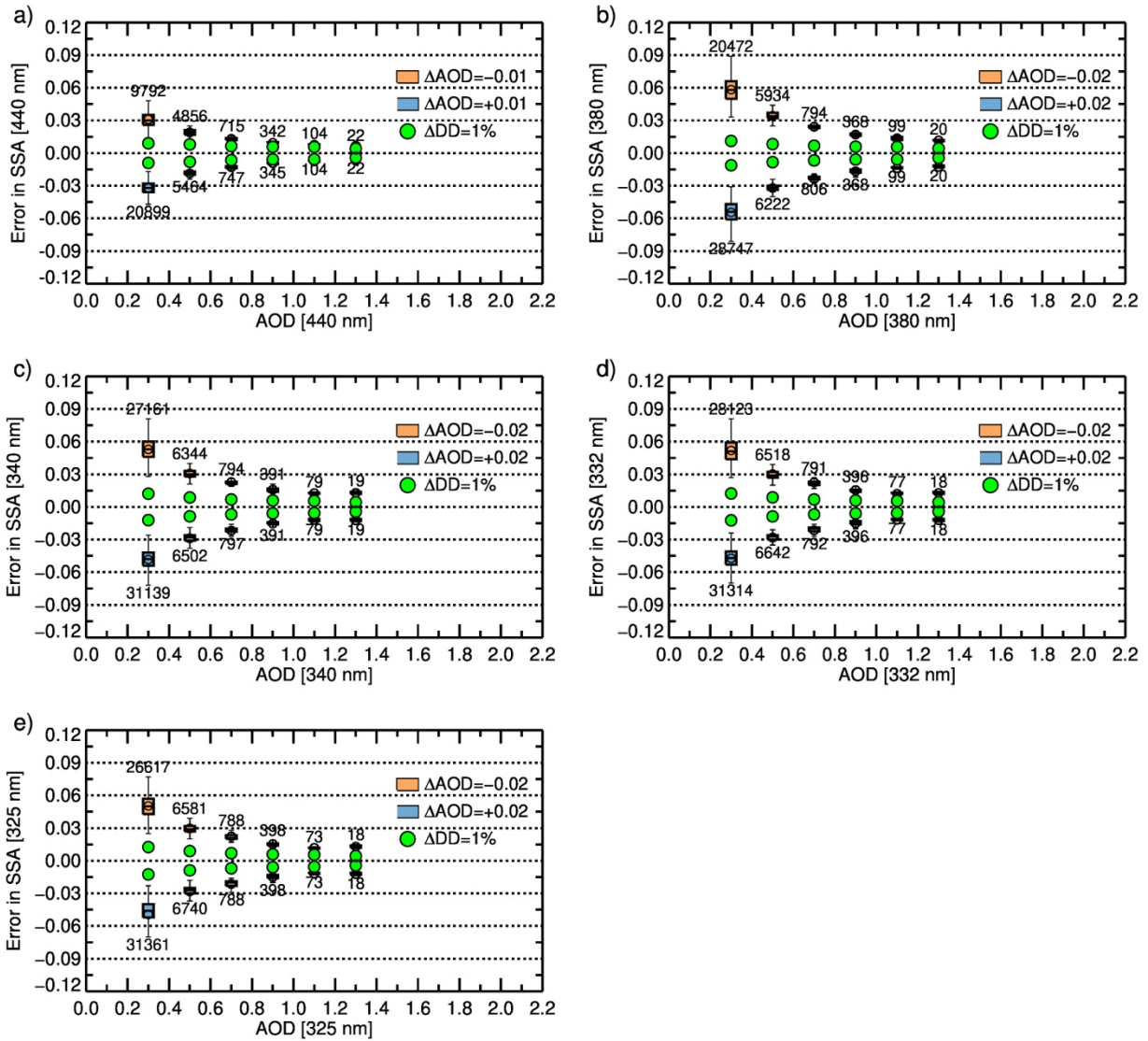
Figure 8 Same as in Figure 7 but for the MFRSR-retrieved spectral SSA.
