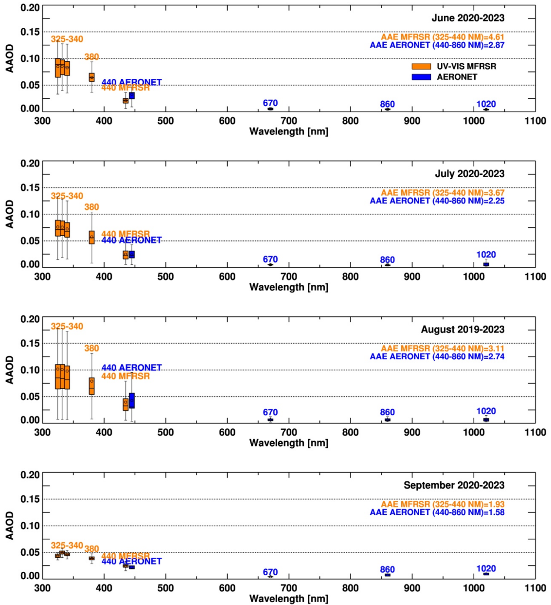
Figure 163. As in Figure 142 but for the retrieved spectral aerosol absorption optical depth (AAOD). The aerosol Absorption Ångström Exponent (AAE) values for UV and VIS-NIR wavelength ranges are also included in each AAOD plot.
