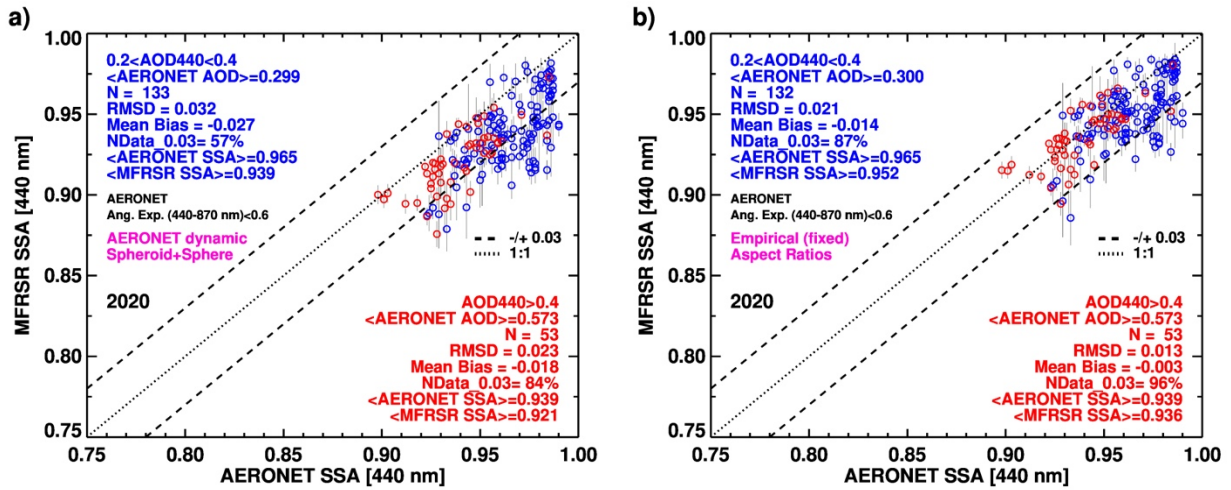
1065 Figure 119. Comparison of MFRSR (y-axis) vs. AERONET (x-axis) SSA at 440 nm for the matchup data collected during 2020 at Izaña site derived assuming a) original aspect ratio distribution representing randomly oriented spheroidal dust suggested in Dubovik et al. (2006) and b) empirically derived aspect ratios adopted in the over-ocean dust aerosol models used for near-UV aerosol algorithm of OMI, EPIC, and TROPOMI sensors. SSA matchup data points in blue and red represent the coincident AOD 440 conditions of 0.2-0.4 and >0.4, respectively. The statistics of the comparison for different AOD conditions are included within the plots. 1070
