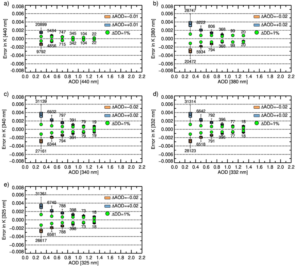
1040 Figure 7 Errors in the MFRSR-retrieved spectral imaginary part of the index (K) resulting from 1) the uncertainties in the AERONET-measured AOD (orange and blue boxes) and 2) 1% change in the MFRSR-measured diffuse-to-direct irradiance ratio (filled green circles). Data represent MFRSR record from 2019-2023. Box-and-whisker elements indicate the interquartile range (25 th -75 th percentiles; boxes) and 1.5 times IQR (whiskers); mean values are shown as open circles and median values as horizontal lines.
