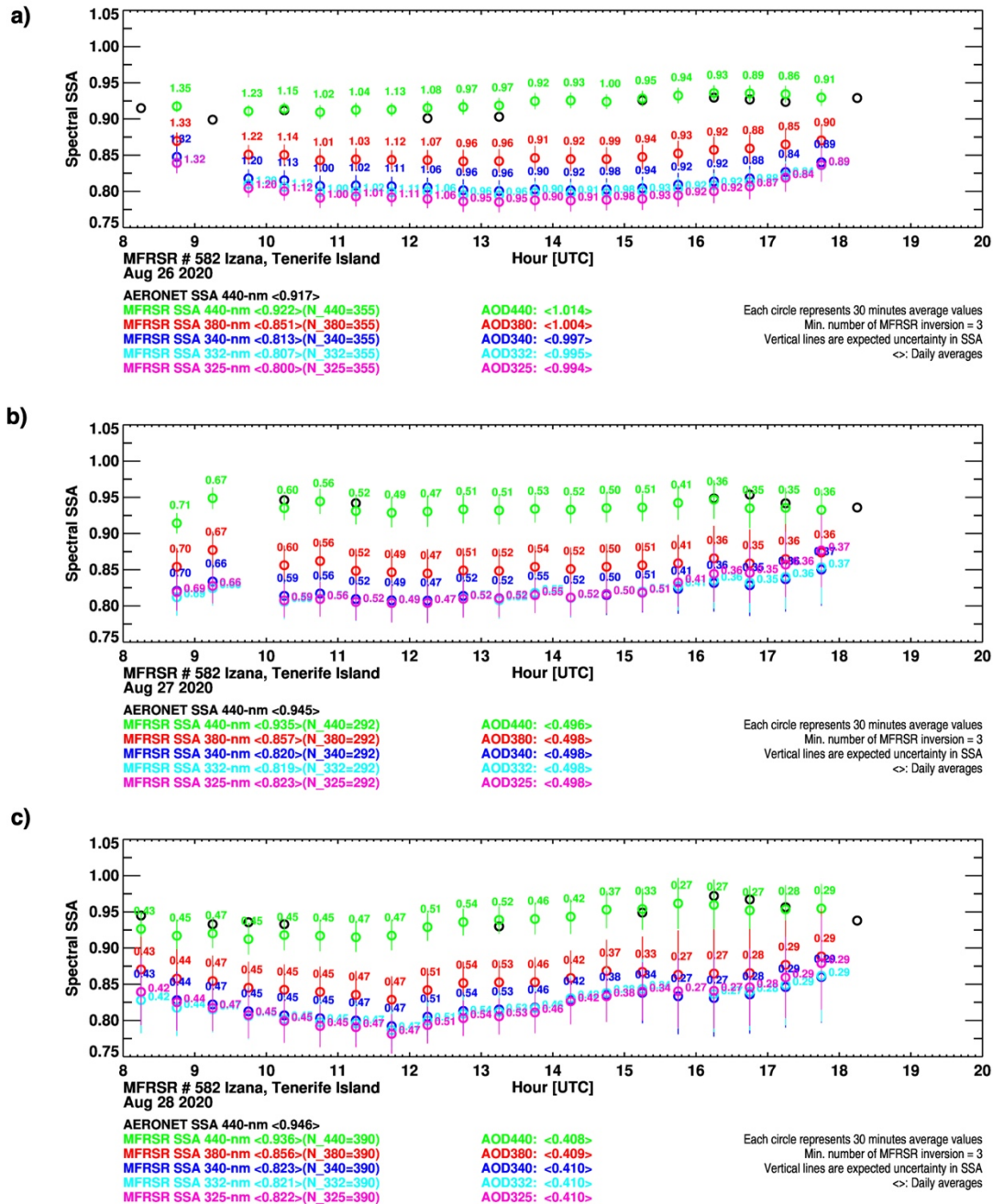
Figure 108. Sub-hourly spectral SSA retrieved from UV-VIS MFRSR observations acquired on August 26, 27, and 28 (a, b, c, respectively) of 2020. Each circle represents 30-minute averaged SSA values with corresponding averaged AOD printed next to it. Vertical lines represent the expected uncertainty in the retrieved SSA, which combinedly accounts for both \pm 0.01 - 0.02 uncertainties in the AERONET-measured AOD and a 1% error in the diffuse to direct irradiance ratio and the standard deviation of 1-minute retrievals within a 30-minute time window. Daily mean values of SSAs and AODs are printed on the bottom of each plot.
