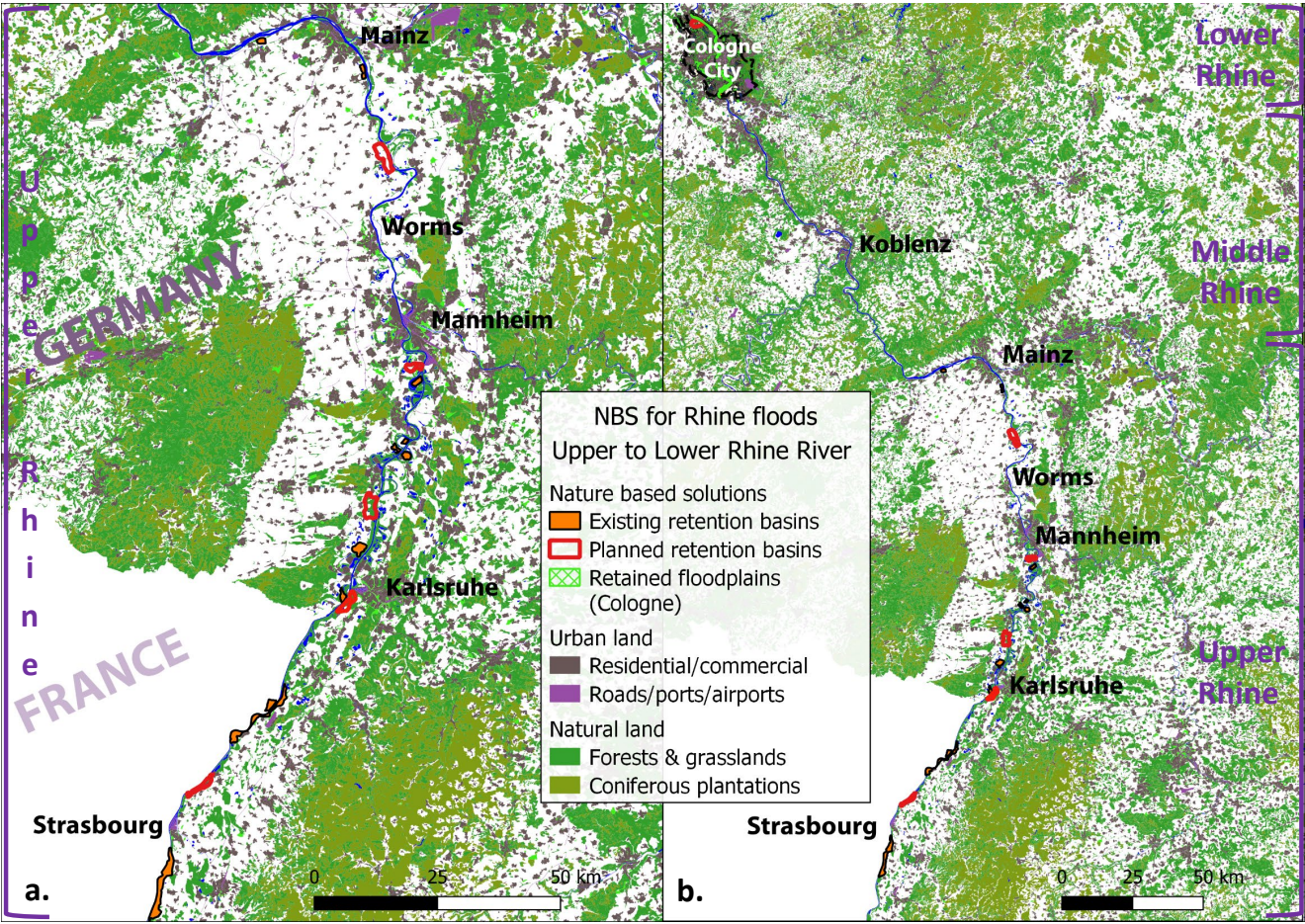
Figure 3: NbS for Rhine floods (left) Strasbourg to Mainz (Upper Rhine) and (right) Strasbourg (Upper Rhine) to Cologne City (Lower Rhine). Data sources: BKG, 2021; ICPR, 2021; OpenGeodata. NRW, n.d. Prepared in QGIS 3.6.2
