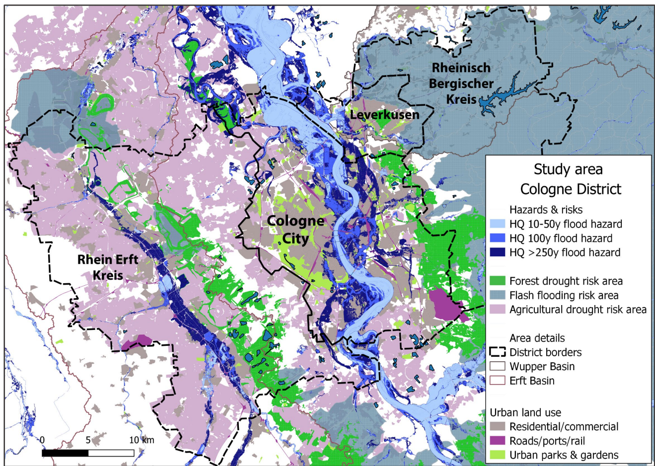
Figure 1: Hydrological hazards and risks occurring in the Cologne District study area Data sources: BKG, 2021; Diva-GIS, n.d.; NASA, 2013; OpenGeodata.NRW, n.d.; Region Köln Bonn, 2019; USGS, 2014. Processed in QGIS 3.6.2.
