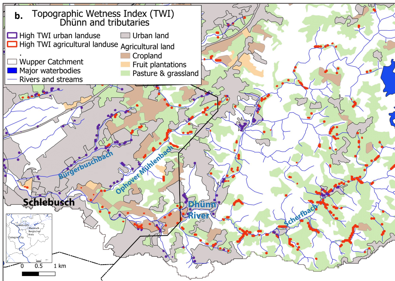
Figure 8: Sites of high TWI on agricultural and urban land affecting (a) Opladen and (b) Schlebusch. Data sources: BKG, 2021; Diva-GIS, n.d.; NASA, 2013; USGS, 2014. Processed in QGIS 3.6.2.
