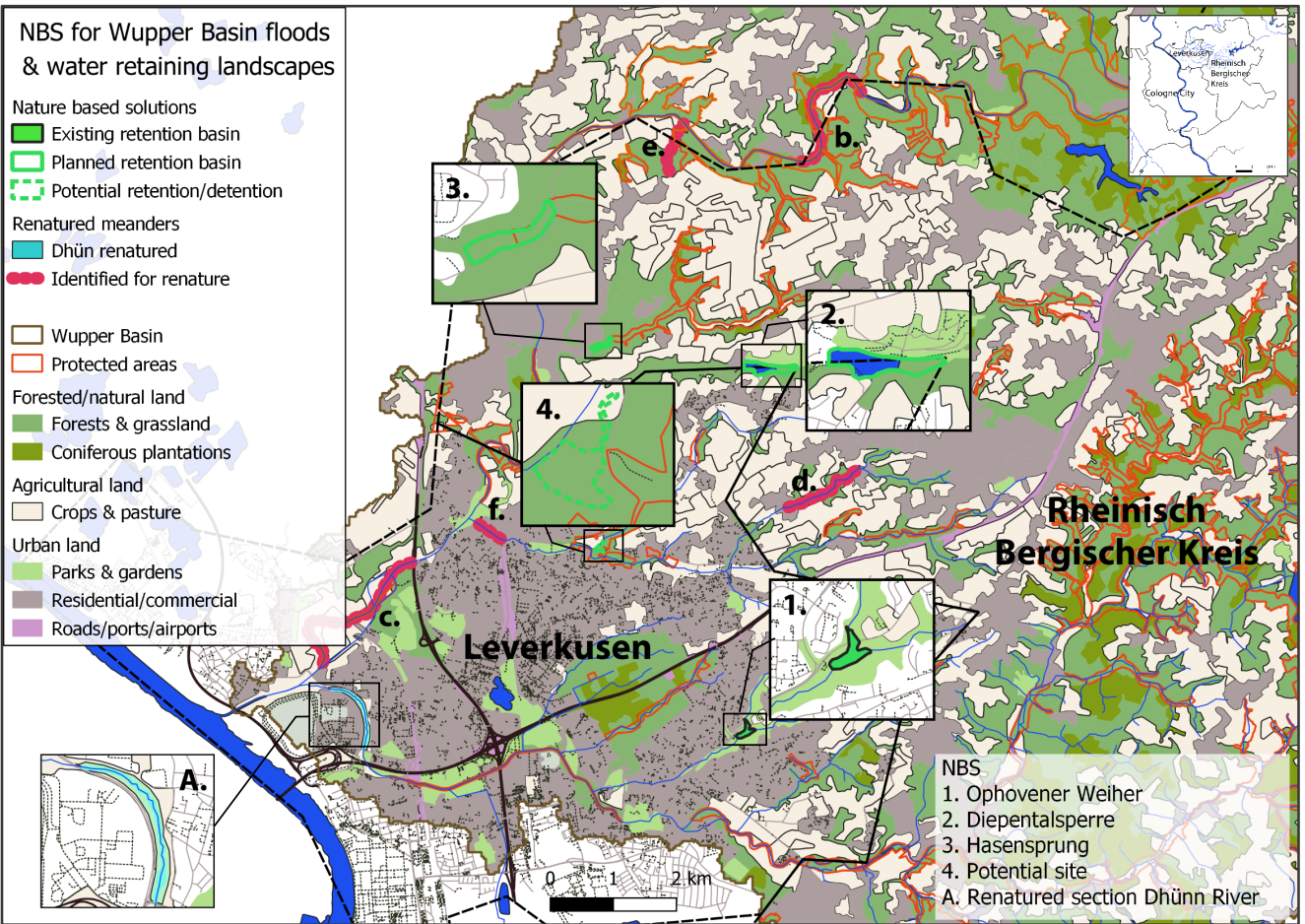
Figure 6: Flood NbS and water retaining landscapes in Leverkusen and Rheinisch-Bergischer Kreis. Data sources: BKG, 2021; Diva-GIS, n.d.; OpenGeodata. NRW, n.d.; © OpenStreetMap contributors 2015. Distributed under the Open Data Commons Open Database License (ODbL) v1.0.; Stadt Leverkusen, 2025; USGS, 2014; Wupperverband, n.da, n.db. Processed in QGIS 3.6.2 Table 4: NbS for river flood mitigation in the Wupper.
