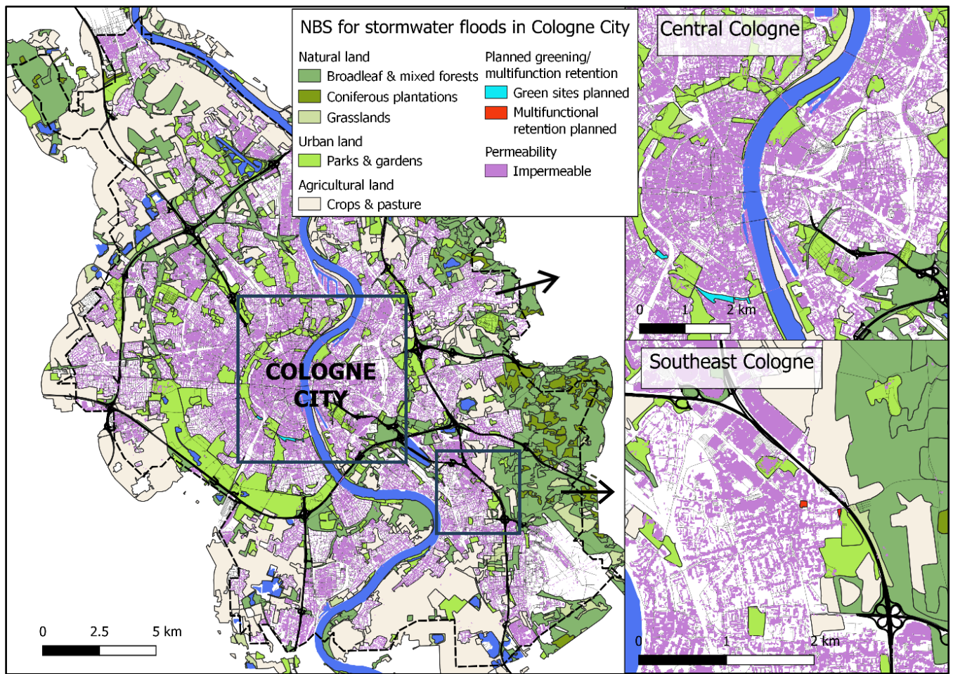
Figure 5: NbS for stormwater floods in Cologne City. Data sources: BKG, 2021; Copernicus,2018; Diva-GIS, n.d.; © OpenStreetMap contributors 2015. Distributed under the Open Data Commons Open Database License (ODbL) v1.0.; StEB, 2025, Stadt Koeln, 2023. Processed in QGIS 3.6.2.
