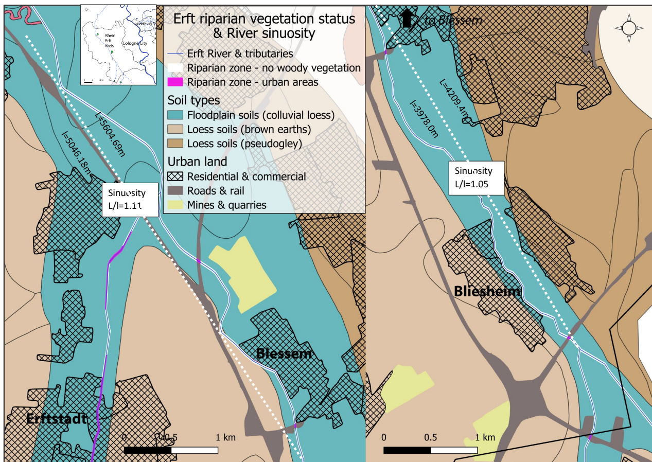
Figure 9: Riparian zones on the Erft devoid of woody vegetation & measure of river sinuosity; Data sources: BKG, 2021; OpenGeodata. NRW, n.d.; © OpenStreetMap contributors 2015. Distributed under the Open Data Commons Open Database License (ODbL) v1.0. Processed in QGIS 3.6.2.
