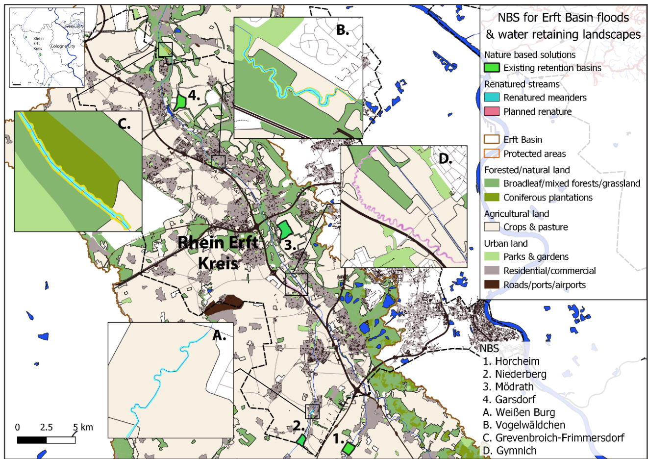
Figure 7: Flood NbS and water retaining landscapes in Rhein-Erft-Kreis. Data sources: BKG, 2021; Diva-GIS, n.d.; Erftverband, n.da, n.db; OpenGeodata. NRW, n.d.; © OpenStreetMap contributors 2015. Distributed under the Open Data Commons Open Database License (ODbL) v1.0.; NASA, 2013. Processed in QGIS 3.6.2
