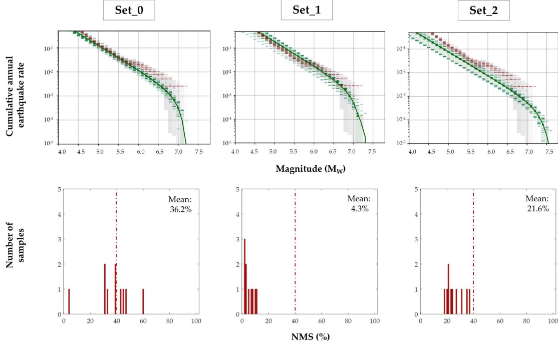
Figure 8. SubArea 1 models: columns show different rupture scenarios. Above: comparison between the modelled MFDs (green) and the seismicity rates from the historical and instrumental regional catalogues within the study area (red). Below: NMS (expressed as a percentage) for each random sample explored in the model.
