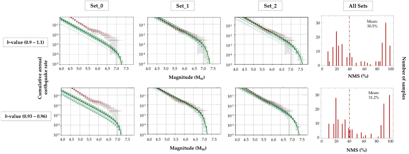
Figure 11. Rows correspond to different b -values. Columns 1–3 show the comparison between modelled MFDs (green) and seismicity rates from the historical and instrumental regional catalogues within the study area (red), for the three rupture scenarios. Column 4 displays the NMS (expressed as a percentage) for each random sample explored under all rupture scenarios.
