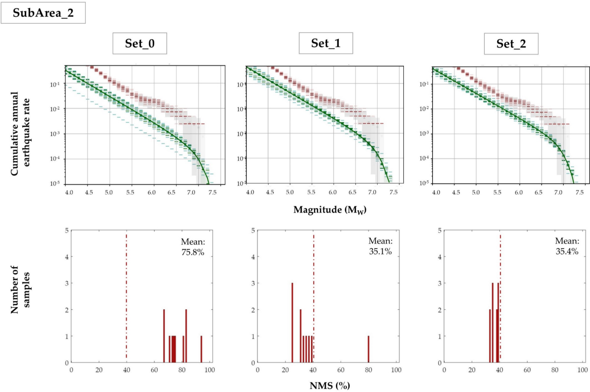
407 408 Figure 9. SubArea 2 models: columns show different rupture scenarios. Above: comparison between the modelled MFDs (green) 409 and the seismicity rates from the historical and instrumental regional catalogues within the study area (red). Below: NMS (expressed 410 as a percentage) for each random sample explored in the model.
