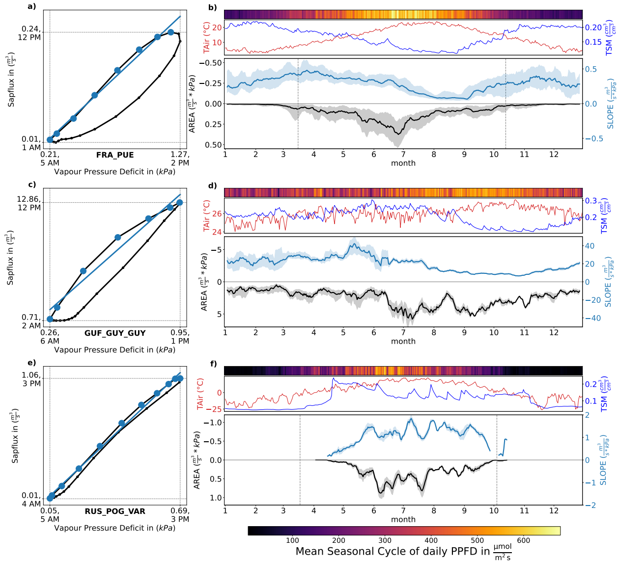
Figure 3. Illustration of metrics derived from diurnal SF-VPD relationships and their variability across seasons. a), c), e): Illustration of the approach used to calculate the two metrics used in this study, based on the mean diurnal cycle of hourly VPD and SF measurements, aggregated over all trees and all days for the whole time span of available data for three selected sites: FRA_PUE, GUF_GUY_GUY, RUS_POG_VAR. The morning slope (SLOPE) is calculated through a linear regression of all hours (colored blue) between minimum VPD and maximum SF, while the area (AREA) is the area enclosed by connecting the data points for all available hourly timestamps. The dashed vertical and horizontal lines indicate the maximum values of the mean seasonal cycles of VPD and SF, and the corresponding average time of the day. b), d), f): Seasonal dynamics of daily values of photosynthetically active radiation (PAR, quantified as daily PPFD), air temperature (TAIR) and top soil moisture (TSM), AREA and SLOPE with interquartile ranges showing the range of the hydrometeorological drivers and the derived metrics per day across years. The vertical lines indicate the selected growing season, i.e. when the day length is higher than 12 hours and temperature > 5^{\circ}C . Absolute values of SLOPE vary according to the magnitude of tree-specific SF rates.
