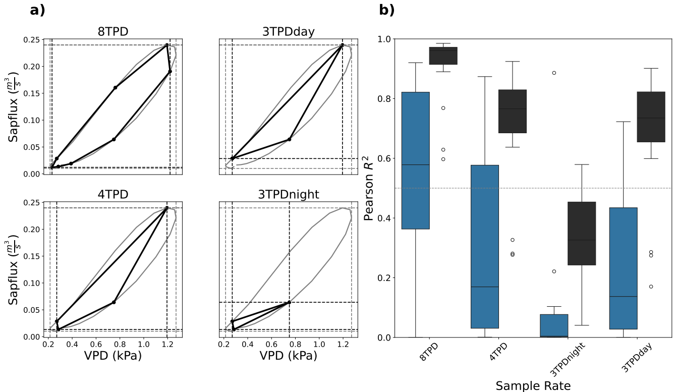
Figure 7. Effect of temporal resolution and sampling times on the two diurnal cycle metrics. a): illustration of the average diurnal cycle for FRA_PUE, estimated based on hourly measurement (solid gray lines), and the corresponding diurnal cycle captured by measurements at different sample rates (bold black lines). The vertices of the curves under lower sampling rates indicate the observations at different sampling rates: 3-hourly, starting at mid-night (8 times per day, 8TPD), 6-hourly, starting at mid-night (4TPD) and 6-hourly with mid-night or noon left out (3TPDday, 3TPDnight). The vertical and horizontal dashed lines indicate the corresponding maximum values of the reference diurnal cycle with hourly time steps (gray) and with coarser temporal sampling (black). b): Boxplots of coefficients of determination ( R^2 ) estimated as the relationship between daily time series of the AREA (black) and SLOPE (blue) metrics at different sample rates (x-axis) and the reference values derived from hourly sampling. The boxplots summarize the variability of R^2 across all sites and reflect how closely the seasonal dynamics of the metrics based on resampled time series track those of the hourly reference across sites.
