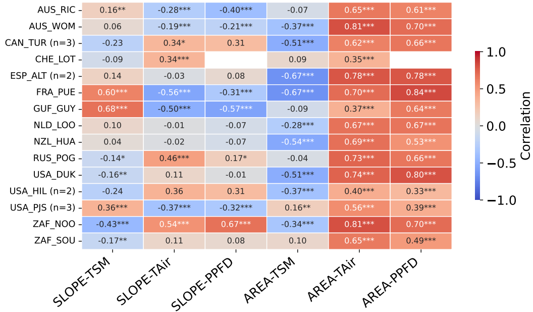
Figure 4. Heatmap of Pearson’s correlation coefficients of the daily values of the SLOPE and AREA metrics and of hydrometeorological drivers (TSM, TAIR and PPF) over the growing season across all studied sites. The number of plots at sites with multiple plots is indicated by n. Asterisks denote statistical significance, with three asterisks indicating p < 0.001 , two indicating p < 0.01 , and one indicating p < 0.05 .
