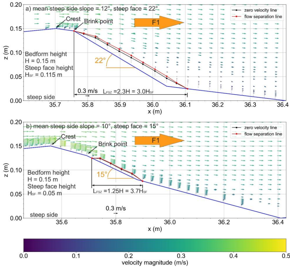
Figure 9. Permanent flow separation zones. a) DUNE1_F1, b) DUNE2_F1.
