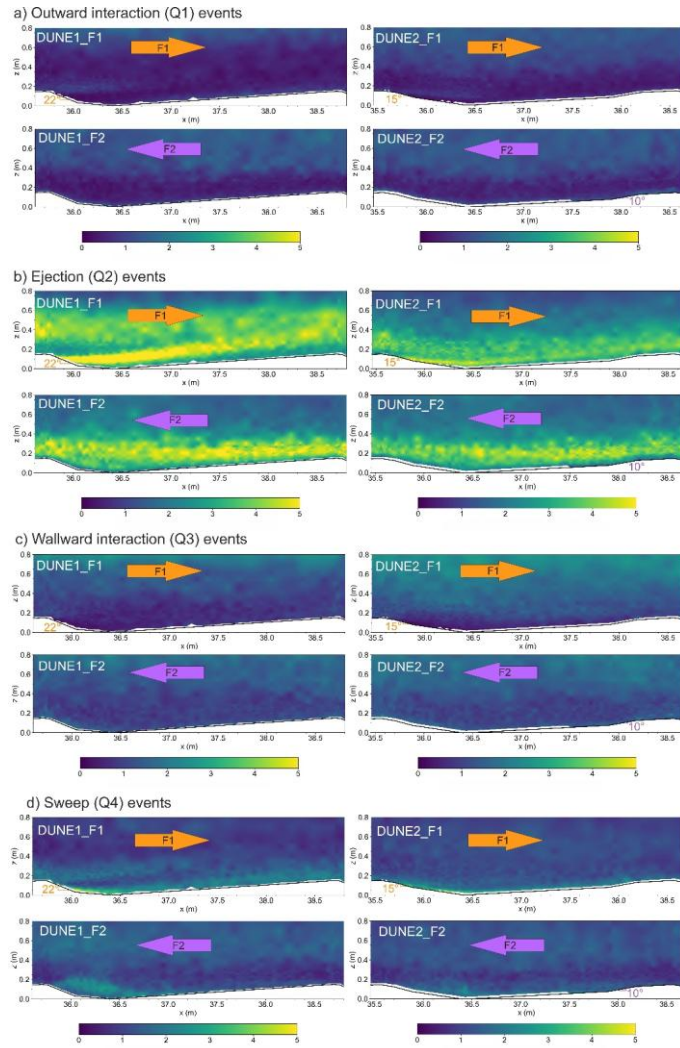
Figure 14. Percentage of observation at each significant quadrant event (%). HS = 2.0. a) Outward interaction event, Q1, b) Ejection event, Q2, c) Wallward interaction event, Q3, d) Sweep event, Q4.
