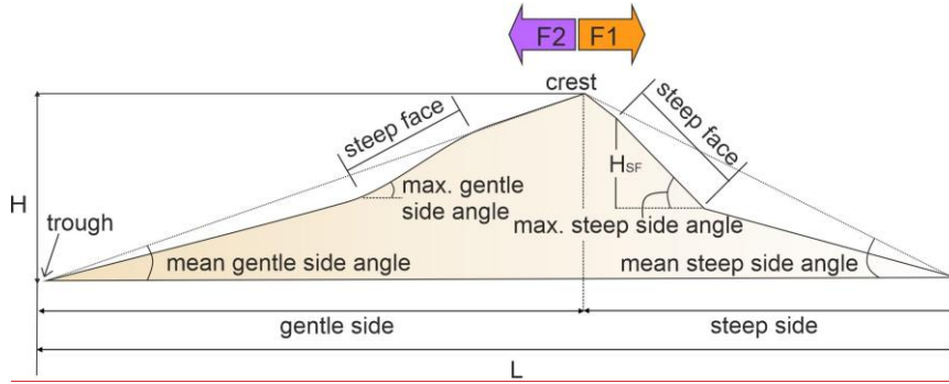
Figure 54. Schematic diagram of tidal dune morphology. H is the bedform height, H_{SF} is the steep face height, L is the bedform length, F1 refers to the flow that is aligned with the dune asymmetry (i.e., the flow is directed from the gentle stoss to the steep lee slope) and F2 refers to the flow that is opposing the dune asymmetry (i.e., the flow is directed from the steep stoss to the gentle lee slope).
