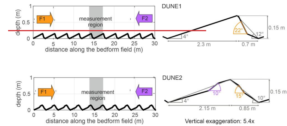
Figure 5. Laboratory tidal dunes and experimental flume setup.
