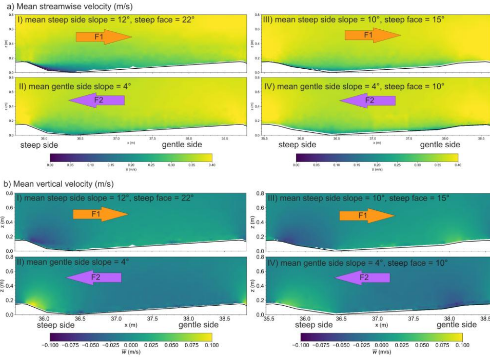
Figure 8. Time-averaged flow fields. I) DUNE1_F1, II) DUNE1_F2, III) DUNE2_F1, IV) DUNE2_F2.
