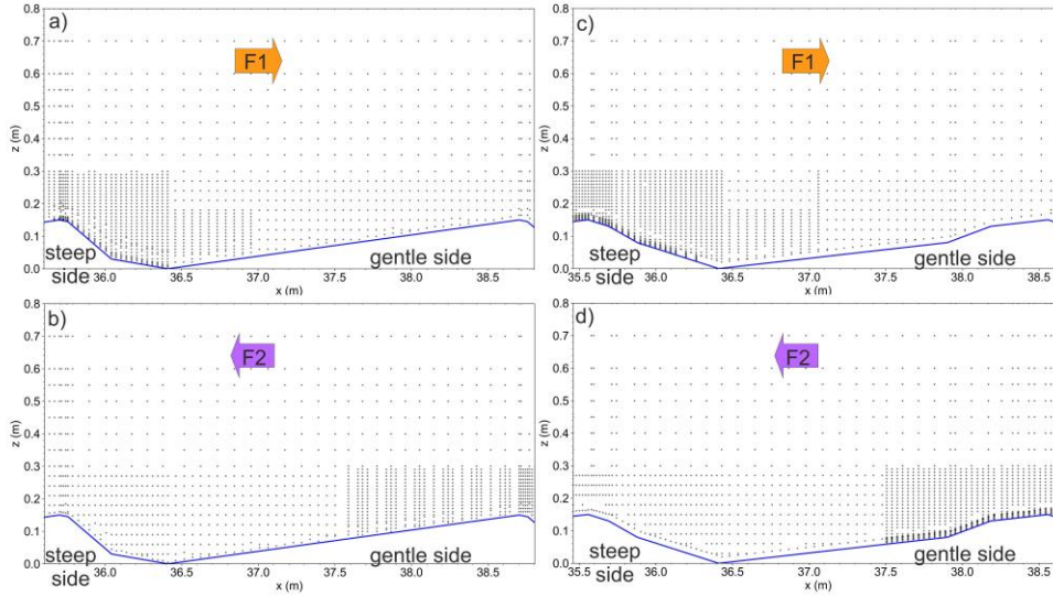
Figure 6. ADV point measurement layout. a) DUNE1_F1, b) DUNE1_F2, c) DUNE2_F1, d) DUNE2_F2. F1: flow aligned with dune asymmetry; F2: flow opposed to dune asymmetry.
