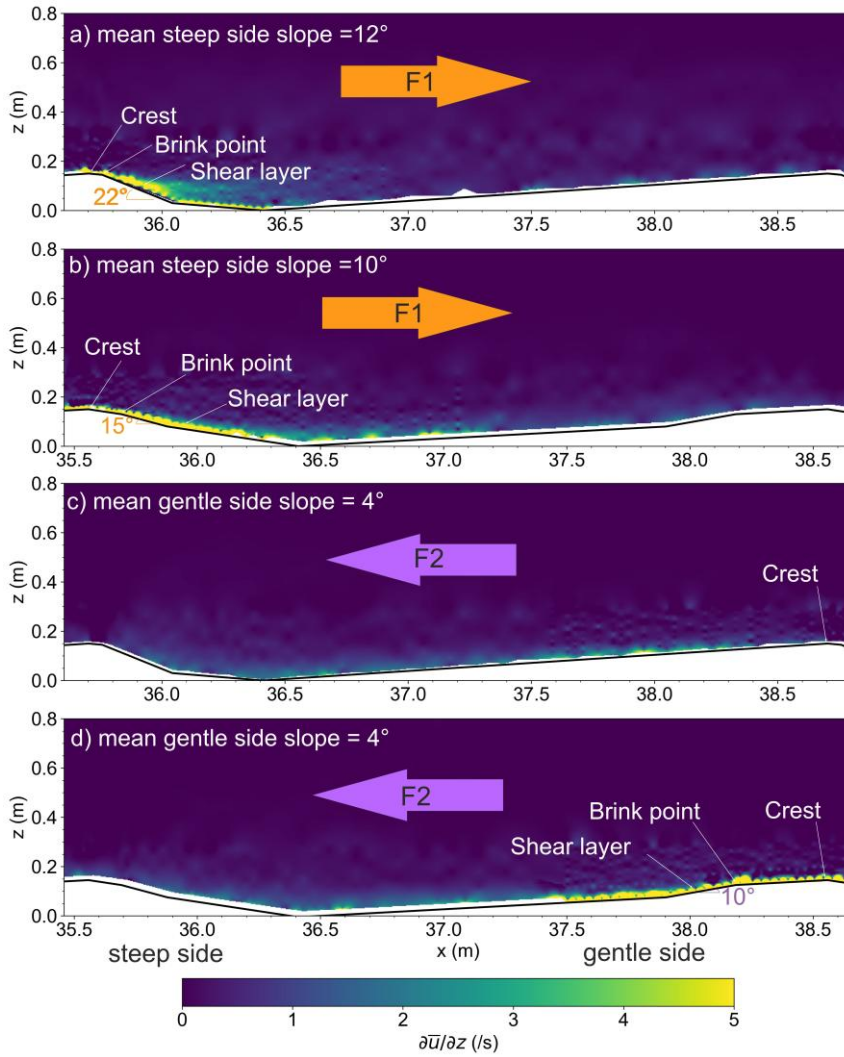
345 Figure 11. Vertical gradient of time-averaged horizontal velocity, \partial \bar{u} / \partial z (1/s). a) DUNE1_F1, b) DUNE2_F1, c) DUNE1_F2, d) DUNE2_F2.
