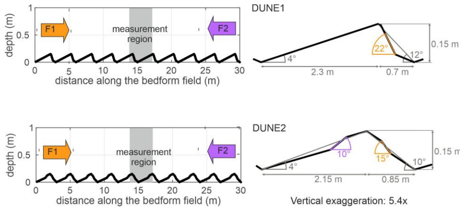
Figure 4. Laboratory tidal dunes and experimental flume setup.
