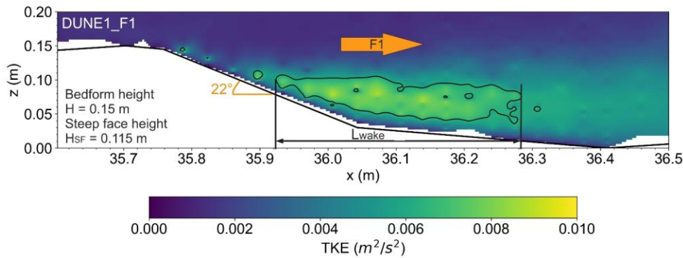
Figure 16. Turbulent wake (70%TKE max isolines) over DUNE1_F1.
