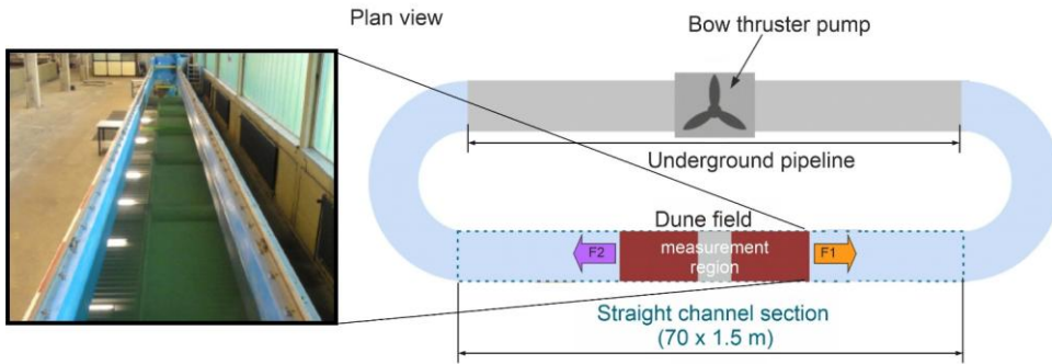
Figure 3: Schematic diagram of the recirculating flume.
