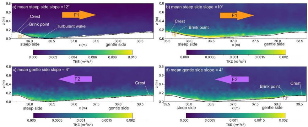
Figure 12. Turbulent kinetic energy, TKE (m 2 /s 2 ). a) DUNE1_F1, b) DUNE2_F1, c) DUNE1_F2, d) DUNE2_F2. Note different scale used for Fig. 12a.
