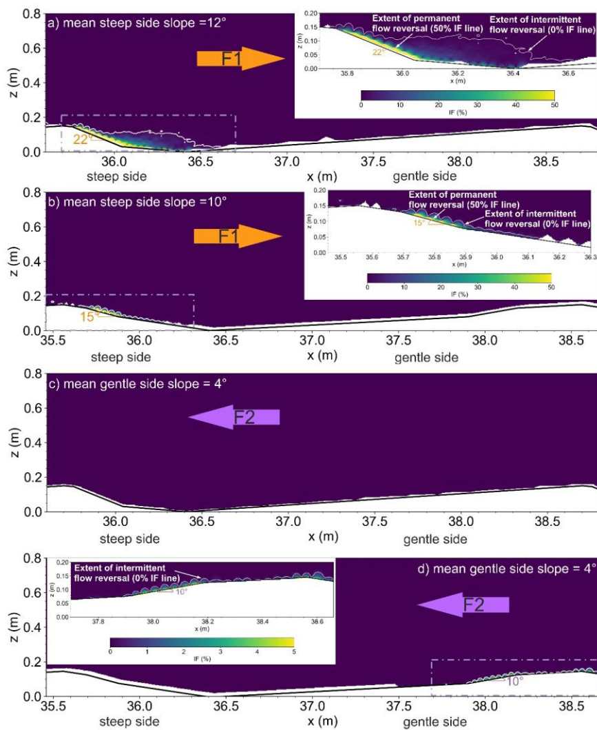
Figure 10. Intermittency factor, IF (%). a) DUNE1_F1, b) DUNE2_F1, c) DUNE1_F2, d) DUNE2_F2. Note different scale used for Fig. 10d.
