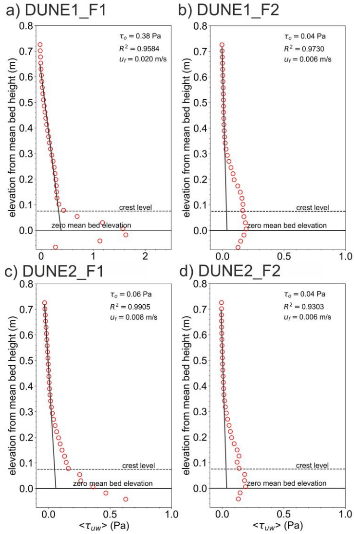
Figure 13. Spatially-averaged Reynolds stress profiles, \langle \tau_{uw} \rangle (Pa). Note different scale for Fig. 13a.
