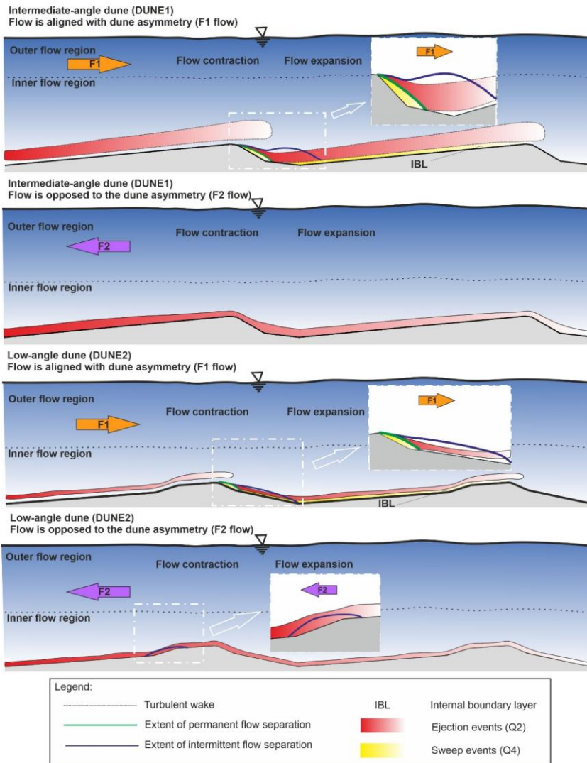
Figure 15. Conceptual diagram of flow and turbulence dynamics over intermediate- and low-angle tidal dunes.
