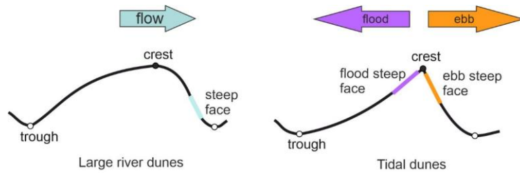
Figure 2: Schematic representations of river and tidal dunes.
