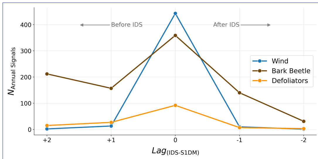
Figure 7. Temporal relationship between disturbance detection by S1CD-S1DM and IDS. The x-axis represents the temporal yearly agreement with IDS - S1CD-S1DM . Negative values indicate that IDS recorded the disturbance before S1CD detected it. The y-axis shows the count of events corresponding to each year's lag, with different disturbance types represented by distinct colored lines. We focuses focus on the single S1DM timestamp closest to the IDS year for each event. We calculate the temporal lag by subtracting the S1DM detection year from the IDS year. Negative values indicate that S1DM detection occurred after IDS, while positive values indicate earlier radar detection.
