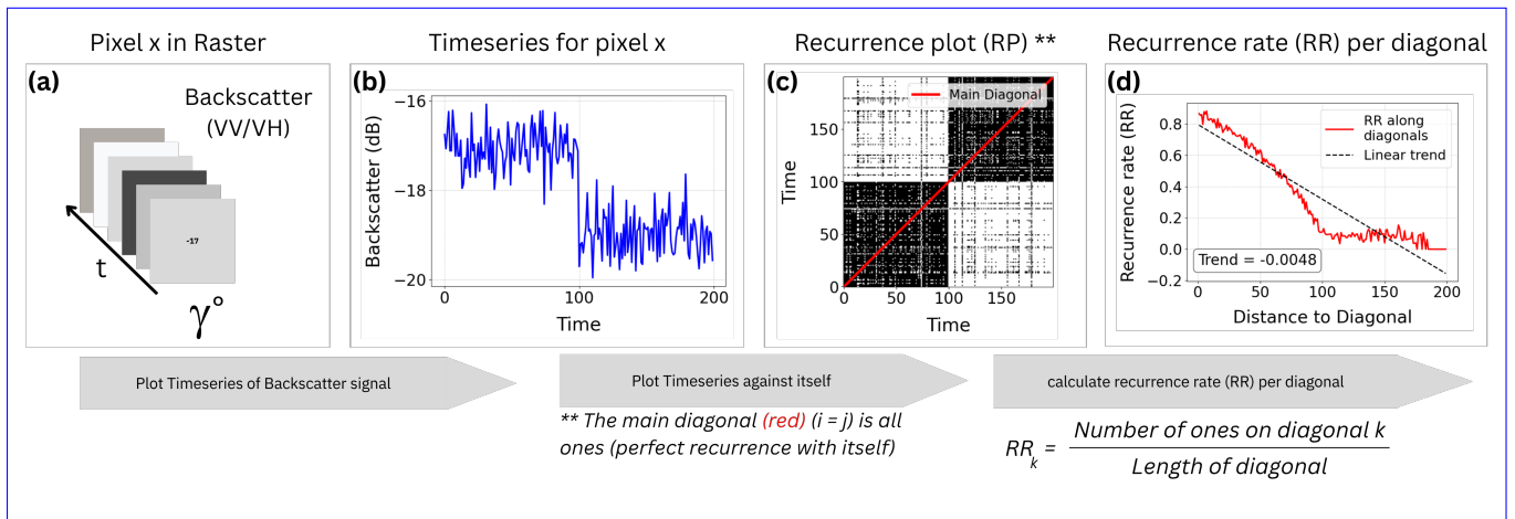
Figure A2. Schematic representation of recurrence analysis for a Gamma backscatter pixel. (a) Singular Pixel of one Sentinel-1 Raster Tile (b) Time series of the pixel showing a sudden change (“break”) in backscatter values. (c) Recurrence plot (RP) highlighting times when the signal revisits similar states; the main diagonal is shown in red. (d) Recurrence rate ( RR_i ) computed along off-diagonals of the RP, with a linear trend (dashed line) indicating the rate of drift in the system. The slope of the trend quantifies whether the process is stationary or drifting over time.
