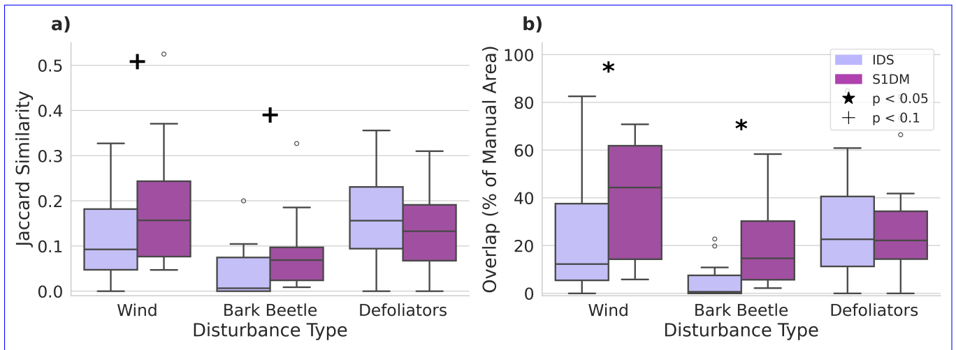
Figure 9. Comparison of agreement between IDS and S1DM disturbance maps with manually delineated reference polygons. Panel (a) shows the Jaccard similarity, and panel (b) shows area overlap (in percentage), both displayed as box plots. Statistical significance from a one-sided t-test Wilcoxon rank test is indicated by a black star for p < 0.05 and a black cross for p < 0.1 .
