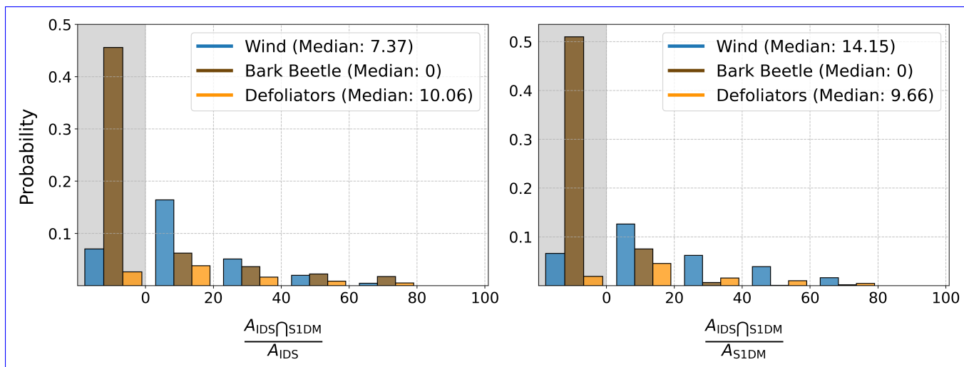
Figure 5. Probability of (a) IDS polygons being covered by S1DM, and (b) S1DM polygons overlapping with IDS, for each disturbance type. Disturbance types are color-coded as follows: Wind-wind (blue), Bark-Beetle bark beetles (brown), and Defoliators-defoliators (yellow). Median probabilities for each disturbance type are indicated in parentheses in the legend.
