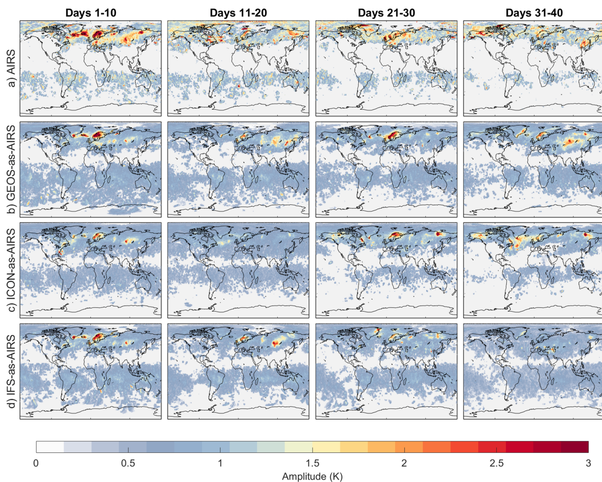
Figure 8. GW amplitudes (measured in K) 10-day conditional mean (only pixels identified as waves are considered). First row AIRS observations, second row GEOS sampled as AIRS, third row ICON sampled as AIRS and bottom row IFS sampled as AIRS. Columns show average 10-day time periods since model initialisation on the 20th January 2020. Data is shown at 33 km altitude. Data is only averaged for instances where a wave is detected.
