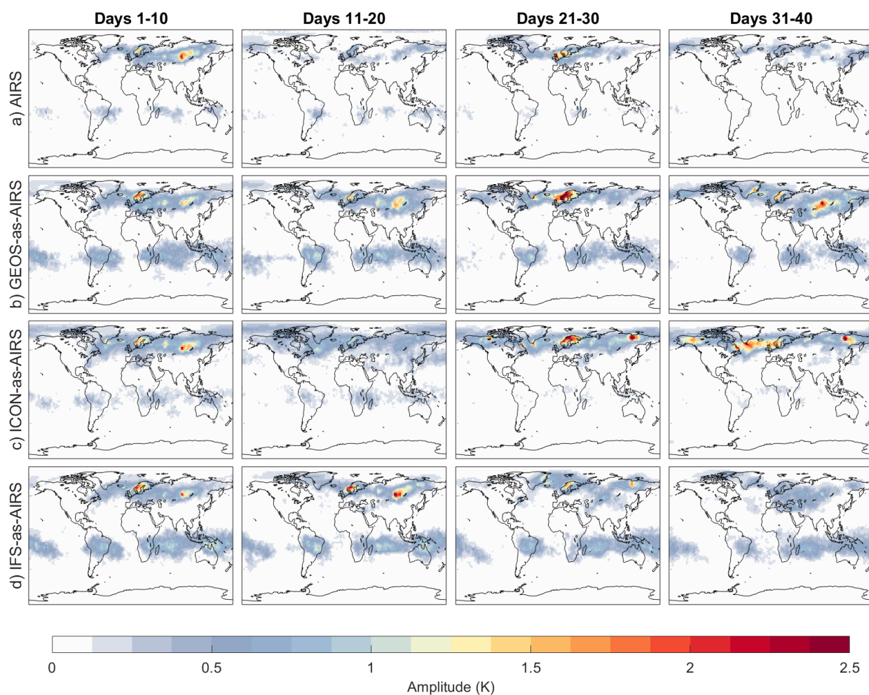
Figure 9. GW amplitudes (measured in K) 10-day unconditional mean (no wave equals a wave with 0 K amplitude). First row AIRS observations, second row GEOS sampled as AIRS, third row ICON sampled as AIRS and bottom row IFS sampled as AIRS. Columns show average 10-day time periods since model initialisation on the 20th January 2020. Data is shown at 33 km altitude. Data is only averaged for instances where a wave is detected.
