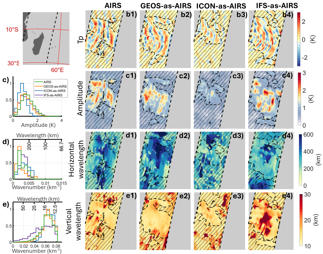
Figure 5. Same as Figure 4 but for an overpass over Madagascar on the 21st January 2020. Panel (a) shows the location of the overpass on the map, dashed black lines indicate the granule edge. Panel (b1-4) shows the temperature perturbations (Tp) measured in K, (c1-4) the amplitude in K, (d1-4) horizontal wavelength in km and (e1-4) vertical wavelength in km respectively. 1) Denotes AIRS observations, 2) GEOS sampled as AIRS, 3) ICON sampled as AIRS and 4) IFS sampled as AIRS. The black dashed border outlines the wave region and hatching covers regions not identified as a wave. Panels (c), (d) and (e) show histograms for the unhatched region for amplitude, horizontal and vertical wavelength respectively.
