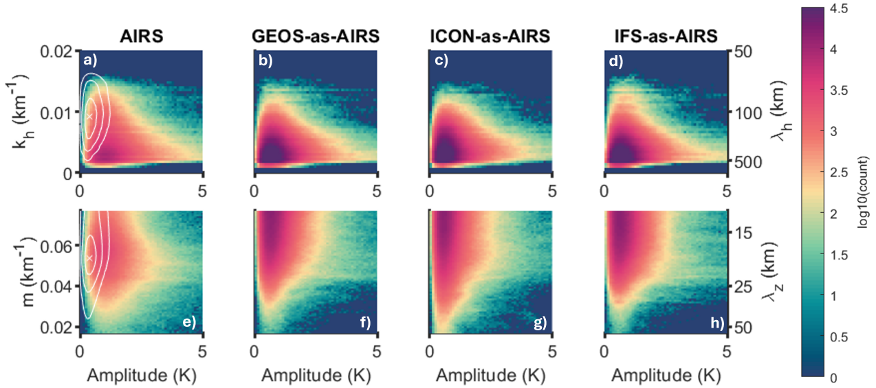
Figure 12. Two-dimensional histograms for (a-d) horizontal wavenumber against amplitude for the first 10 days of the model runs, (e-h) vertical wavenumber against amplitude. Panels (a, e) are AIRS observed GWs, (b, f) GEOS sampled as AIRS, (c, g) ICON sampled as AIRS and (d, h) IFS sampled as AIRS. All data is shown from 33 km altitude. Note the log10 scale on the histogram counts. White contours on the AIRS panels indicate the wavenumber-amplitude properties of areas where there is no wave present (this method is described in further detail in the text). The white cross indicates the most frequent GW properties with contours at 1/2, 1/10 and 1/100th of this maximum.
