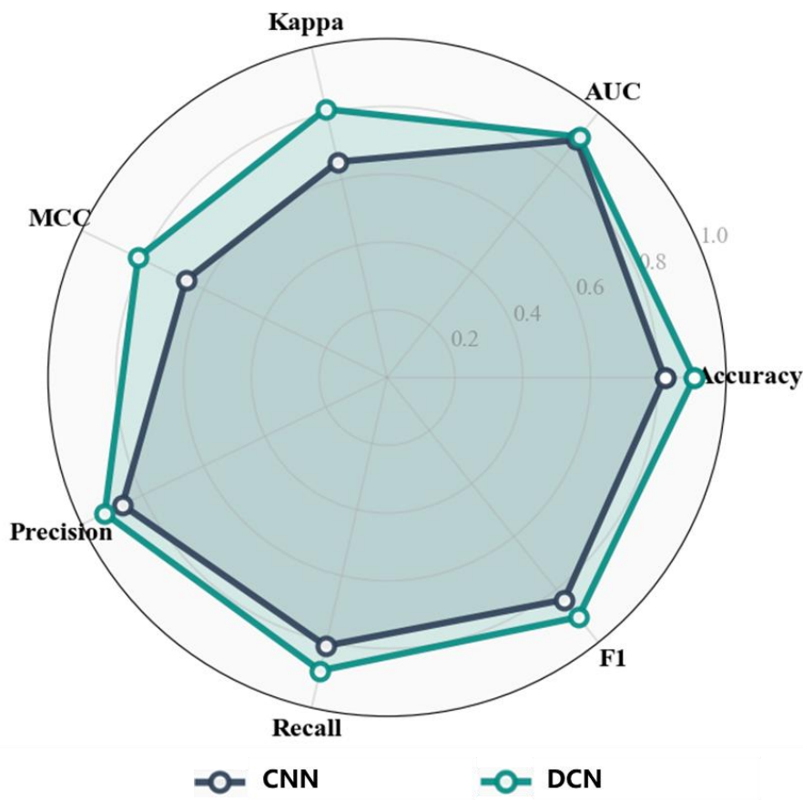
Figure 13: Evaluation of model performance between CNN and DCN in Accuracy, Precision, Recall, F1-score, AUC, Kappa, and MCC.
