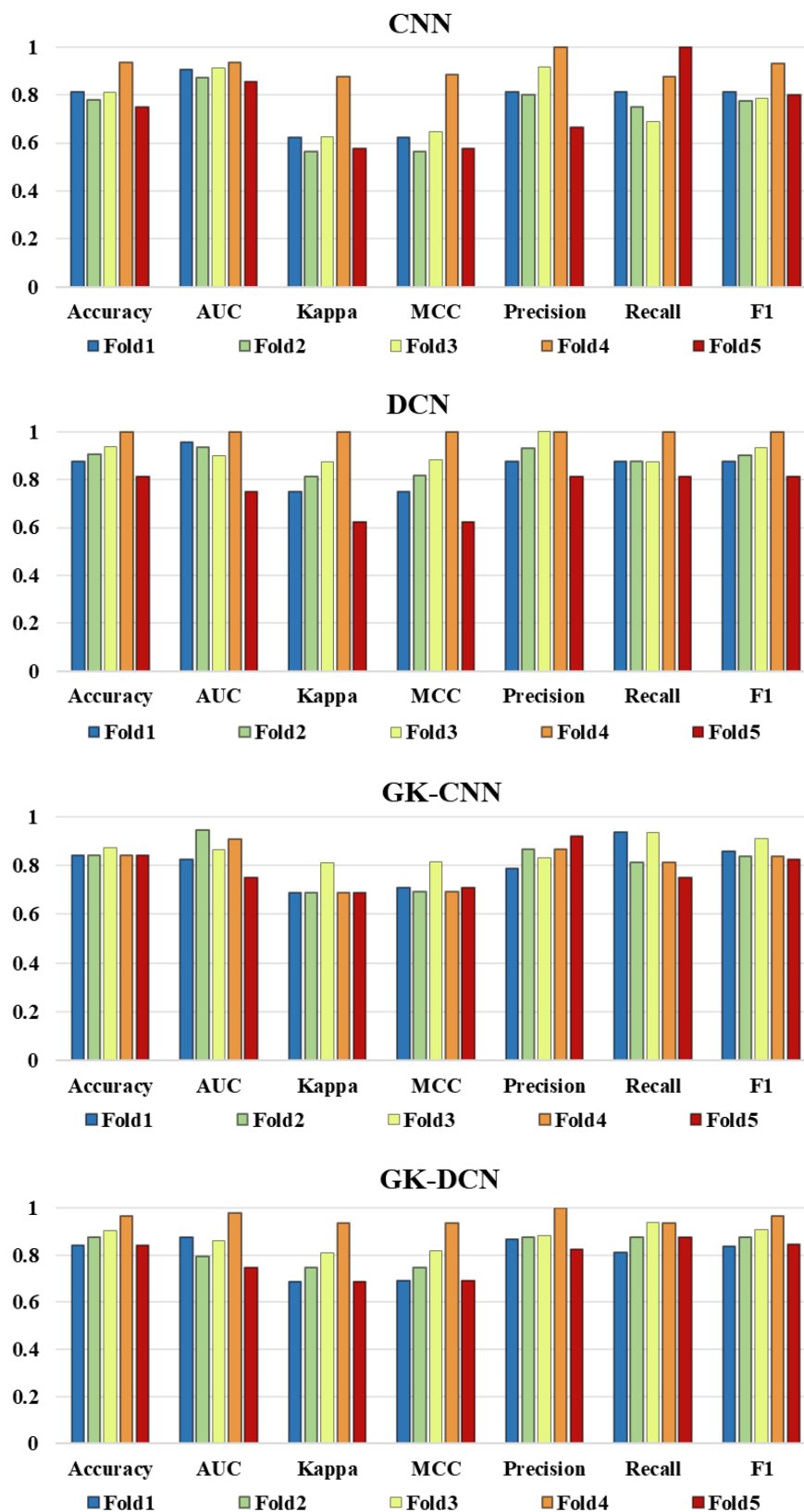
Figure 12: Results of five-fold cross-validation for models CNN, DCN, GK-CNN, and GK-DCN across different performance metrics.
