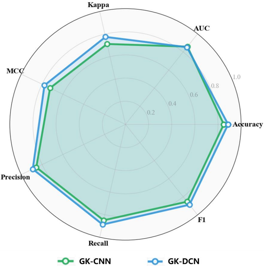
Figure 14: Evaluation of model performance between GK-CNN and GK-DCN in Accuracy, Precision, Recall, F1-score, AUC, Kappa, and MCC.
