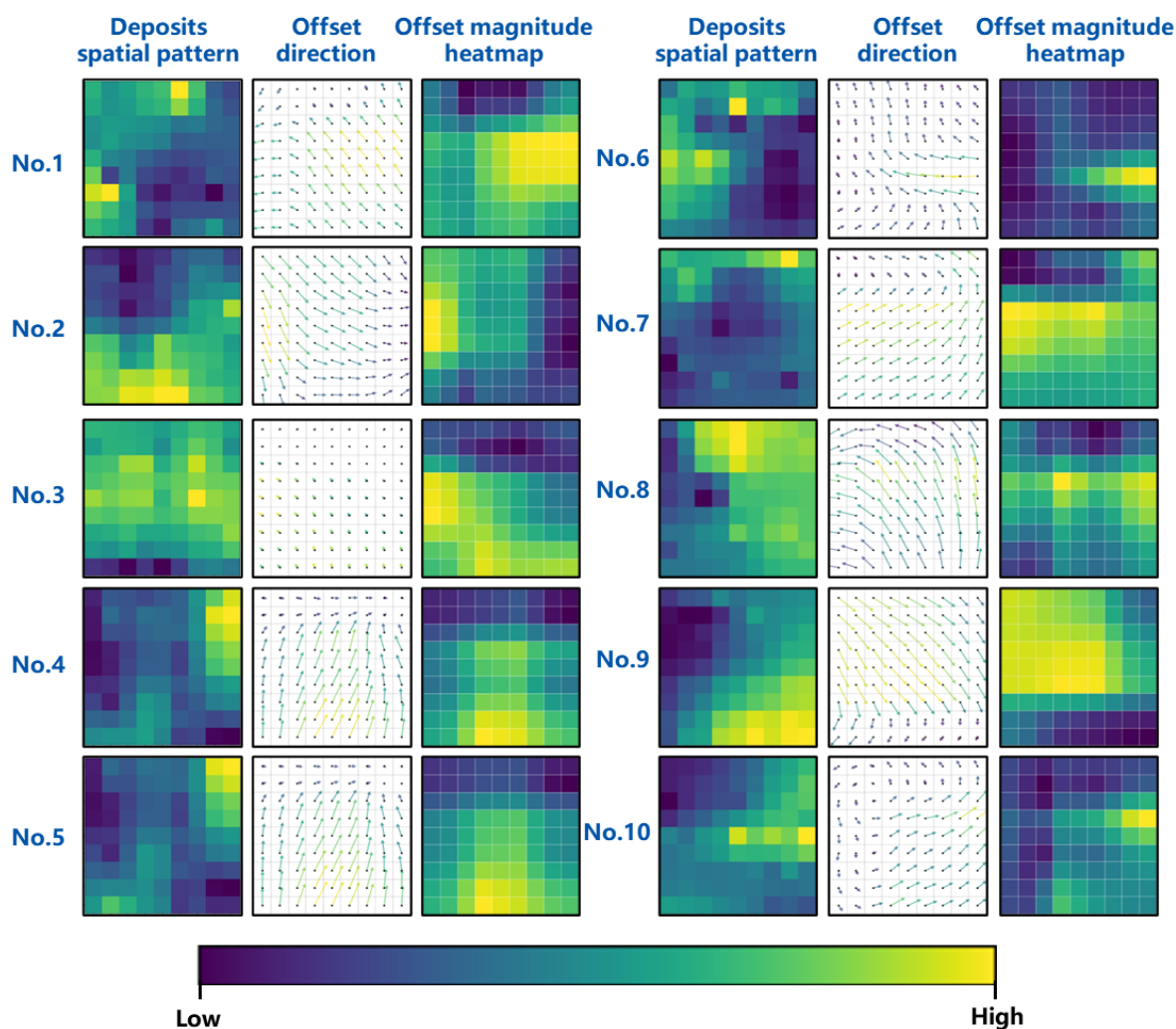
Figure 10: Comparison of offset direction and magnitude maps obtained by GK-CNN and GK-DCN with the geochemical patterns of ten mineral deposits clipped from PC2 score maps in this study. The yellow in the maps represent high concentration and high offset magnitude. The longer the arrow in the offset direction maps, the greater the offset.
