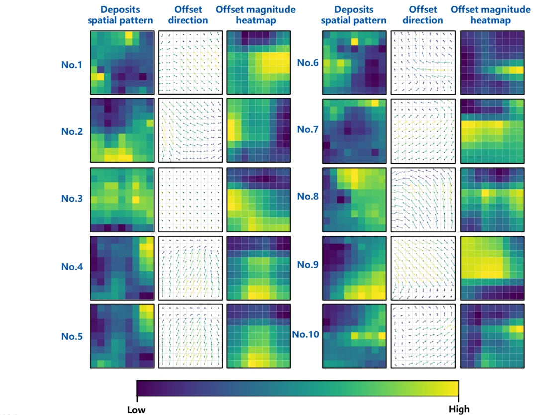
Figure 10: Comparison of offset direction and magnitude maps obtained by GK_CNN and GK_DCN with the geochemical
