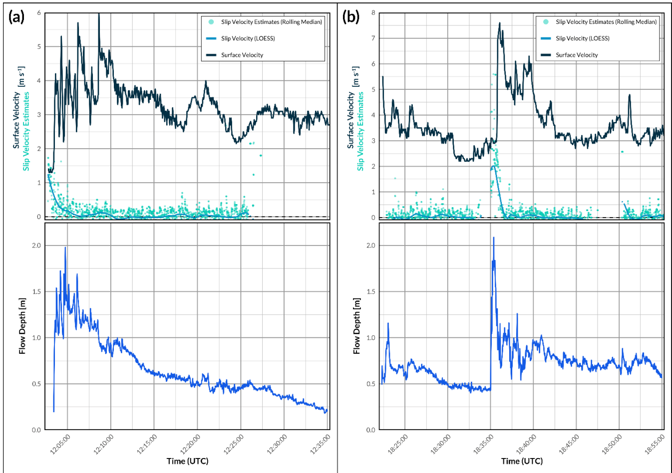
90 Figure 2: Tendency of basal slip for two debris-flow events at Lattenbach: (a) 15 June 2025 and (b) 30 June 2025. In the respective upper plots, the turquoise scatter represents rolling median values of cross-correlated velocity estimates from three sensor pair combinations, the light blue line represents a trend of these rolling median values (LOESS), and the gray-blue line shows the individual measured surface velocity. The blue line in the respective lower plots represents the fluctuation of flow depth from a laser gauge.
