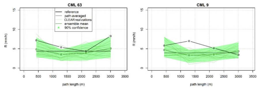
395 Figure 10: CLEAR disaggregation of rain rates during one time step at 19:45 UTC demonstrated on real data from two CMLs of similar path length.
