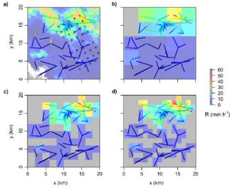
Figure A1: a) Reference rainfall field and CMLs with color-coded path-averaged rain rates. The positioning of the points used to sample rain rates for SC rule is illustrated for CML 33 and marked with crosses. b-d) Gridded rainfall used to evaluate spatial coherence rule when splitting CML segments at successive levels (1 st , 2 nd , 3 rd ) of the cascade. Grey color is used to indicate cells with not available rain rate values.
