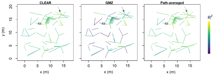
Figure 7: R-squared between reference and disaggregated rain rates evaluated over all time steps separately for each CML. Left: CLEAR ensemble mean. Middle: GMZ. Right: GMZ path-averaged rain rates .
