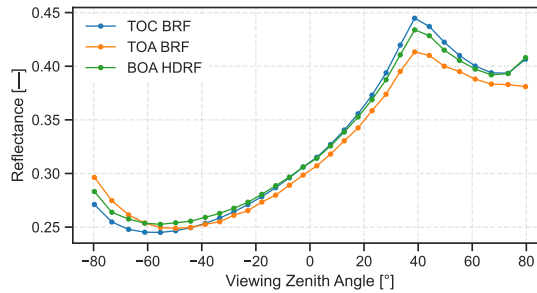
Figure 13. The TOA BRF (surface and atmosphere, sensor at satellite altitude), BOA HDRF (surface and TOC-atmosphere, sensor at top of canopy altitude) and TOC BRF (surface only, sensor at top of canopy altitude) for a retro-reflective RPV surface illuminated with a solar zenith angle of 38^\circ . In the scenarios that include an atmosphere, a clear-sky AFGL 1986 (US Standard) profile is used. The values shown are computed using Eradiate in monochromatic at 550 nm.
