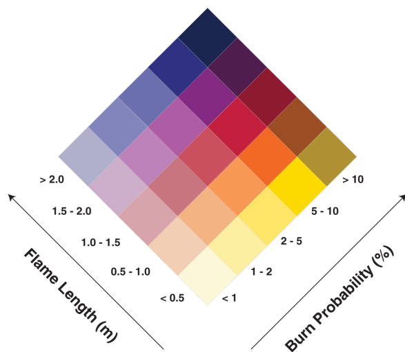
Figure 4: The nine wildfire hazard rasters for three different levels of forest fire danger (WBI) and three different fire durations. National borders and the River Elbe are also overimposed. Each scenario simultaneously represents the flame length (FL) and burn probability (BP) classes. The legend's colours were created using the HSB (Hue Saturation Brightness) Colour Model. Hue was varied to visualise FL ranging from yellow (low flames) to dark blue (high flames). Saturation was varied to represent BP from light colours (low burn probability) to dark colours (high burn probability).
