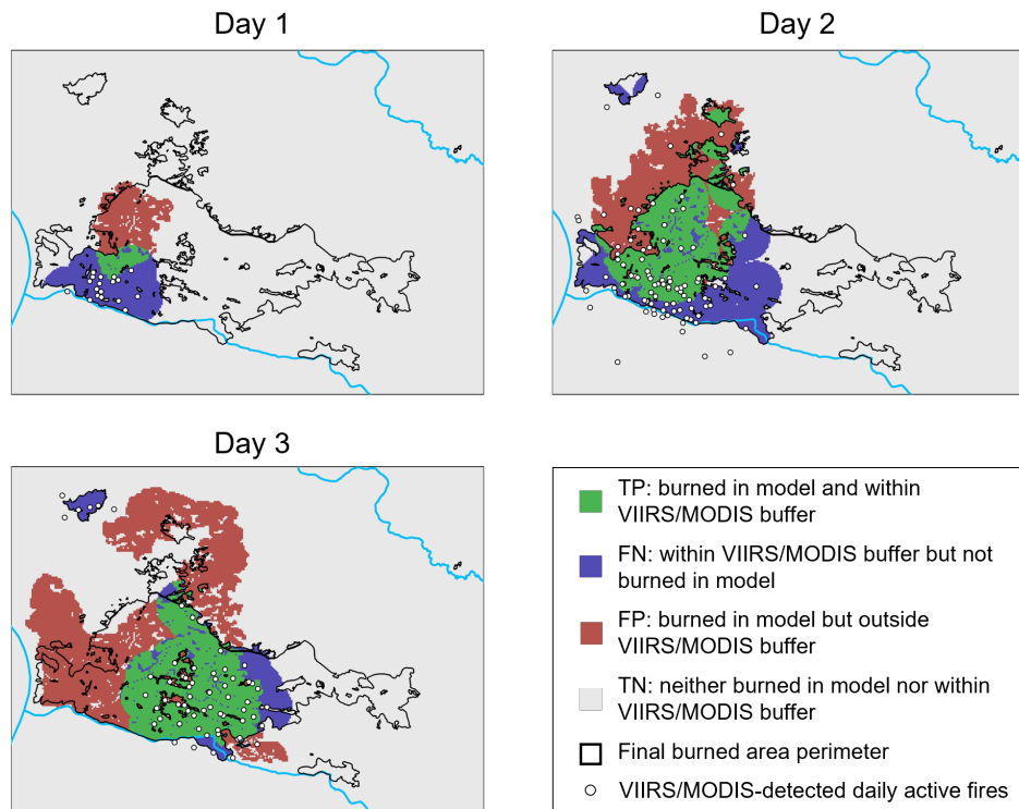
480 Figure 8: Comparison of three daily FlamMap simulations with satellite-detected fires (TP true positive, FN false negative, FP false positive, TN true negative).
