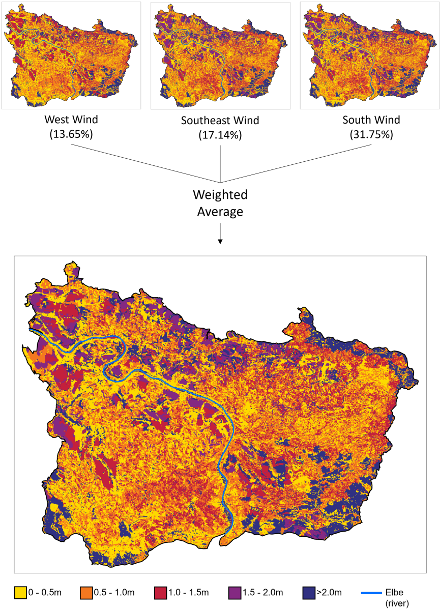
700 Figure D1. Workflow for derivation of flame length raster for scenario WBI = 5 and duration = 3 days
