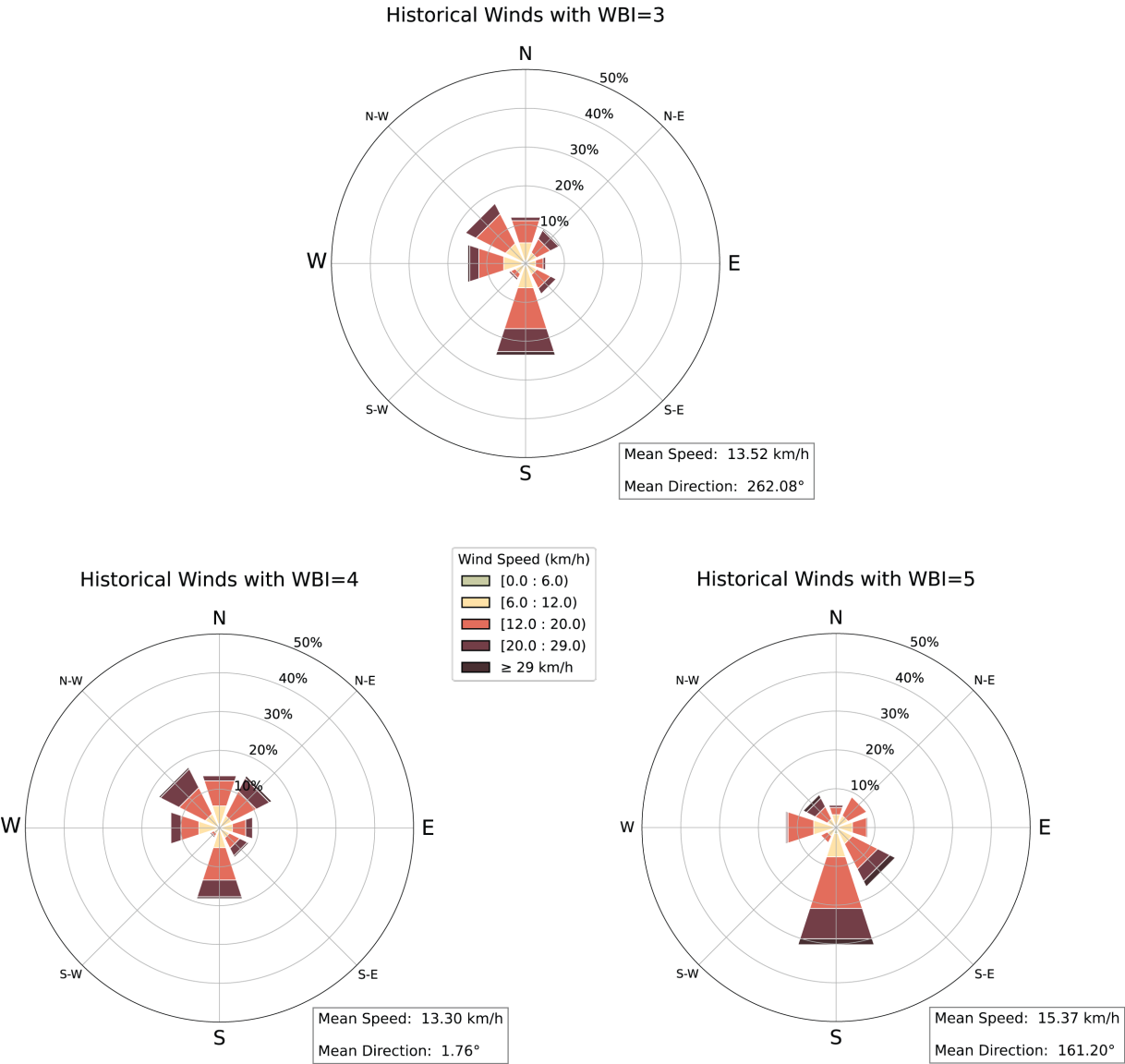
695 Figure C1: Wind roses for winds that occurred on days with WBI = 3, 4 and 5 in Bad Schandau from 15.02.2009 until 12.08.2022.
