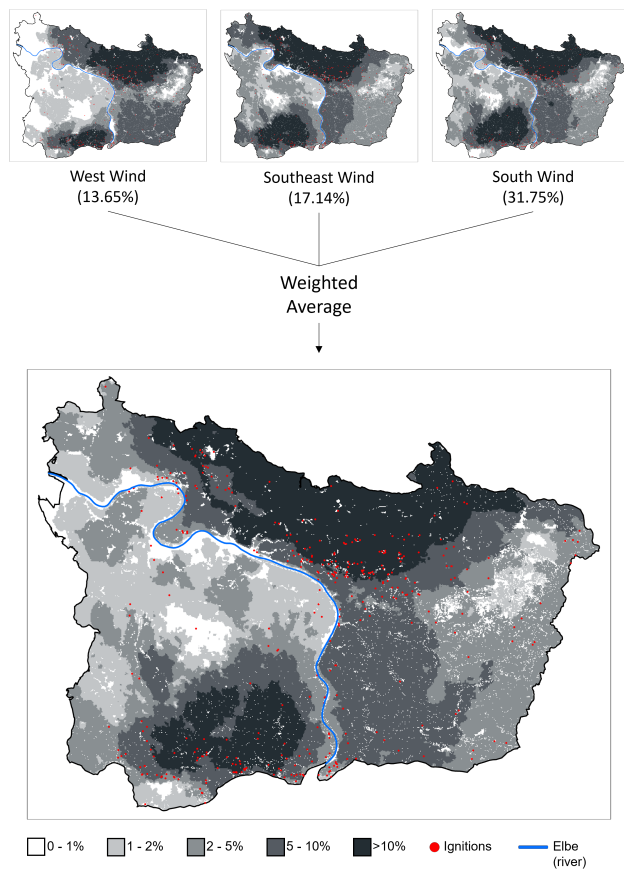
Figure D2. Workflow for derivation of burn probability raster for scenario WBI = 5 and duration = 3 days
