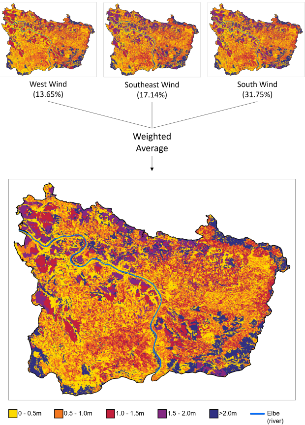
Figure D1. Workflow for derivation of flame length raster for scenario WBI = 5 and duration = 3 days
