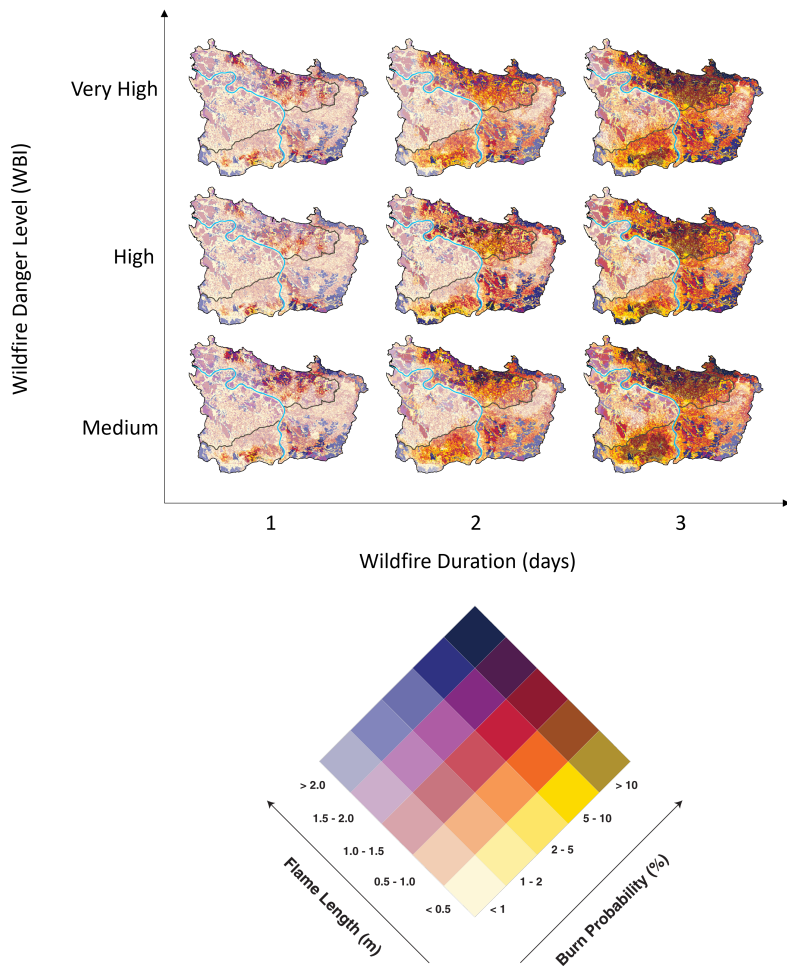
Figure 4: The nine wildfire hazard rasters for three different levels of forest fire danger (WBI) and three different fire durations. National borders and the River Elbe are also overimposed. Each scenario simultaneously represents the flame length (FL) and burn probability (BP) classes. The legend's colours were created using the HSB (Hue Saturation Brightness) Colour Model. Hue
