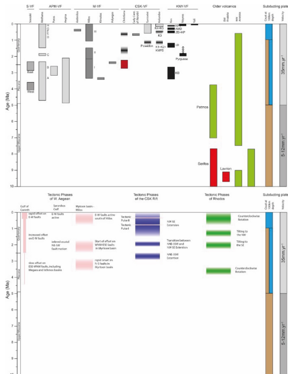
425 Figure 7: (A) Age distribution for the different volcanic fields of the South Aegean Volcanic Arc and older volcanics from Western 430 Anatolia and the Aegean Sea. Abbreviations S-VF, Sousaki volcanic field; APM-VF, Aegina-Poros-Methana volcanic field, M-VF, 435 Milos Volcanic field, CSK-VF, Christiania-Santorini-Kolombo volcanic field, KNY-VF, Kos-Nisyros-Yali volcanic field. The east- west Sousaki volcanic field data are from Vougioukalakis et al., 2019 and references therein). The different phases for Methana are labelled A-H (Pe-Piper and Piper, 2013). The volcanic periods of Milos are labelled I, II and III (Zhou et al., 2021). The shaded fields are ages derived from seismic profiles and sedimentation rates for Christiania volcanics and the Poseidon centre (Preine et al., 2021). The new ages for subareal Christiania volcanics from this study are indicated with a red box. Label KMFD, K1-K5 are volcanic phases of Kolombo (Hubscher et al., 2015). The volcanic deposits of Kos are: KP1=Kos Plateau Tuf (Smith et al., 1996) AMD = Agios Mamas dome, ZD=Zini dome, KP=Kefalos series pyroclastics, KD=Kefalos dacite (Bachmann et al., 2010 and ages reported therein). The age for Pyrgussa is from Piper et al. (2019). Arrows indicate that due to excess ^{40}\text{Ar} this is the maximum age. Nisyros ages are from Poppa et al. (2020). The ages from Patmos are from Boehm et al. (2023). Data for Serifos, Lavrion, NW and SW Anatolia are from Schaarschmidt et al. (2020) and Aklunkaynak et al. (2012) and sources in these publications. Nature of the subducted crust and the subduction velocity are after Schaarschmidt et al. (2021). (B) Tectonic events in Aegean Sea, based on compilations by Pe-Piper and Piper (2013) for the western Aegean and on Preine et al. (2022) for the Rhodos region.
