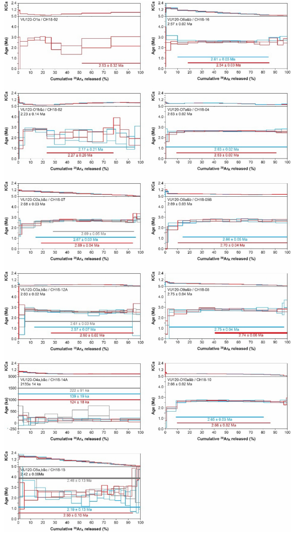
Figure 4: Cumulative ^{39}\text{Ar}_K released versus Age and K/Ca ratio for Christi samples. See text for discussion.
