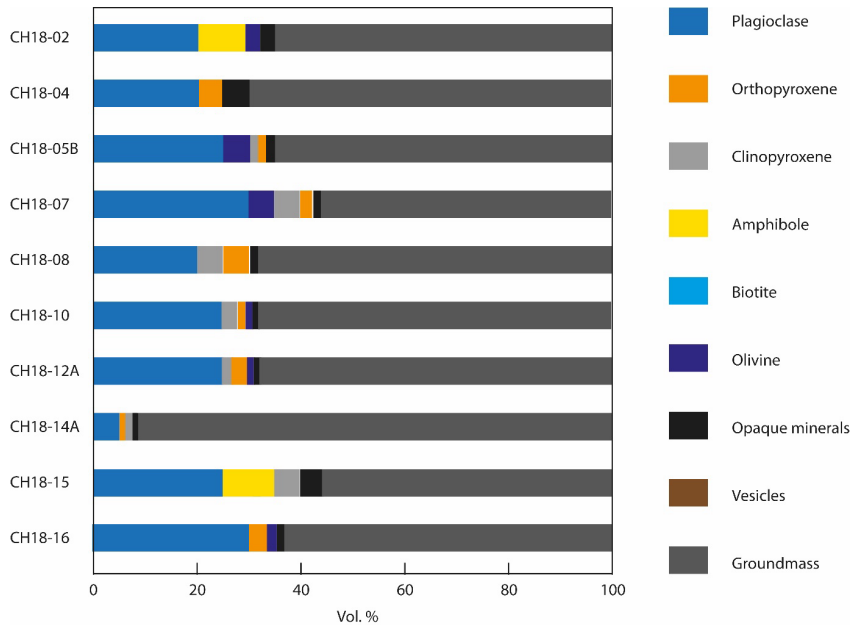
245 Figure 3: Modal composition (phenocrysts/groundmass/vesicles) of the studied samples from Christiani island.
