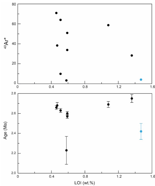
350 Figure 6: LOI versus (A) ^{40}\text{Ar}^* and (B) Age. Three samples that did not provide a meaningful age are also included (see Table 1). Black symbols are samples without amphibole, sample CH18-15 (blue symbol) does contain amphibole. Sample CH18-14A is omitted from (B) due to its very young age 0.133Ma. Error bars are 2\sigma . See text for discussion.
