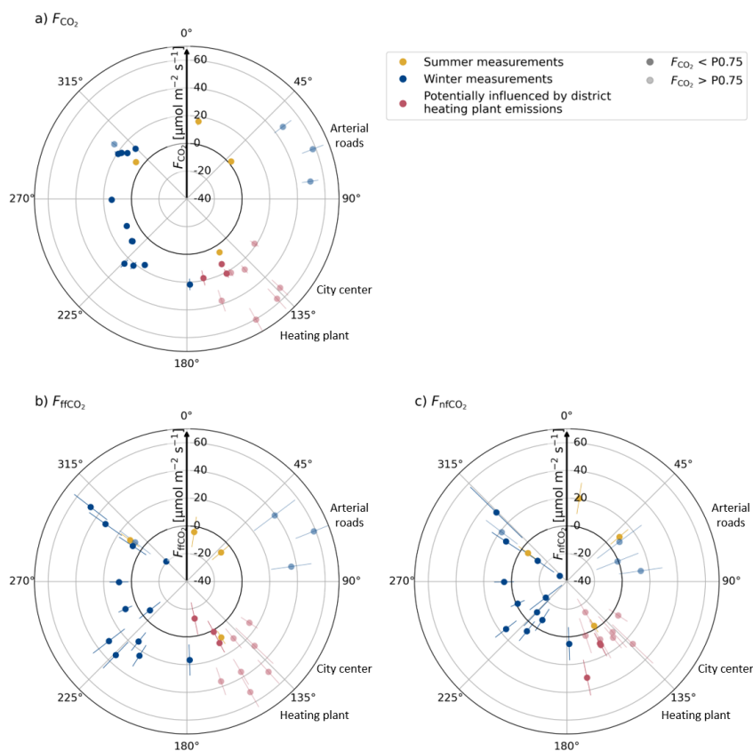
Figure 6. Net \text{CO}_2 fluxes (a), \text{ffCO}_2 fluxes (b), and \text{nfcCO}_2 fluxes (c) with respect to the mean wind directions during the measurement intervals in Zurich with well-mixed conditions. The error bars represent the respective flux uncertainties. Measurements potentially influenced by emissions from a district heating plant to the southeast are indicated in red. P_{0.75} denotes the 75th percentile of the continuous EC \text{CO}_2 fluxes at the respective hour of the day of the respective season. Indicated are also the directions of the arterial roads, the city center, and the district heating plant.
