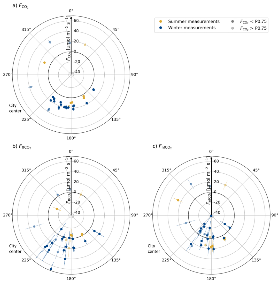
Figure G1. Net \text{CO}_2 fluxes (a), ff \text{CO}_2 fluxes (b), and nf \text{CO}_2 fluxes (c) with respect to the mean wind directions during the measurement intervals in Paris with well-mixed conditions. The error bars represent the respective flux uncertainties. P0.75 denotes the 75th percentile of the continuous EC \text{CO}_2 fluxes at the respective hour of the day. Indicated is also the direction of the city center.
