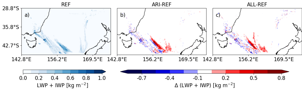
Figure 13. LWP+IWP for the a) REF, difference in LWP+IWP for b) ARI-REF, and c) ALL-REF on December 31 at 14:30 AEDT.
