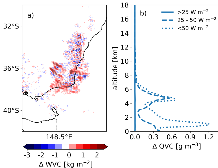
Figure 4. Impact of fire induced moisture release at 14:30 AEDT on December 30. a) difference in WVC MOIST-REF. b) mean vertical profile of QVC difference within three different fire areas (MOIST-REF). Solid: 0 < \text{FRP} > 25 \text{ W m}^{-2} , dashed: 25 \text{ W m}^{-2} < \text{FRP} and \text{FRP} > 50 \text{ W m}^{-2} , dotted: \text{FRP} < 50 \text{ W m}^{-2} .
