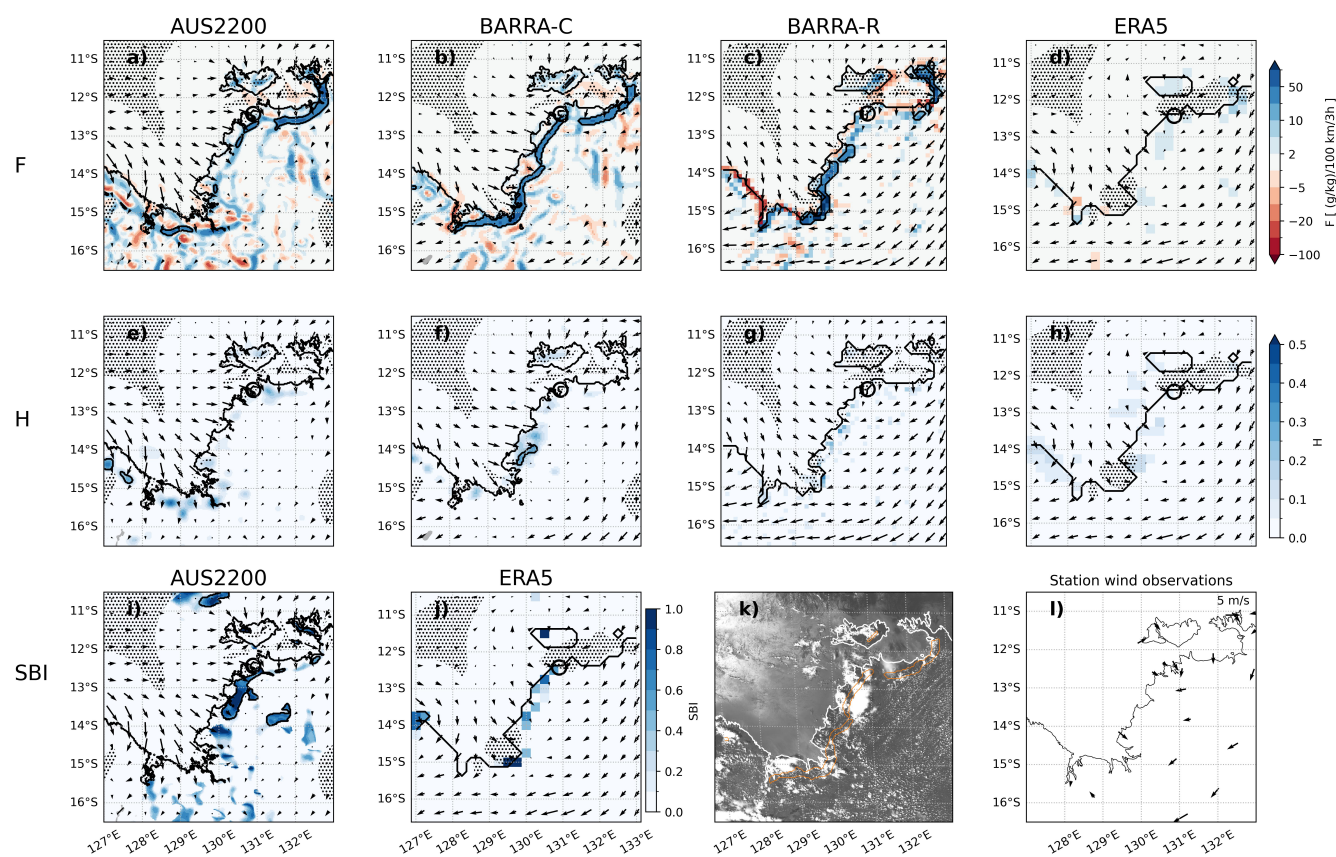
Figure 5. As in Figure 3 but for 2016-01-10 05:00 UTC (14:30 local time) for a case over the Darwin region.
