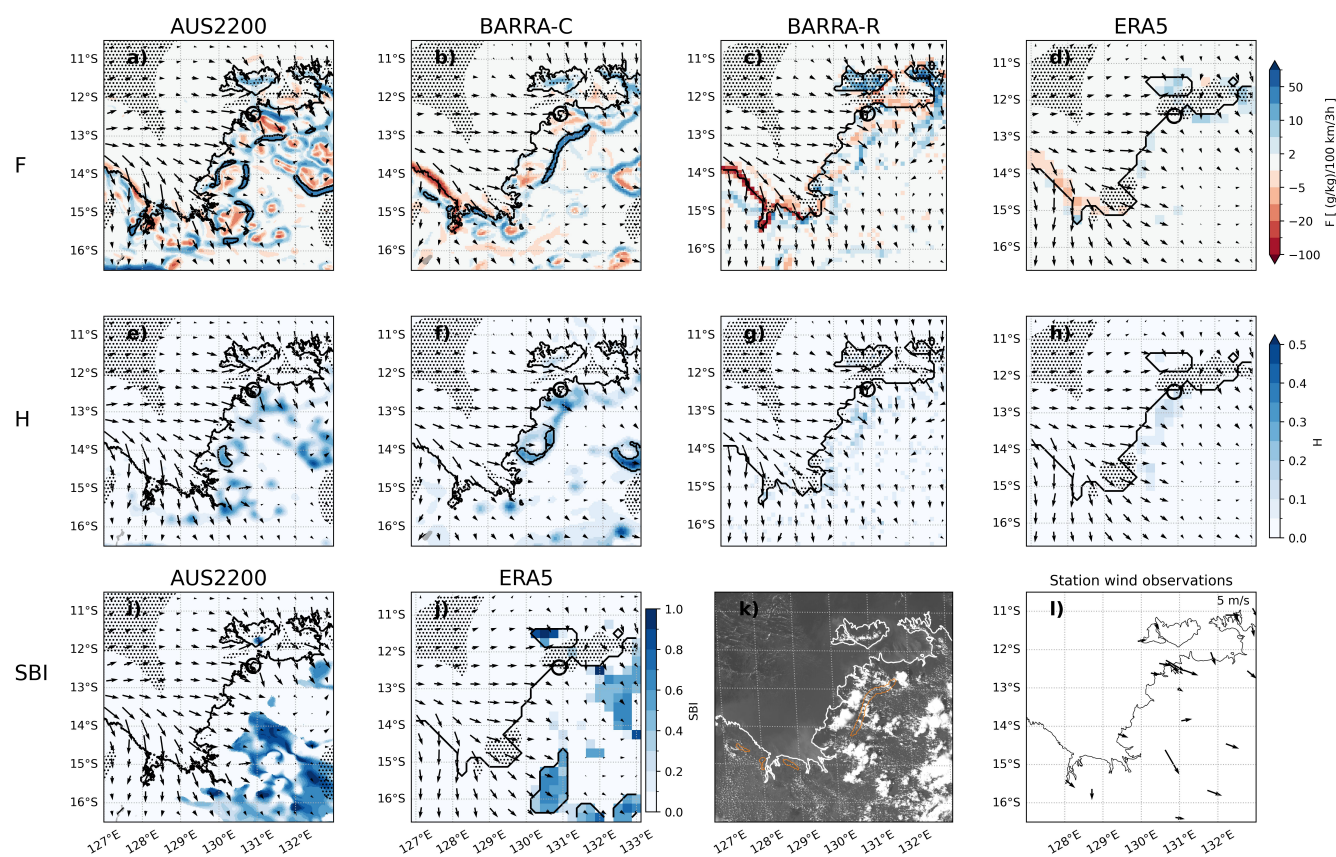
Figure 6. As in Figure 3 but for 2016-01-12 06:00 UTC (15:30 local time) for a case over the Darwin region.
