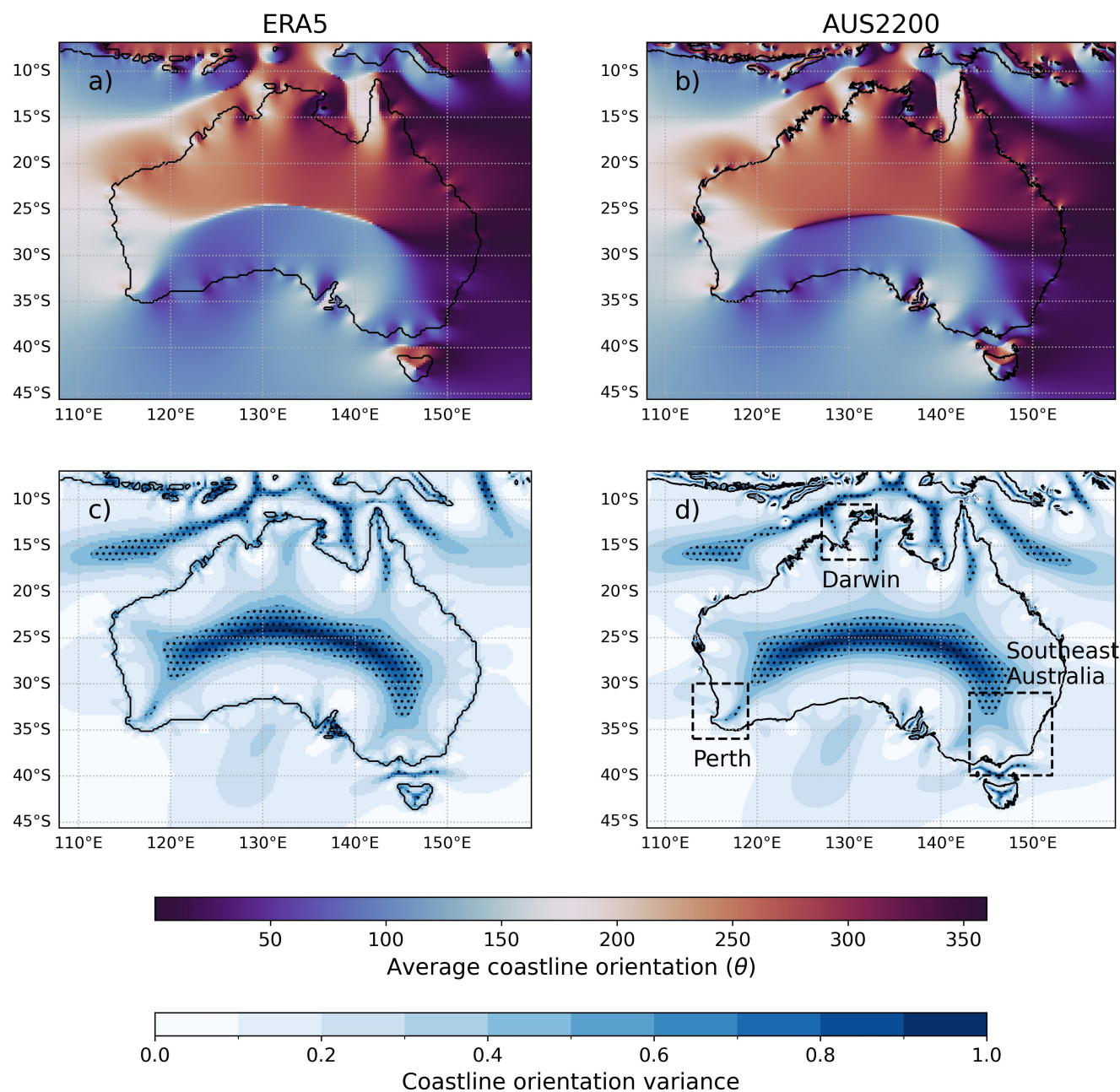
Figure 2. The weighted average angle between each point and the coastline, representing average orientation orientation ( \theta ), shown separately for (a) ERA5 and (b) AUS2200. Also shown is the coastline orientation variance at each grid point, for (c) ERA5 and (d) AUS2200. Variance values above 0.5 are highlighted here using stippling, as regions where it may not be appropriate to define a coastline orientation angle. In each panel, the coastline is shown as a contour between land and ocean in the land sea mask. In panel (d), the location of the case study domains (Section 4) are indicated with black dashed boxes.
