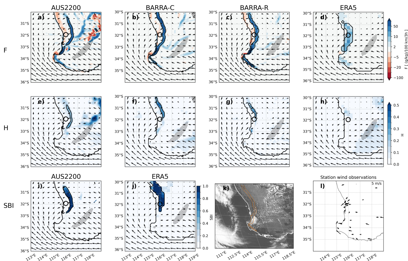
Figure 3. Sea breeze diagnostics for 2016-01-06 08:00 UTC (16:00 local time) for a Perth sea breeze case, including (a–d) F , (e–h) H , and (i and j) SBI , calculated from (a, e, and i) AUS2200, (b and f) BARRA-C, (c and g) BARRA-R, and (d, h, and j) ERA5. Model 10 m wind vectors are shown in each panel, and compared with (l) station wind observations. Sea breeze objects are shown with a black contour. The corresponding Himawari visible satellite image is shown in (k), with the BARRA-C F sea breeze mask indicated with an orange contour for comparison. In each panel, the model land-sea mask is also contoured with a black line, representing the coastline. Stippling indicates regions where there is no dominant onshore direction (see Section 3.1).
