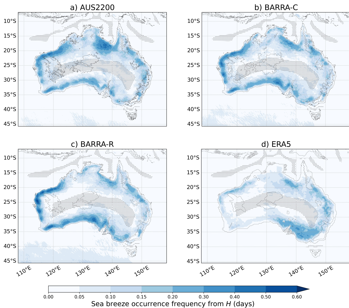
Figure 11. As in Figure 9 but for H
