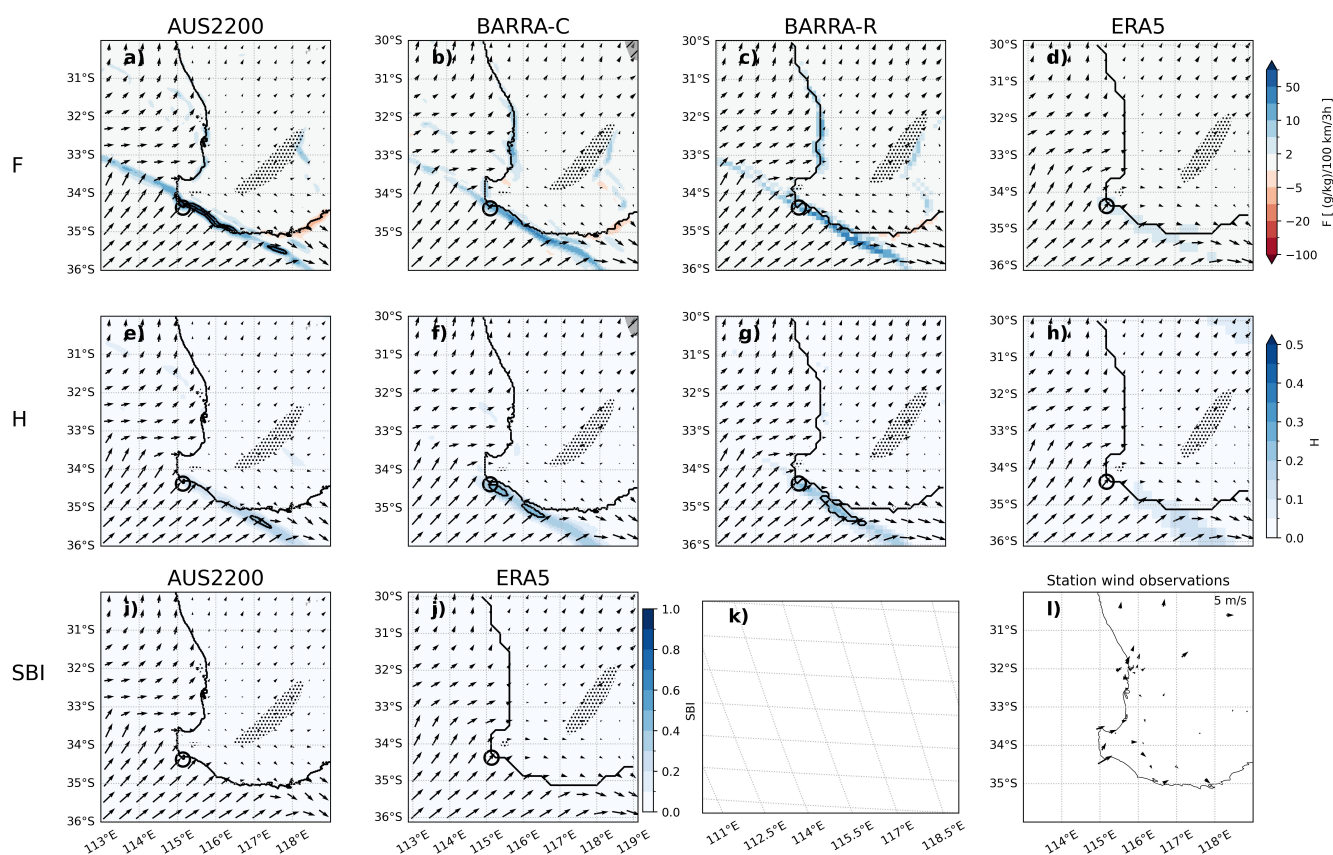
Figure 4. As in Figure 3 but for 2016-01-11 20:00 UTC (04:00 local time). There is no visible satellite imagery available for this case.
