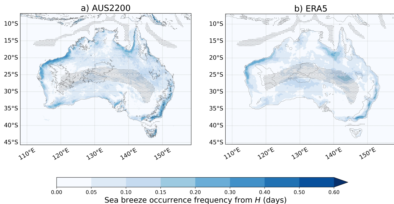
Figure 10. As in Figure 9 but for SBI
