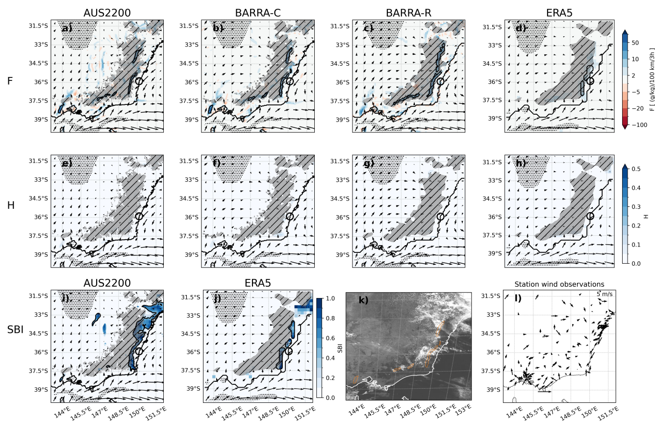
Figure 7. As in Figure 3 but for 2016-01-09 04:00 UTC (approximately 14:00 local time) for a sea breeze event over the south-east of Australia. Shaded hatched regions indicate model topography that exceeds 500 m.
