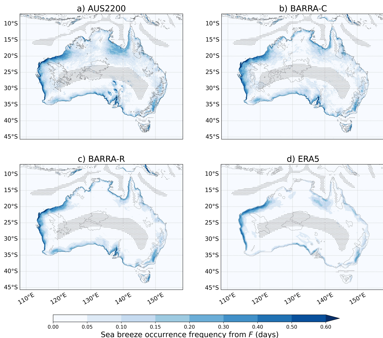
Figure 9. The fraction of days with a sea breeze object from 00:00 to 23:00 UTC at each pixel, based on the F diagnostic over the entire 6-month study period. Shown separately for each model dataset. Regions exceeding 500 m above sea level are indicated with a contour, and stippling indicates regions without a dominant coastline direction (see Section 3.1). Note that the color scale is not evenly spaced, to capture the spatial variability and small occurrence frequencies.
