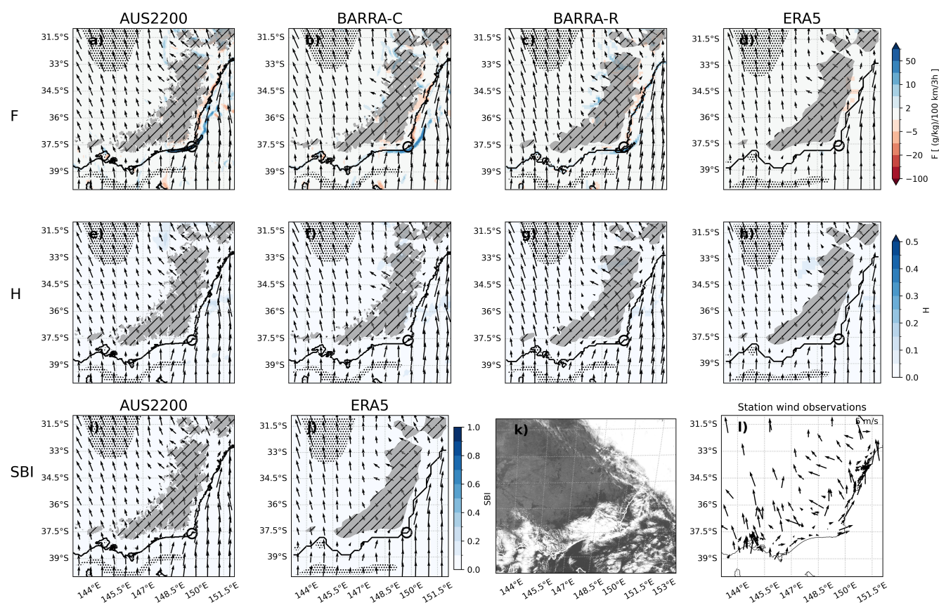
Figure 8. As in Figure 3 but for 2016-01-14 23:00 UTC (approximately 09:00 local time) for a sea breeze event over the south-east of Australia. Shaded hatched regions indicate model topography that exceeds 500 m.
