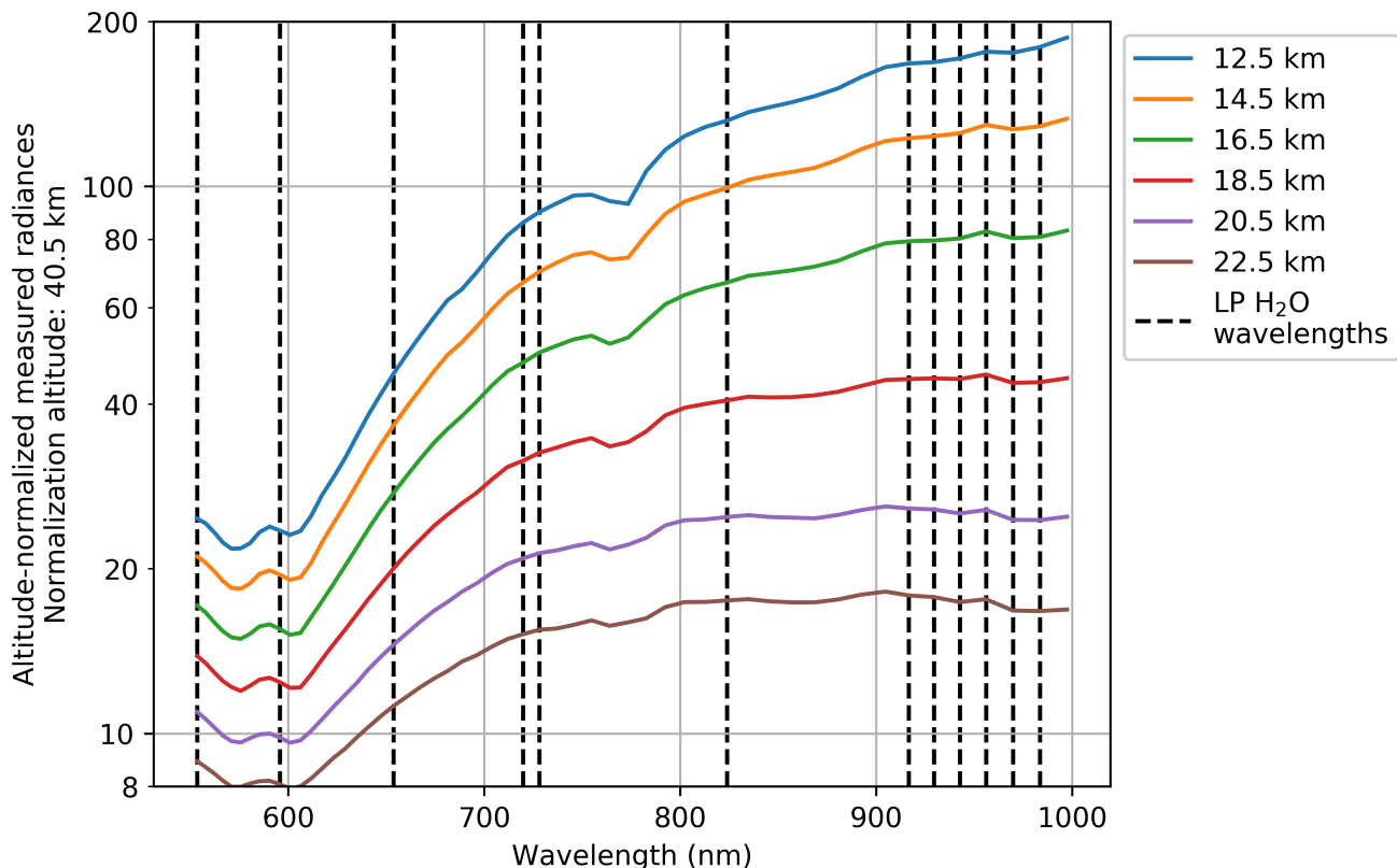
Figure A4. Like Figure A2, but for the event simulated in Figure A3. Unlike in Figure A2, there are no obvious spectral features attributable to H 2 O in the 930–970 nm spectral band.
