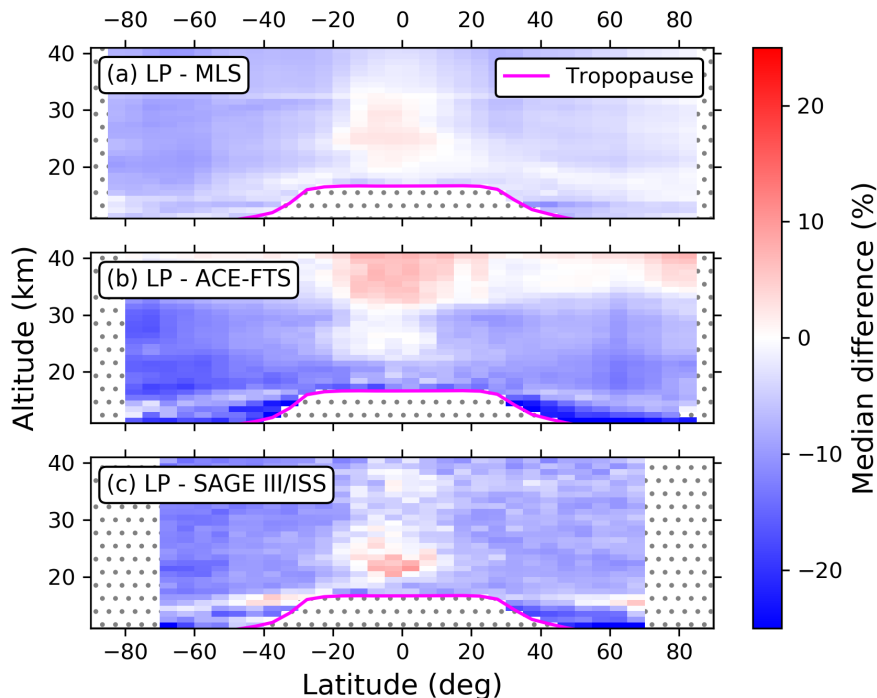
Figure 14. Like Figure 5, but for NOAA-21 OMPS LP.
