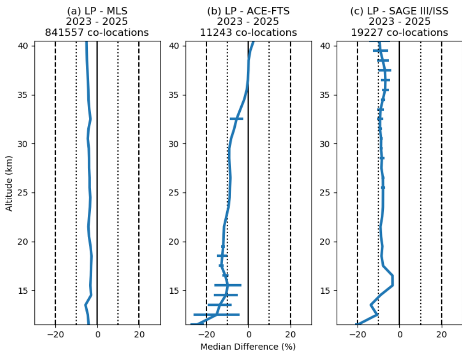
Figure 13. Like Figure 4, but for NOAA-21 OMPS LP.
