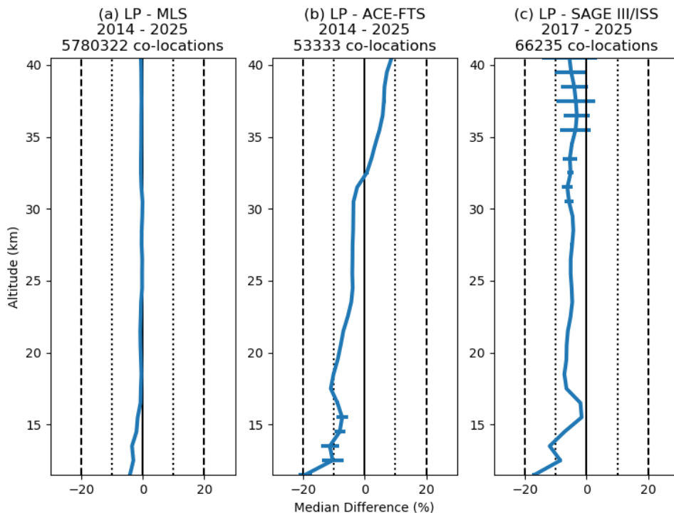
Figure 4. Summary of global median percent differences between the LP stratospheric H 2 O profiles and co-located (a) MLS, (b) ACE-FTS, and (c) SAGE III/ISS profiles. Horizontal uncertainty bars indicate the standard error of the median.
