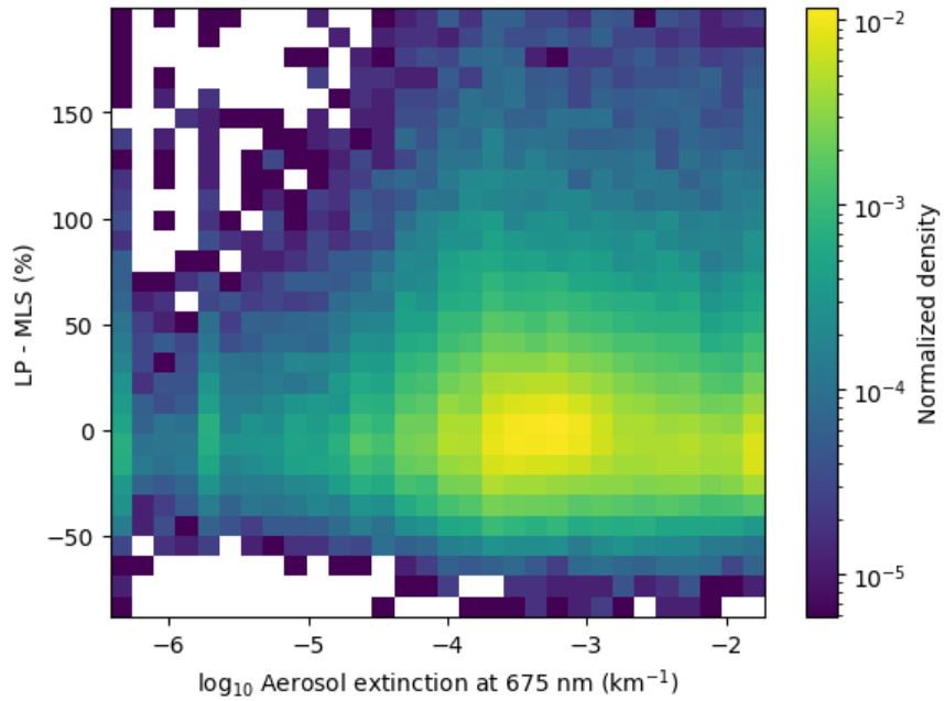
Figure D1. Histogram of the LP-MLS percent differences vs. OMPS LP aerosol extinction at 675 nm at 11.5 km. Errors are clustered around 0%, indicating aerosols do not significantly impact model performance.
