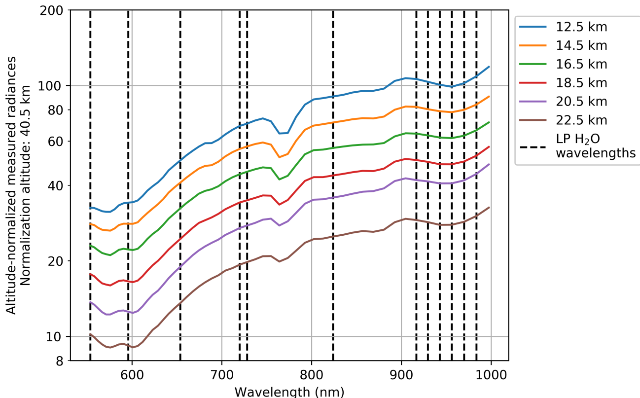
Figure A2. Altitude-normalized radiances measured by OMPS LP for the event modeled in Figure A1. At these altitudes, including in the lower stratosphere, a small decrease in radiances is observed around 930–970 nm, which we believe is attributed to water vapor absorption. However, the measured radiances do not show reduction around 720 and 824 nm as predicted by the RTM simulations, possibly due to the RTM’s simplifying assumptions.
