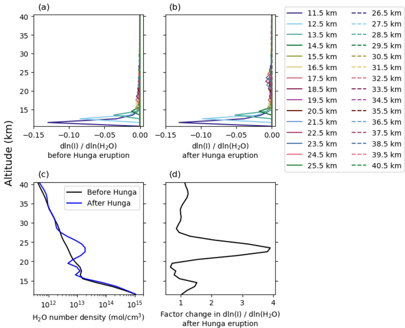
Figure 1. Example of OMPS LP’s sensitivity to H_2O at 945 nm in the tropics. Panels (a) and (b) show the Jacobians for selected MLS H_2O profiles from before and after the Hunga eruption, respectively. Panel (c) shows the selected water vapor profiles, which show an enhancement in water vapor around 24 km attributable to the Hunga eruption. Panel (d) shows the ratio of (b) to (a). The increased water vapor concentration between 21–27 km due to Hunga results in LP’s sensitivity increasing by up to 4\times in this altitude range.
