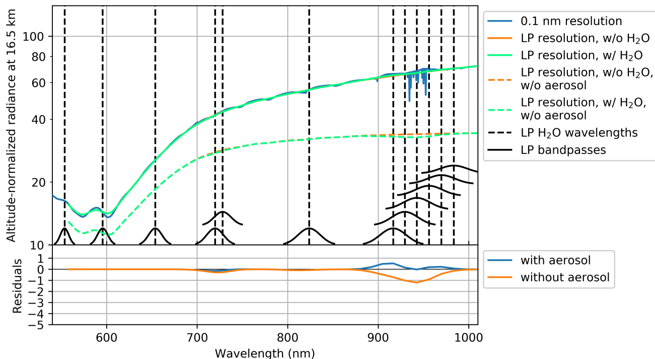
Figure A3. Like Figure A1, but for a measurement at 61.6^\circ N latitude, 87.0^\circ E longitude, solar zenith angle of 46.2^\circ , and a single scattering angle of 49.5^\circ . Simulations without aerosol are shown as dashed orange and green lines. Unlike in Figure A1, the lower panel here shows almost no differences between the simulations with and without \text{H}_2\text{O} in 930 – 970 nm spectral range, and even indicate a small increase in radiances simulated with \text{H}_2\text{O} compared with the simulation without \text{H}_2\text{O} . When omitting aerosol, radiances decrease due to \text{H}_2\text{O} absorption, confirming the increase in radiances for these viewing conditions is due to aerosol.
