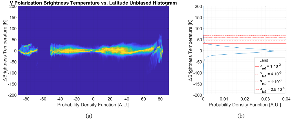
Figure 3. (a) Unbiased 2-D histogram of the brightness temperature at 6.9 GHz V polarization in AMSR2 as function of the latitude. The histogram is normalized in bins of 0.25^\circ latitude. (b) Integrated 1-D histogram for the unbiased 2-D histogram in (a). The figure has been rotated and vertically aligned to match the integration of (a) along the latitudinal axis aligning their peaks.
