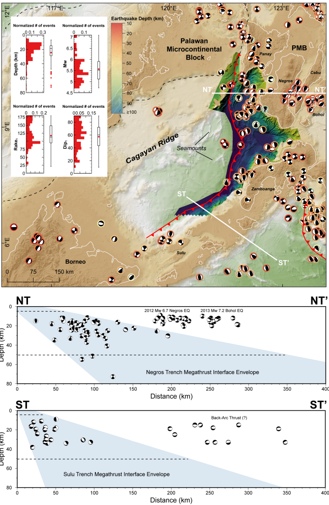
Figure 2. Reverse-oblique focal mechanism solutions (1977–2023) of earthquakes along the Negros–Sulu subduction zone collated by the International Seismological Centre (ISC) (Bondár et al., 2015; Di Giacomo et al., 2015, 2018; Storchak et al., 2013, 2015). Earthquakes in the cross-sectional profiles (NT–NT' and ST–ST') are within 80 km depth and 200 km distance from each side of the
