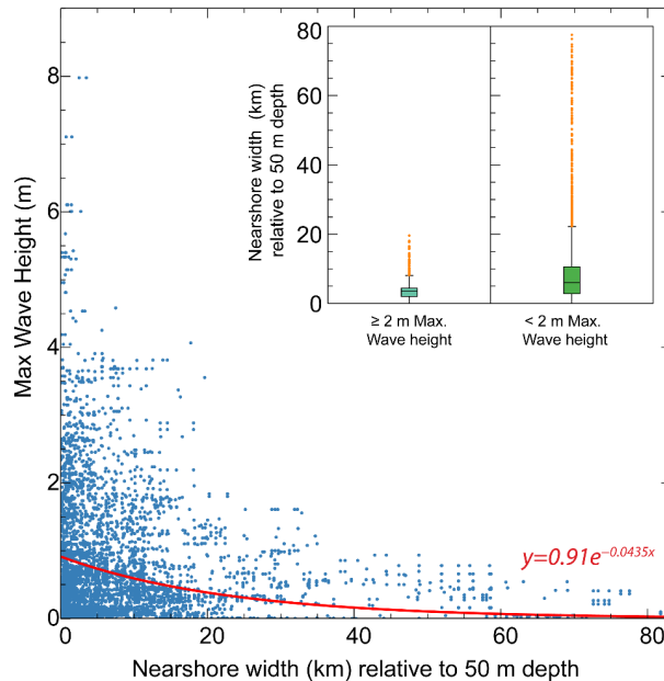
Figure 13. Maximum tsunami wave height from 6,879 sampling points across the coastal regions in central and southern Philippines and the corresponding nearshore width (km) relative to 50 m depth. Boxplots show the interquartile range (1.5IQR) of nearshore width between coastlines with \geq 2 m and < 2 m maximum tsunami wave height. Orange circles indicate the outliers of the interquartile range.
