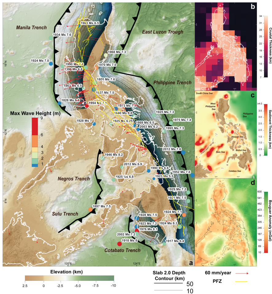
Figure 1. Philippine tectonic setting. (a) Estimated epicenters of positive tsunamigenic earthquakes and the associated eyewitness accounts of maximum wave heights in the affected coastal areas since 1589 (Bautista et al., 2012). The trace of the Philippine Fault Zone (PFZ) was adapted from PHIVOLCS. Depth contours of the Slab 2.0 model from Hayes et al. (2018). Arrows indicate the velocity vectors relative to no-net-rotation reference frame from inland GPS networks (Kreemer et al., 2014). Bathymetry and topography data from the 2024 General Bathymetric Chart of the Oceans (GEBCO) (GEBCO Compilation Group, 2024). (b) Crustal
