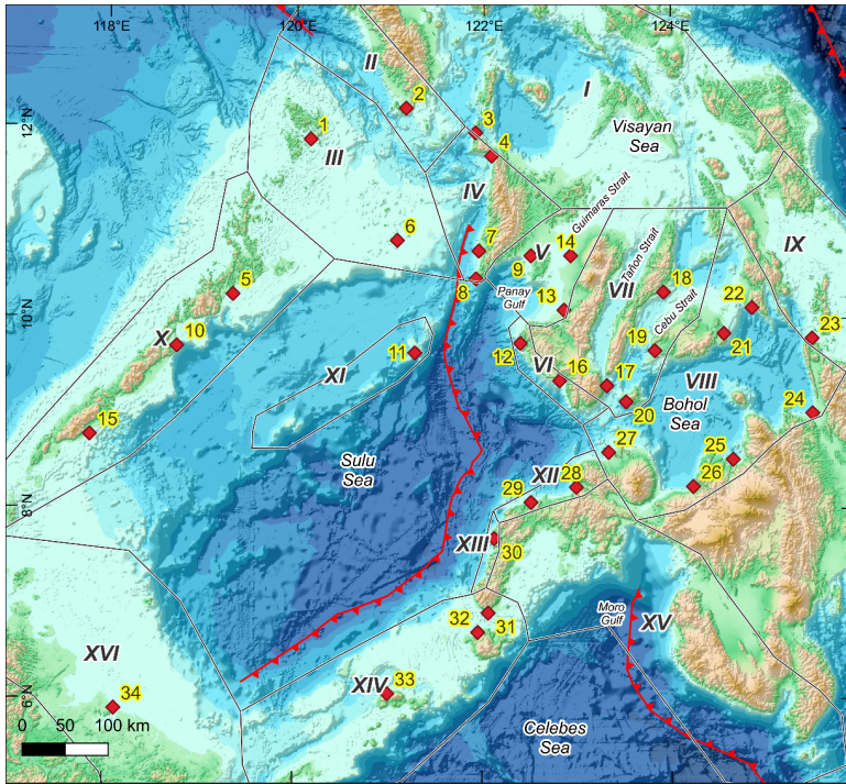
Figure 4. The 16 coastal regions surrounding the Negros–Sulu subduction zone and the 34 synthetic tide gauge stations (TGS). I, Visayan Sea; II, Mindoro; III, Coron–Cuyo; IV, West Panay; V, Panay Gulf; VI, Sipalay–Bayawan; VII, Tañon–Cebu Strait; VIII, Bohol Sea; IX, Leyte Gulf; X, Palawan; XI, Cagayancillo; XII, Sindangan–Labason; XIII, Siocon–Sibuco; XIV, Basilan–Sulu; XV, Moro Gulf; XVI, northeast Borneo. Basemap from GEBCO Compilation Group (2024).
