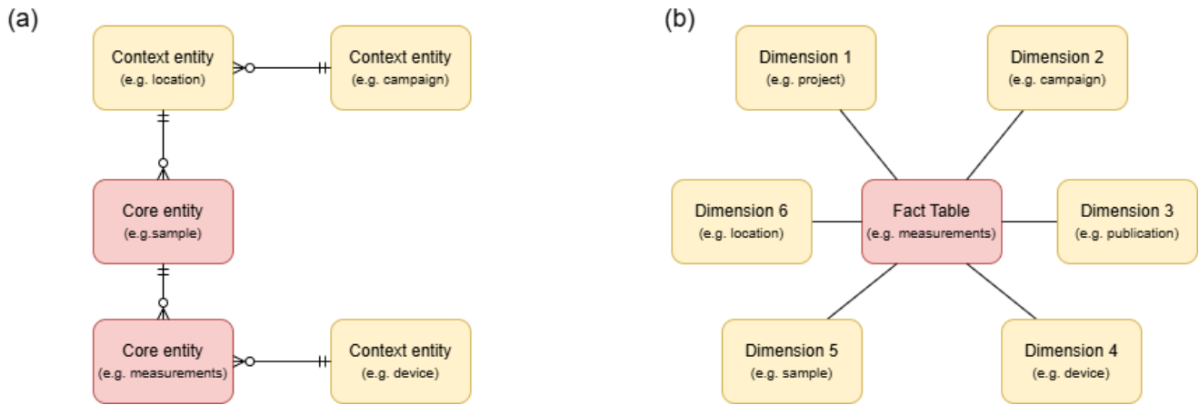
Figure 2. A simplified relational schema (a) as used in the a relational OLTP database model and a star schema (b) as used a star schema in the denormalised OLAP database direct comparison. The normalised relational schema (a) organises data across logically linked tables to minimise redundancy and ensure data integrity. Here To clarify their function within this diagram, we use the relationships are more granular: a sample is linked to a location, which is then linked to a campaign illustrative terms Core entities for the central objects of research and , finally, to a project Context entities for the descriptive metadata. Although this structure makes analytical queries more complex, it is ideal for transactional operations and ensures consistency in operational workflows. By contrast, the central fact table in the star schema (b) stores quantitative measurements and is directly linked to dimension tables that contain descriptive information on projects, locations, campaigns, and different data types. This design enables efficient analytical queries by denormalising the data structure, which improves query improving performance for aggregations and slicing operations. In contrast, the normalised relational schema represents a more complex perspective on the relationships between entity types that organises data in logically linked tables to avoid redundancy.
