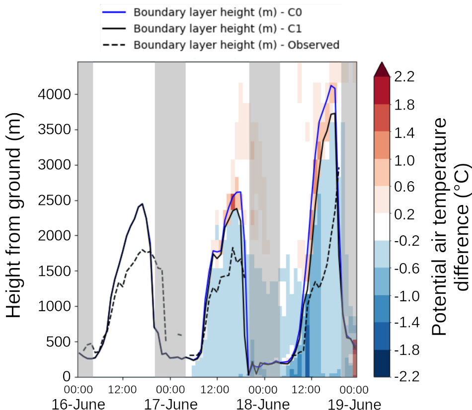
Figure 9. Comparaison of time-series of boundary layer height simulated (C0 and C1) and observed at the Jussieu station, and vertical variation of the potential air temperature difference between C1 and C0 at the the same location.
