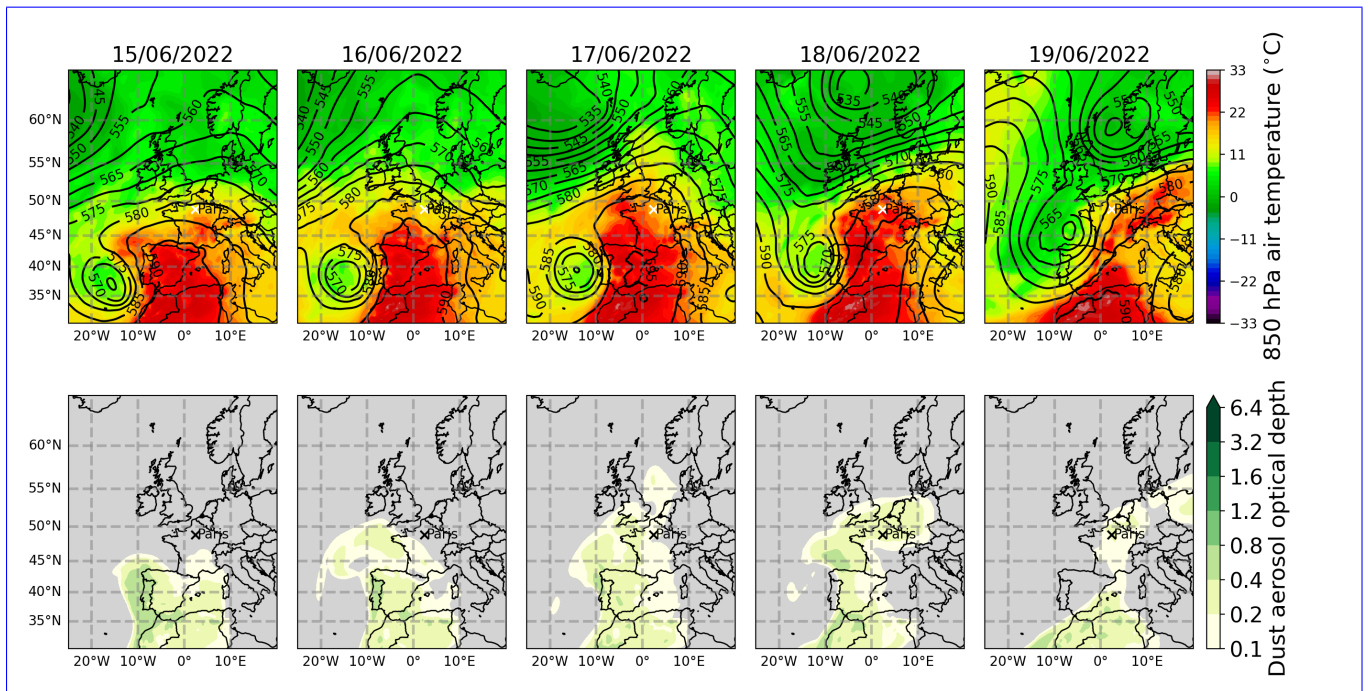
Figure 1. Synoptic-Top panel: synoptic overview at 12 UTC (14 LT in Paris ) from 15 to 19 June 2022 based on ERA5 reanalysis (Hersbach et al., 2023). The colors and the contours represent the air temperature at 850 hPa and the 500 hPa geopotential height, respectively.
