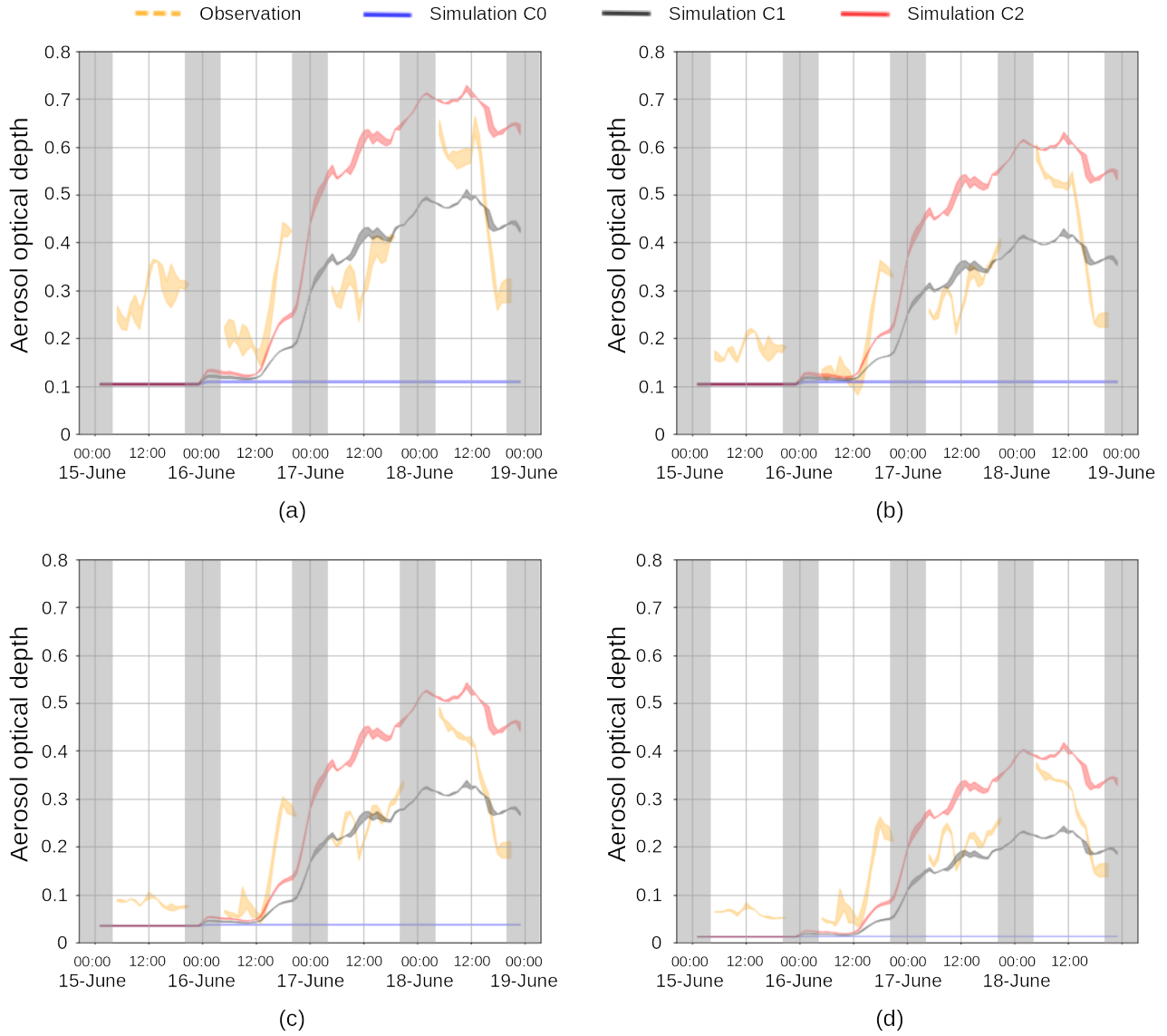
Figure 4. Time-series of aerosol optical depth observed (and simulated) at the Jussieu and Palaiseau station-stations (a) at 340 nm (250-440 nm), (b) at 500 nm (440-690 nm), at 1020 nm (690-1190 nm) and (d) at 1640 nm (1190, 2380 nm). The color patches represent the AOD value difference between the two locations: a larger patch thus denotes higher spatial variability. Note that this is not possible to observe AOD during night-time (20 UTC to 04 UTC).
