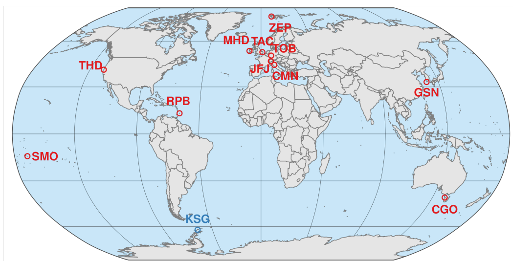
Figure 1. Location of the AGAGE (Advanced Global Atmospheric Gases Experiment) stations (in red) with publicly available measurements of HFO-1234yf ( \text{CF}_3\text{CF}=\text{CH}_2 ), HFO-1234ze(E) ( trans - \text{CF}_3\text{CH}=\text{CHF} ), and HCFO-1233zd(E) ( trans - \text{CF}_3\text{CH}=\text{CHCl} ): Zeppelin, Spitsbergen (ZEP), Mace Head, Ireland (MHD), Tacolneston, UK (TAC), Taunus, Germany (TOB), Jungfrauoch, Switzerland (JFJ), Monte Cimone, Italy (CMN), Trinidad Head, California, USA (THD), Gosan, South Korea (GSN), Ragged Point, Barbados (RPB), Cape Matatula, American Samoa (SMO), and Kennaook / Cape Grim, Australia (CGO). Flask sample measurements are available from the South Korean Antarctic station King Sejong (in blue).
