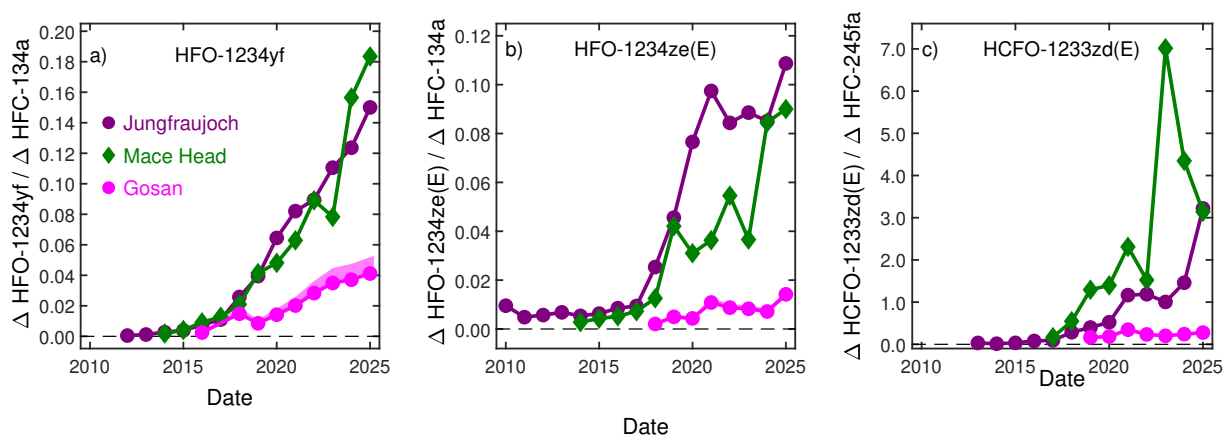
Figure 3. Ratios of pollution magnitudes (above baseline, \Delta ) of HFO-1234yf (a) and HFO-1234ze(E) (b) to HFC-134a and of HCFO-1233zd(E) to HFC-245fa (c) at Jungfrauoch, Mace Head, and Gosan. Assuming co-located The sources and ignoring decay of the substances during are assumed to be co-located for each site. An approximated estimate for a decay correction is applied to the haloolefins for the Gosan measurements by correcting the yearly means for an average conservative transport -time of four days and the yearly averaged lifetimes (Table S1). This correction is shown as a shaded band and only large enough to be visible for HFO-1234yf. The elevated ratios found at Jungfrauoch and Mace Head compared to Gosan suggest an earlier replacement of HFC-134a and HFC-245fa by the HFOs and HCFO-1233zd(E), respectively, in Europe compared to the source region covered by Gosan.
