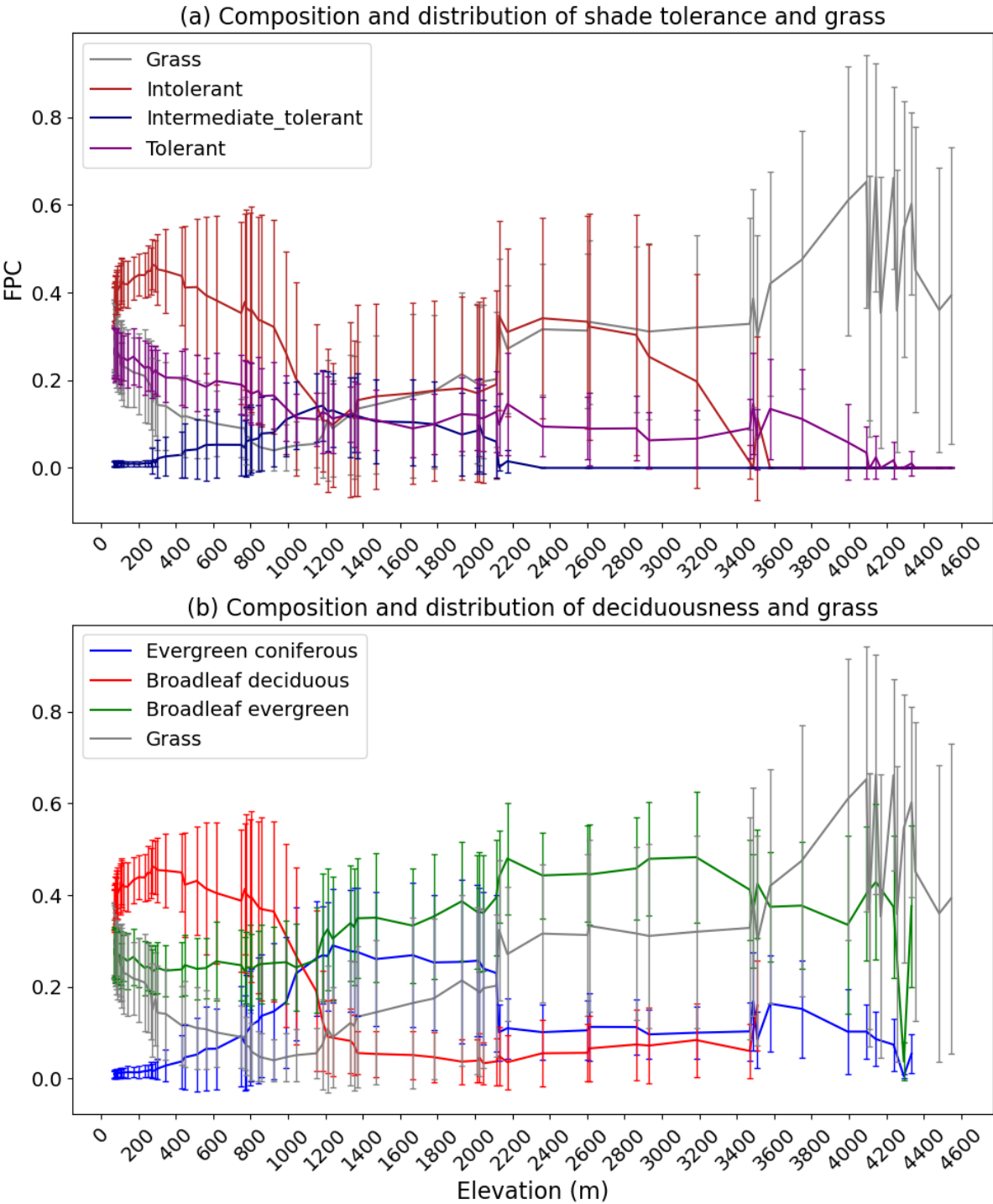
504 505 Figure 10: Distribution and composition of PFTs adaptation strategies (shade tolerance 506 and deciduousness) and grasses (line represents mean and bar represents standard 507 deviation) along the elevation gradient.
