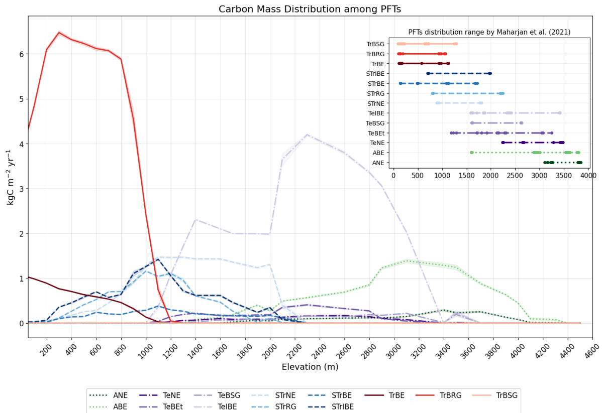
Figure 6: Carbon mass production by PFT along the elevation gradient (the inset figure shows the PFTs' distribution ranges recorded by Maharjan et al. (2021) in the gradient).
