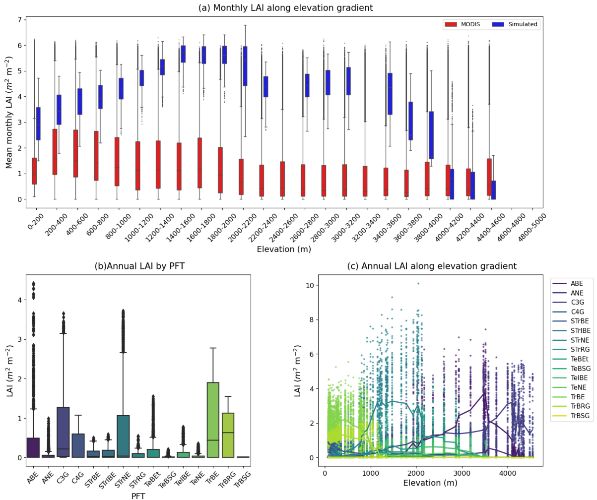
Figure 4: LAI across the elevational gradient. Top panel (a): comparison of monthly simulated LAI (3 km resolution) and MODIS LAI (1 km resolution) plotted against elevation, with points representing mean monthly LAI values at individual grid. Bottom panel: (b) boxplot of simulated annual LAI by PFTs and (c) line plot of total annual LAI (line represents mean LAI for each PFT and dots representing LAI at simulated grids across latitude) across the elevation gradient by PFTs.
