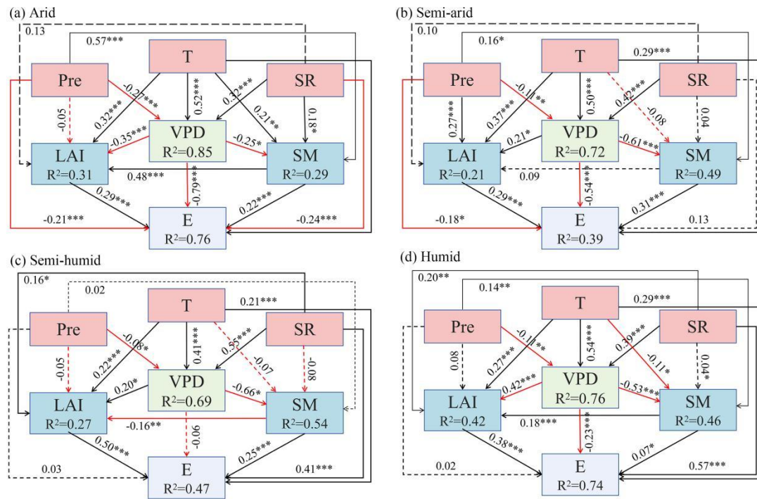
Figure 5. Aridity-zone-specific structural equation models showing the pathways linking VPD and E under different hydroclimatic conditions. Panels show the SEM results for (a) arid, (b) semi-arid, (c) semi-humid, and (d) humid regions. Numbers on arrows indicate standardized path coefficients.
