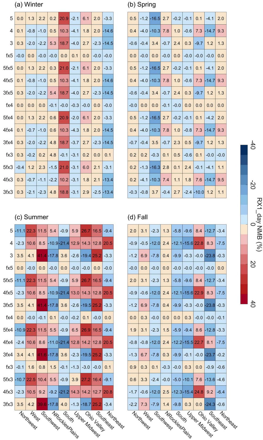
Figure S2: Seasonal and regional NMB of RX1_day (a-d).
