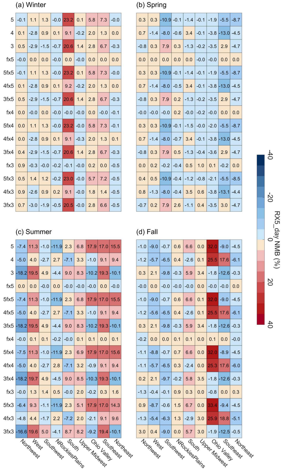
Figure S3: Seasonal and regional NMB of RX5_day (a–d).
