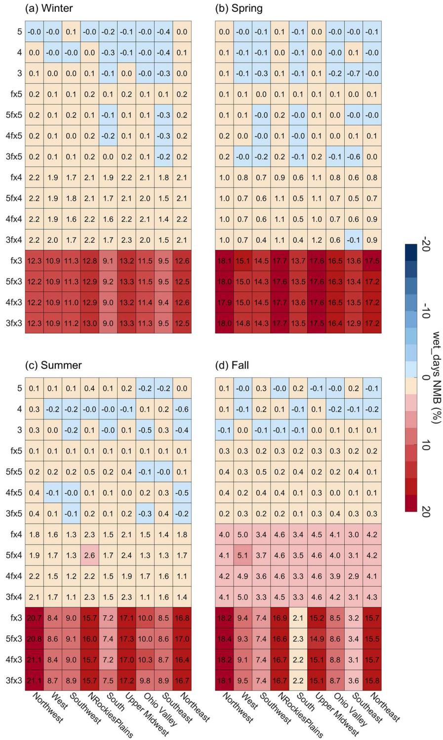
Figure S6: Seasonal and regional NMB of wet_days (a-d).
