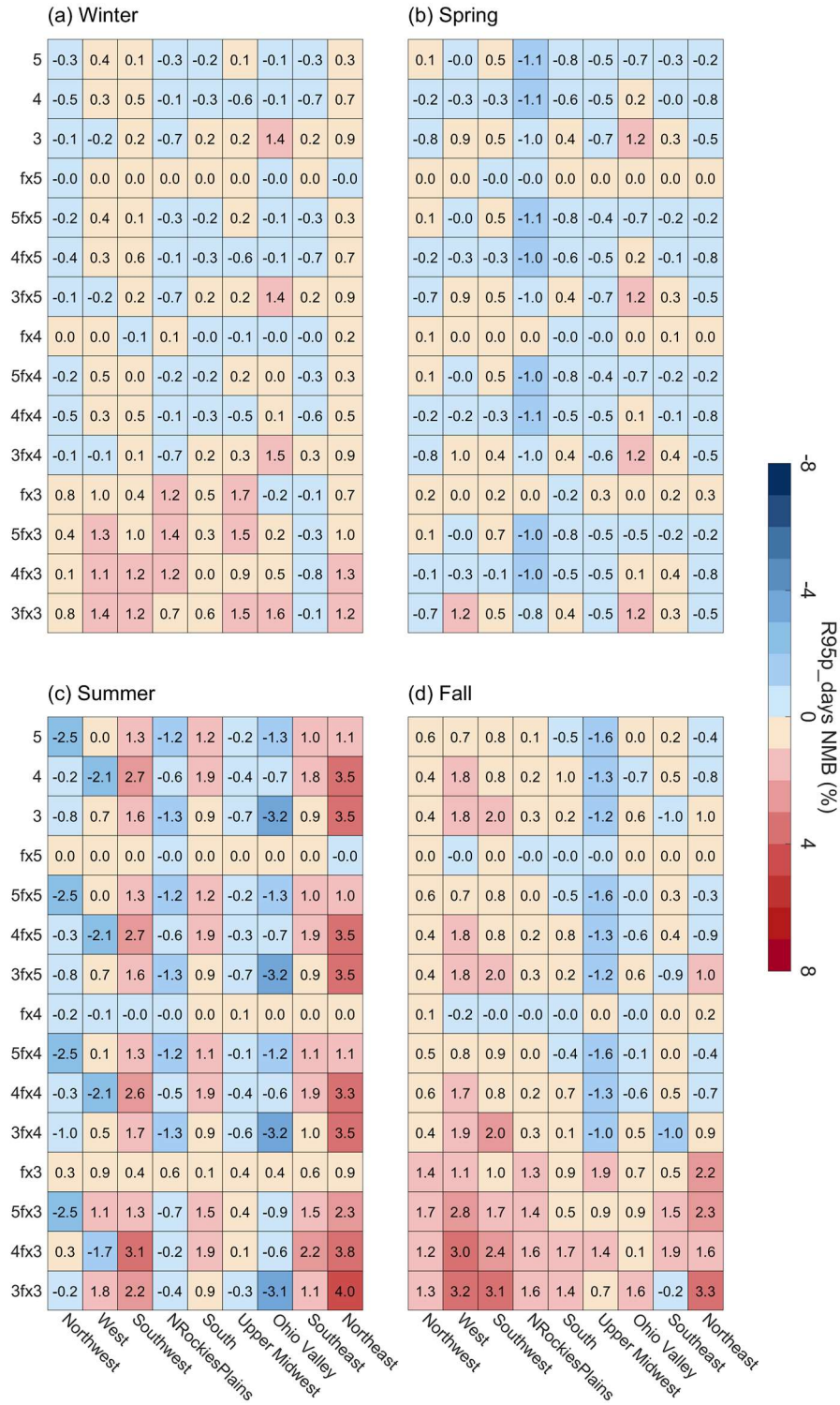
Figure S1: Seasonal and regional NMB of R95p_days (a-d).
