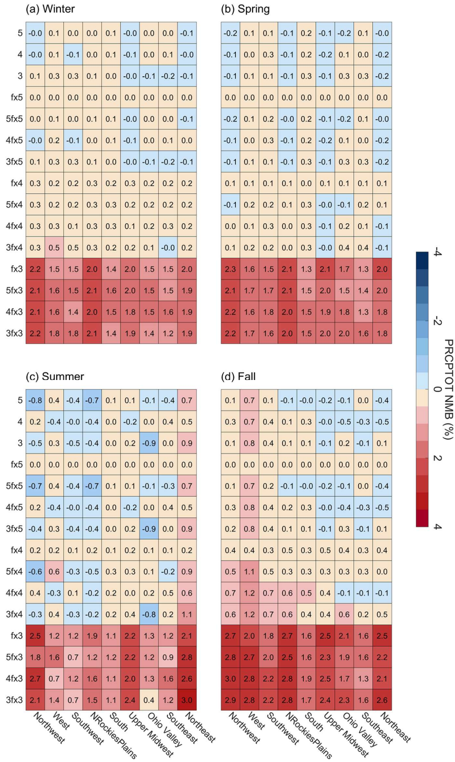
Figure S5: Seasonal and regional NMB of PRCPTOT (a–d).
