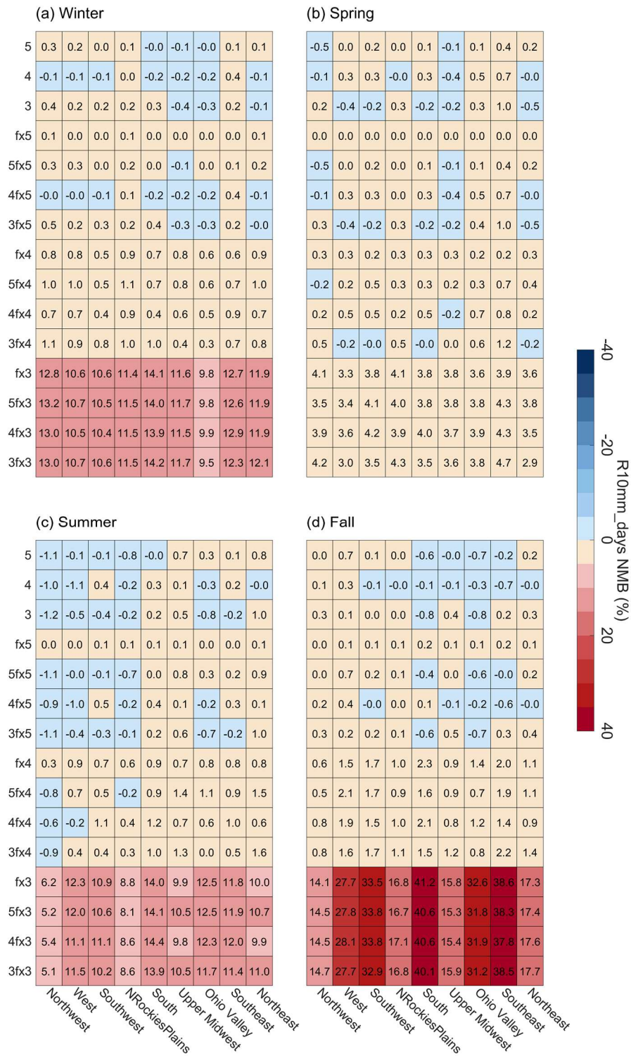
Figure S4: Seasonal and regional NMB of R10mm_days (a-d).
