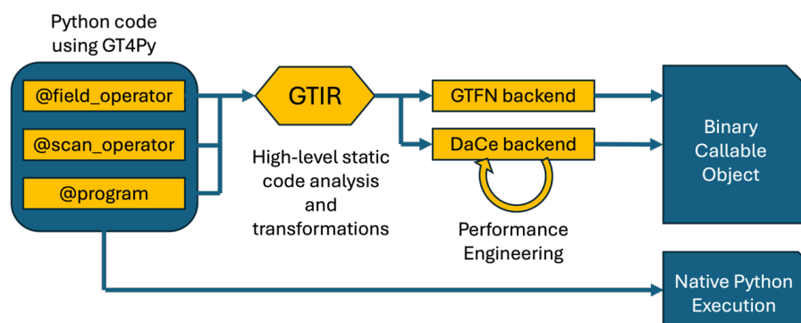
Figure 1 Schematic illustrating the various steps within GT4Py from the user front end to the executable.
