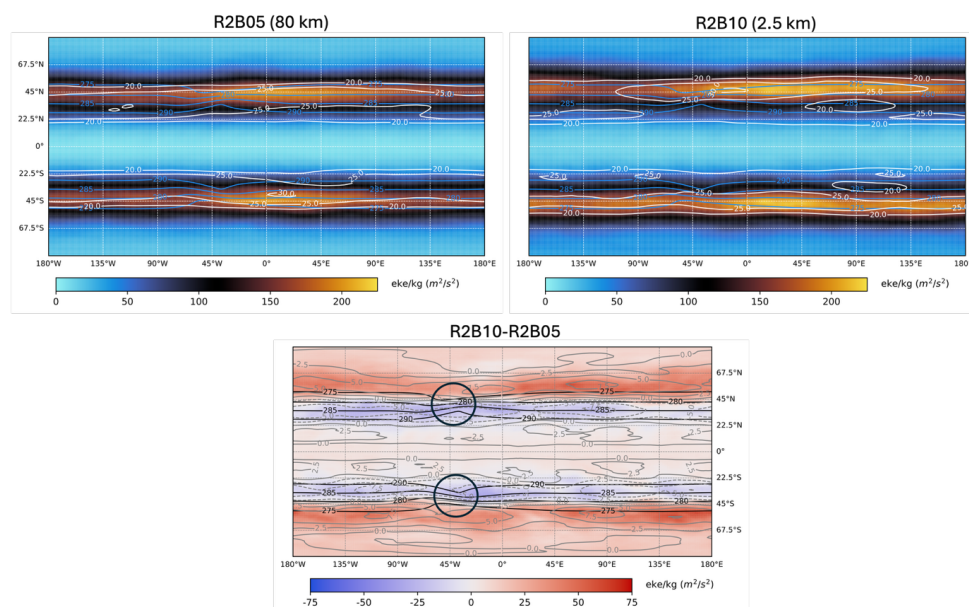
Figure 9: Mean state of the jet in aquaplanet simulations for indicated grids (top) and their difference (bottom). EKE is shaded and the horizontal wind speed is depicted in white (grey) contours (dashed negative) starting at 20 m/s with a spacing of 5 m/s (2.5 m/s) in top (bottom) panel. The blue (black) contours are SST in top (bottom) panels starting at 275 K with a spacing of 5 K. Region around the SST fronts are circled in the bottom panel.
