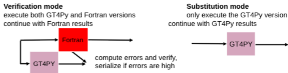
Figure 4: Liskov verification and substitution modes.
