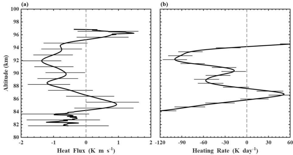
260 Figure 12. The vertical flux of sensible heat. (a) Annual mean sensible heat flux derived from vertical wind and temperature measurements at Hainan, China, and (b) the corresponding heating rates. Error bars are shown as thin lines.
