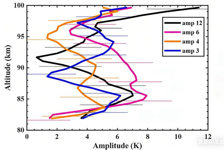
Figure 11. Seasonal harmonic amplitude profiles with the period of 12 (black), 6 (red), 4 (orange), and 3 (blue) months. Error bars are shown as thin lines.
