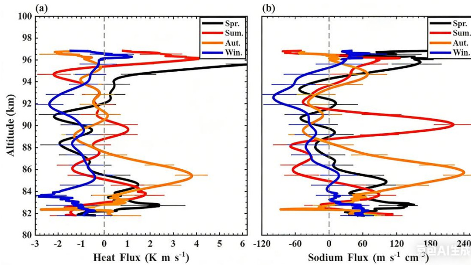
Figure 14. The seasonal profiles of the heat (a) and Na (b) fluxes. Spring (black), summer (red), autumn (orange), winter (blue). Error bars are shown as thin lines.
